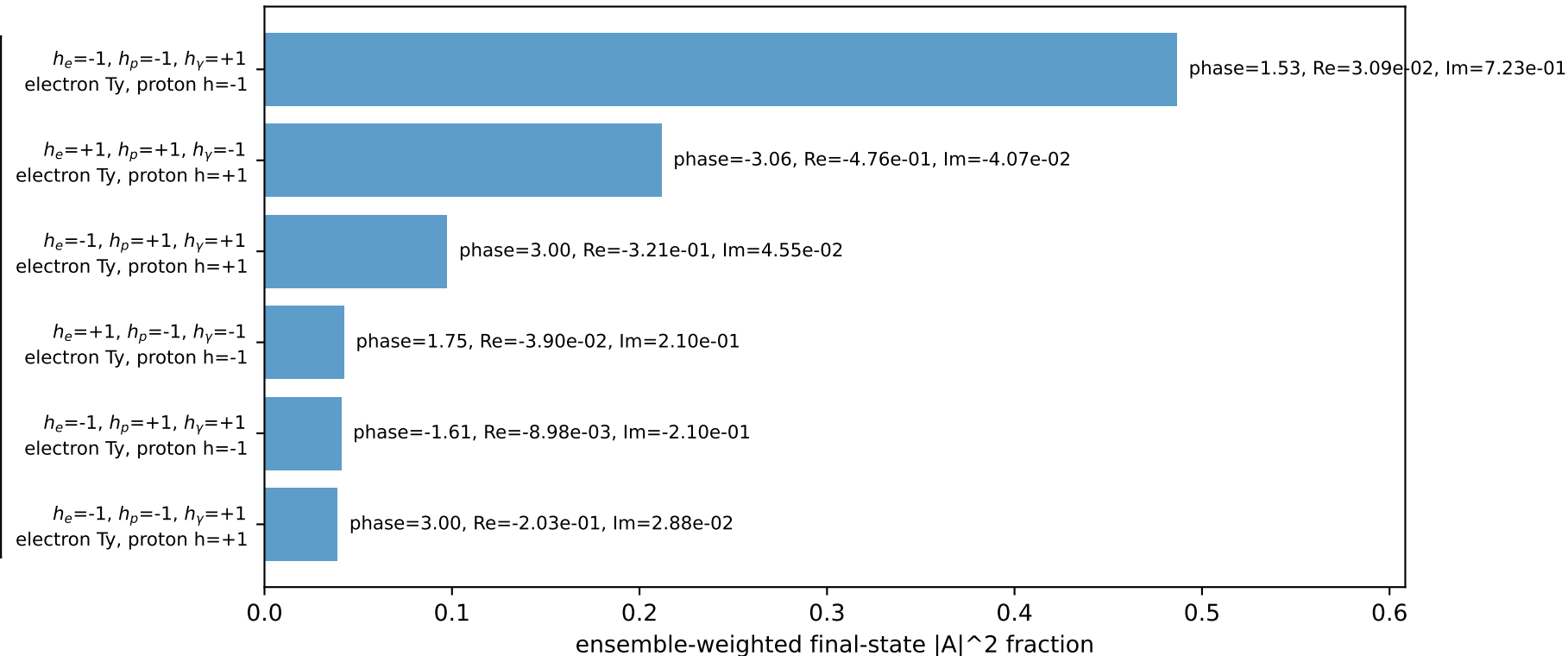
Leading initial-ensemble/final-state components (N=6, retained=91.9%)
