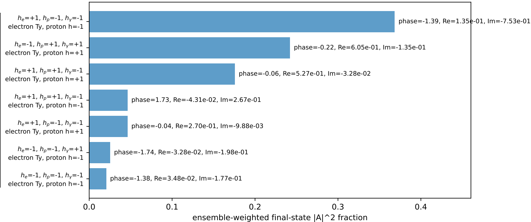
Leading initial-ensemble/final-state components (N=7, retained=92.4%)
