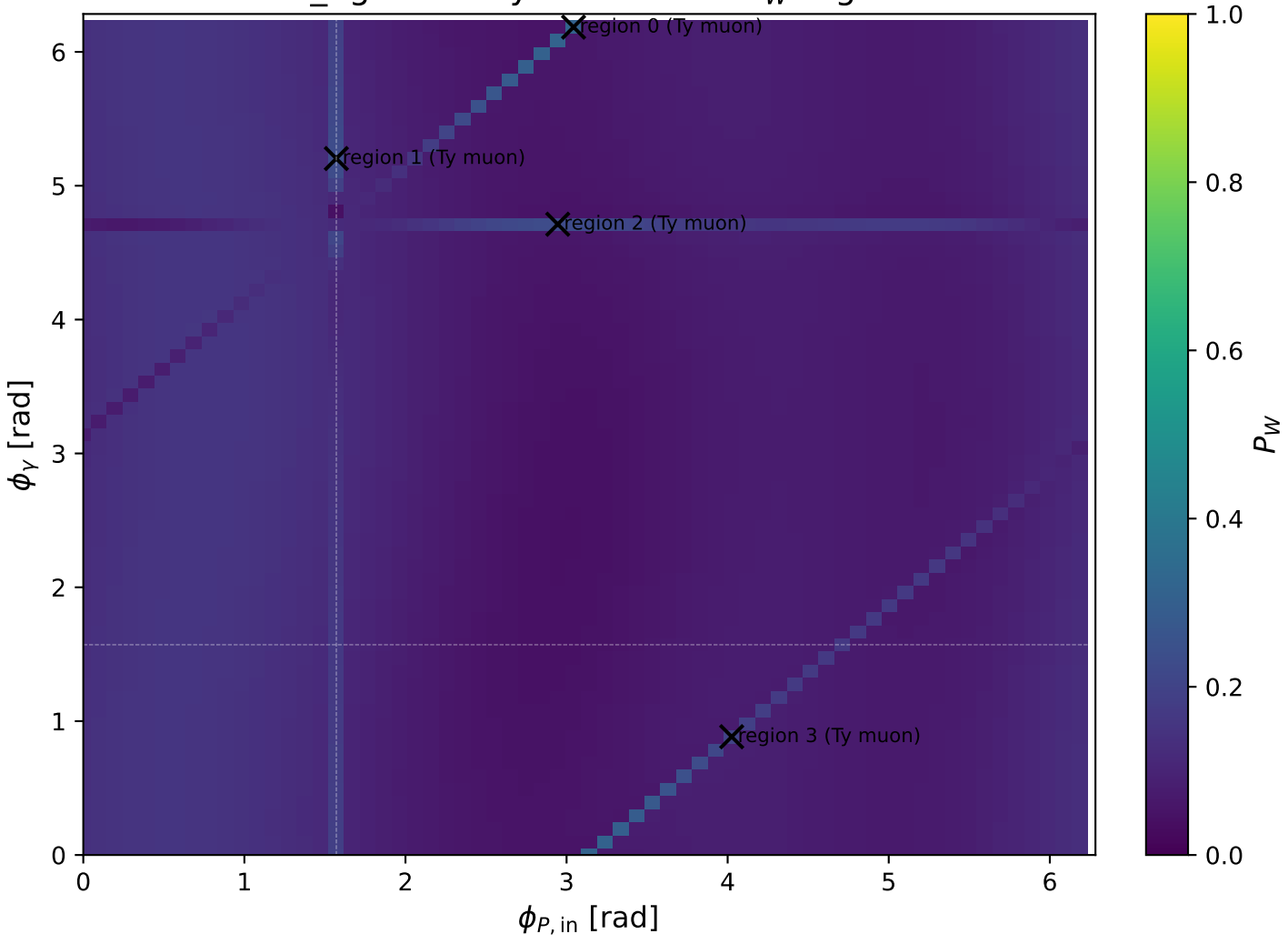
low_Egamma Ty muon: max P_W regions
