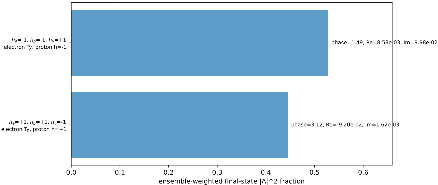
Leading initial-ensemble/final-state components (N=2, retained=97.3%)
