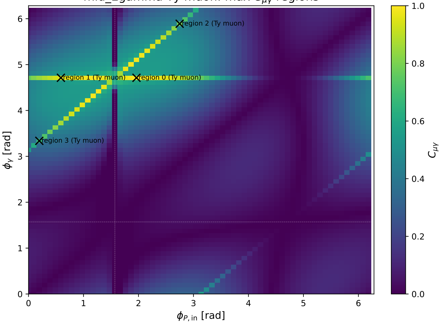
mid_Egamma Ty muon: max C_{\mu\gamma} regions
