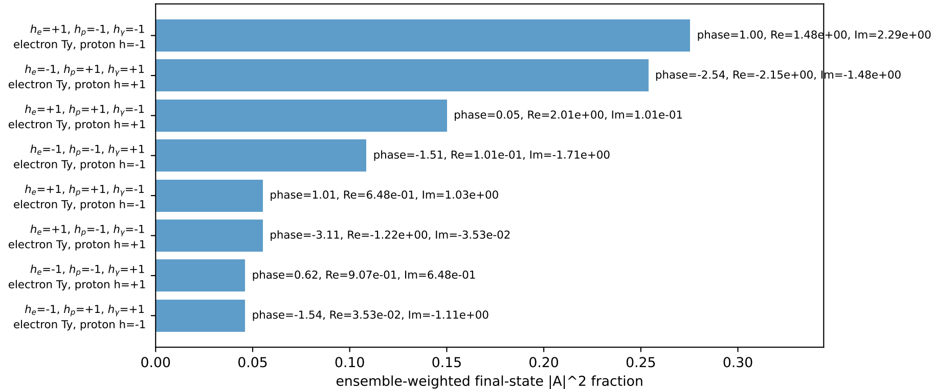
Leading initial-ensemble/final-state components (N=8, retained=99.0%)
