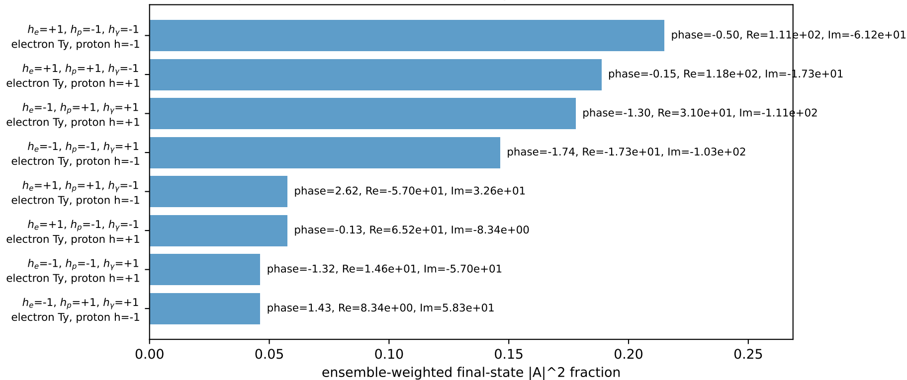
Leading initial-ensemble/final-state components (N=8, retained=93.5%)
