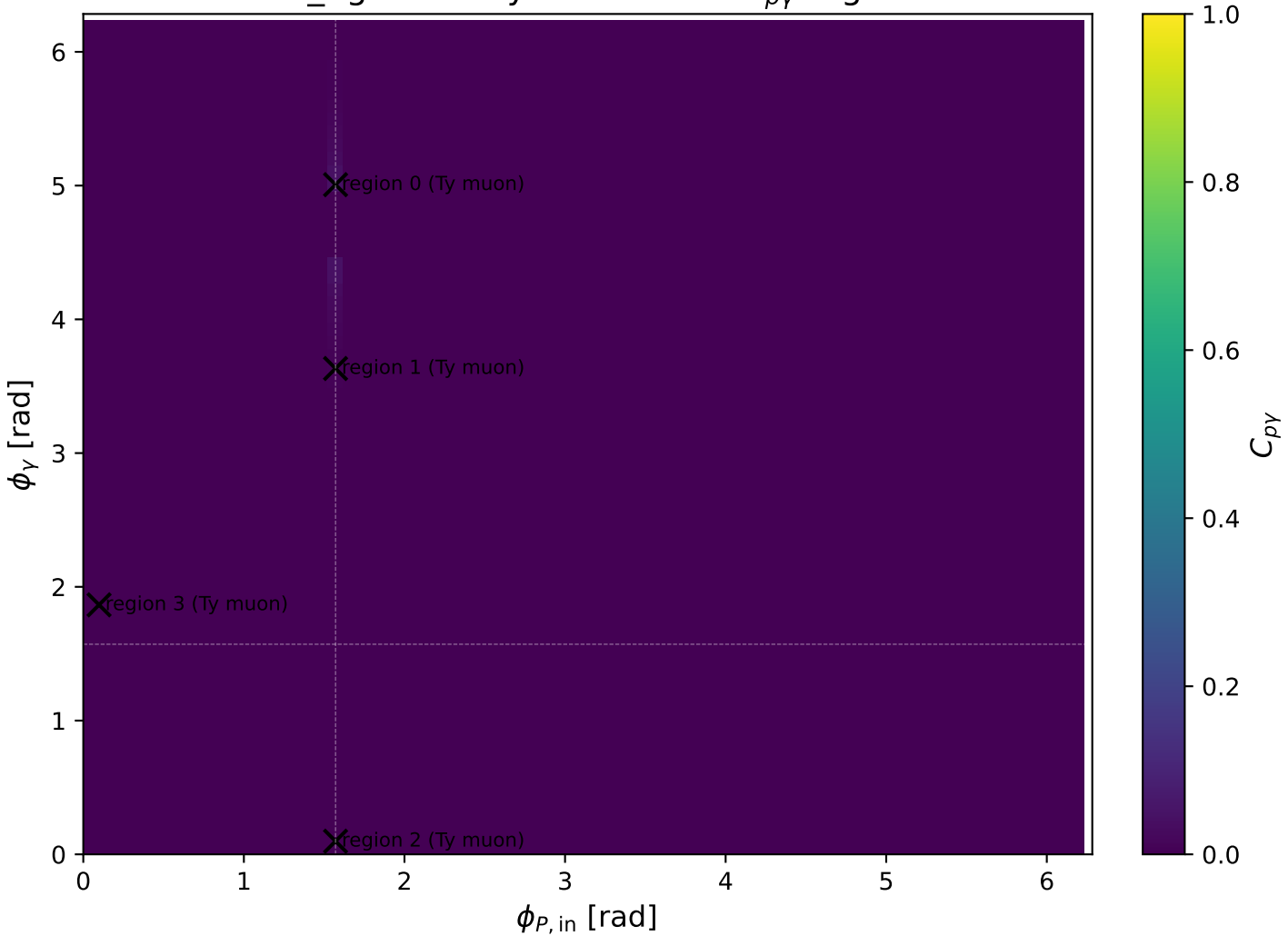
mid_Egamma Ty muon: max C_{p\gamma} regions
