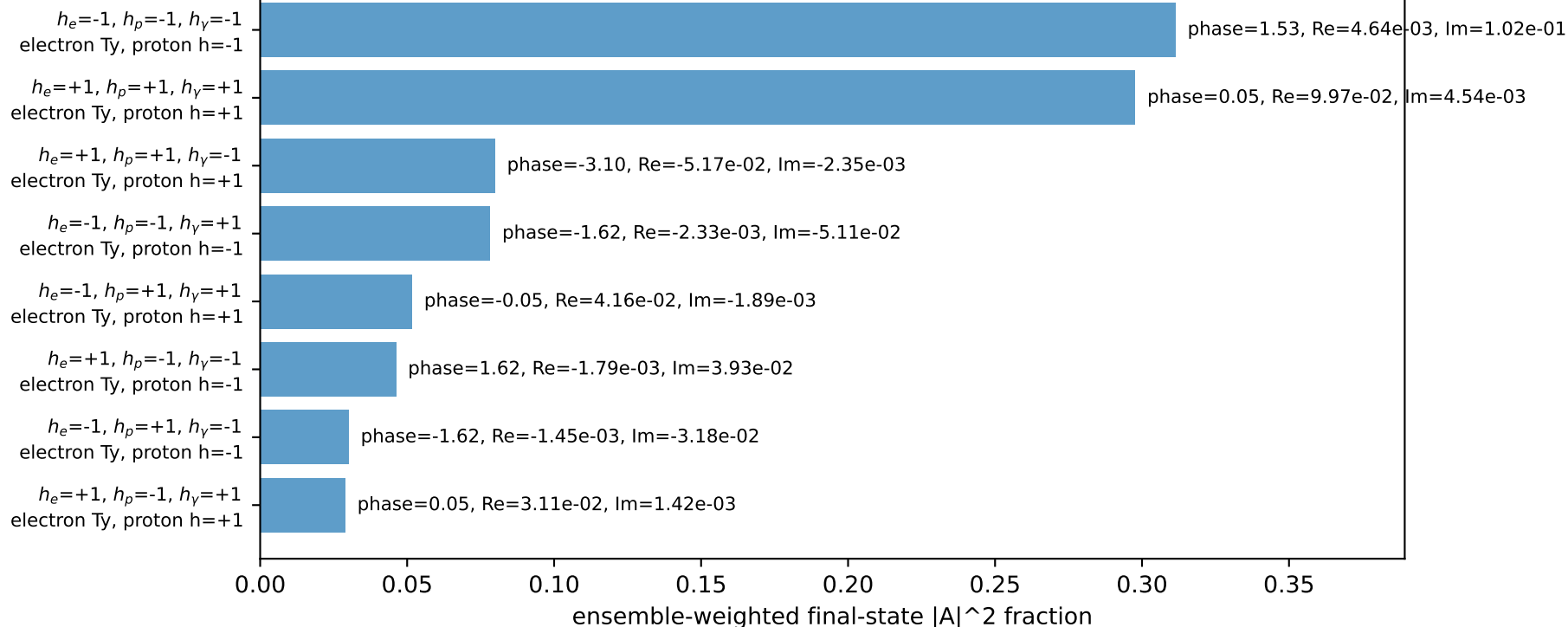
Leading initial-ensemble/final-state components (N=8, retained=92.5%)
