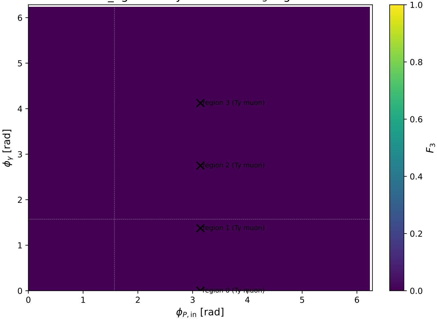
mid_Egamma Ty muon: max F_3 regions
