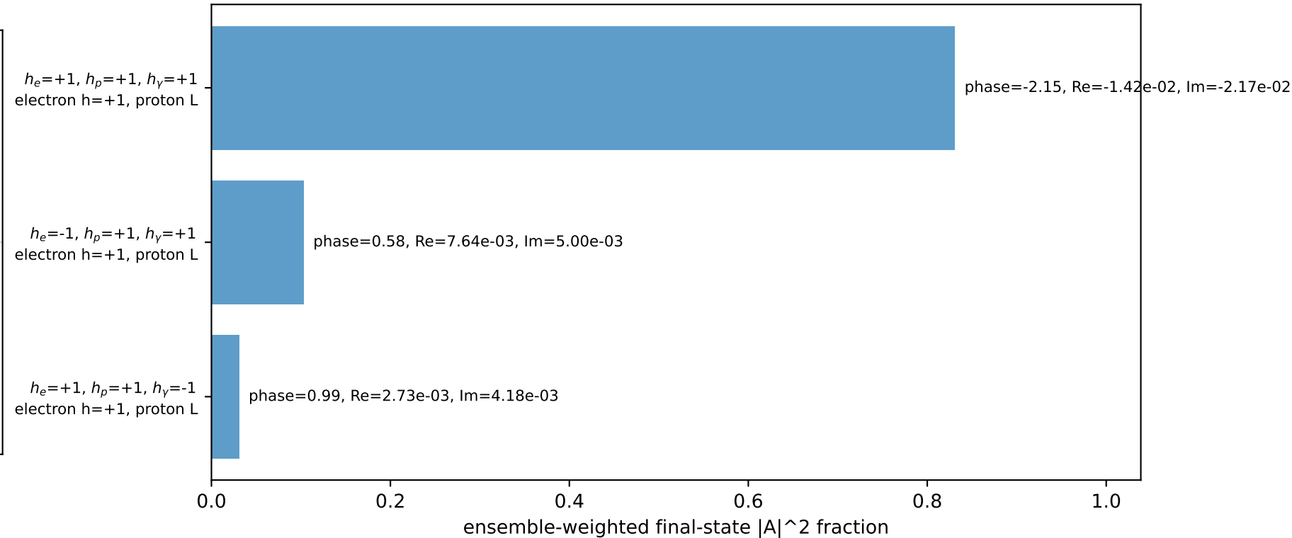
Leading initial-ensemble/final-state components (N=3, retained=96.5%)
