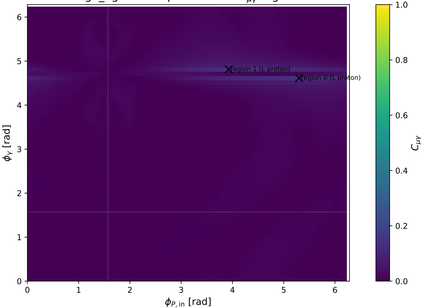
high_Egamma L proton: max C_{\mu\gamma} regions
