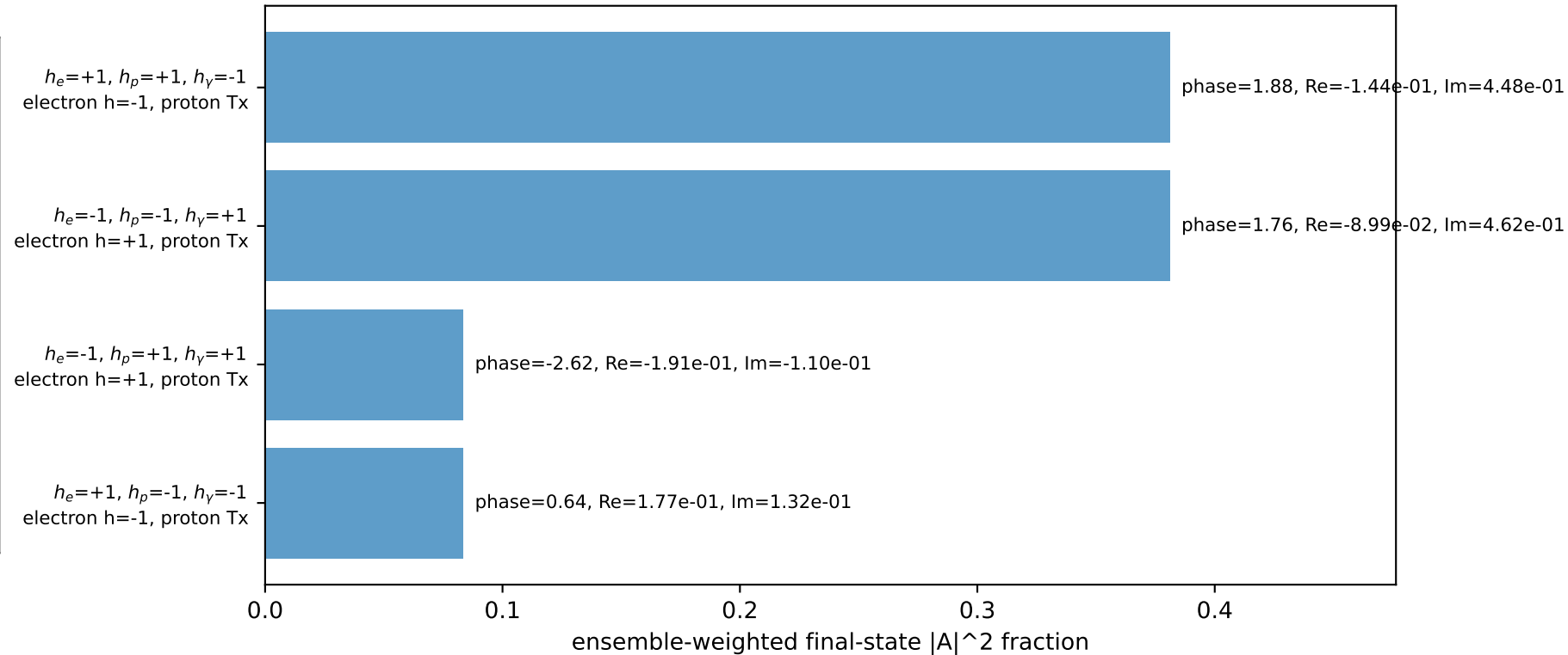
Leading initial-ensemble/final-state components (N=4, retained=92.9%)
