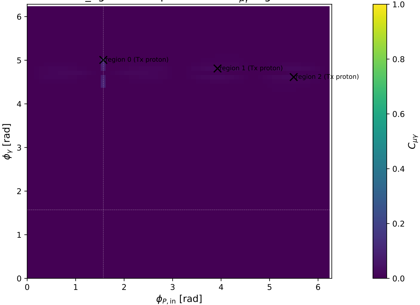
mid_Egamma Tx proton: max C_{\mu\gamma} regions
