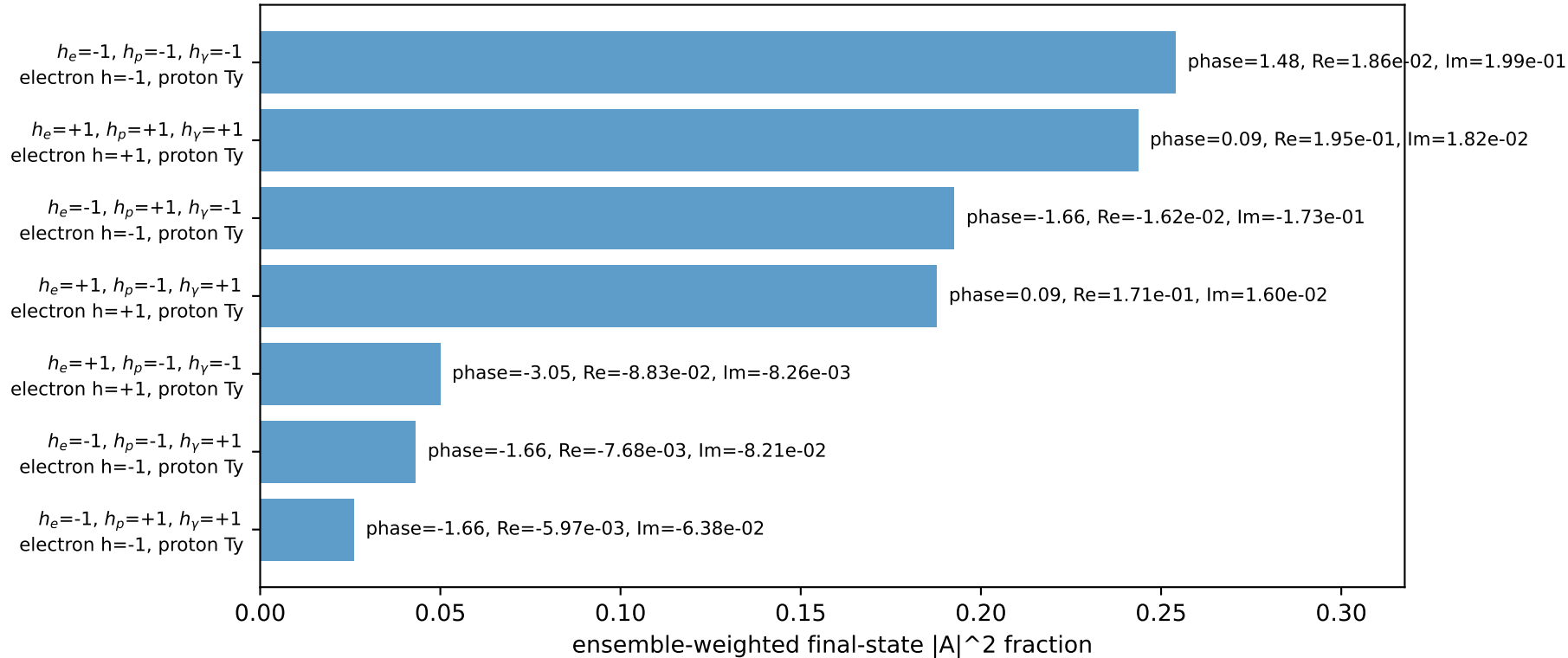
Leading initial-ensemble/final-state components (N=7, retained=99.7%)
