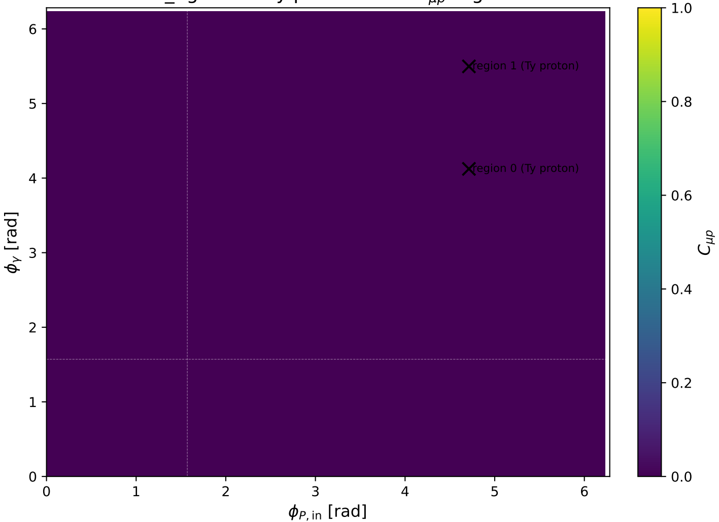
low_Egamma Ty proton: max C_{\mu p} regions
