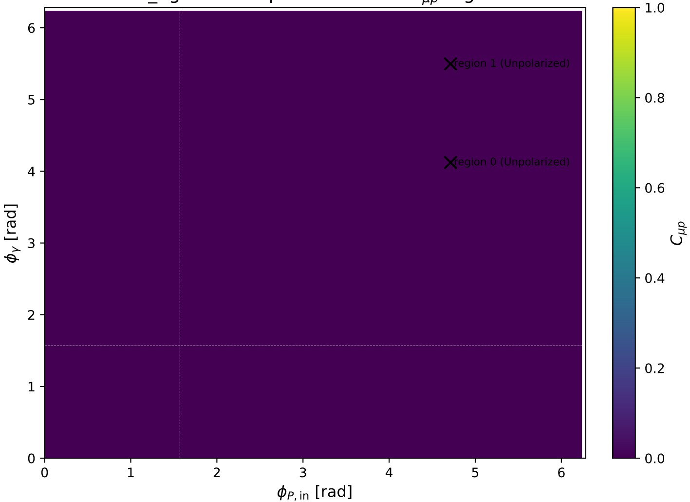
low_Egamma Unpolarized: max C_{\mu p} regions
