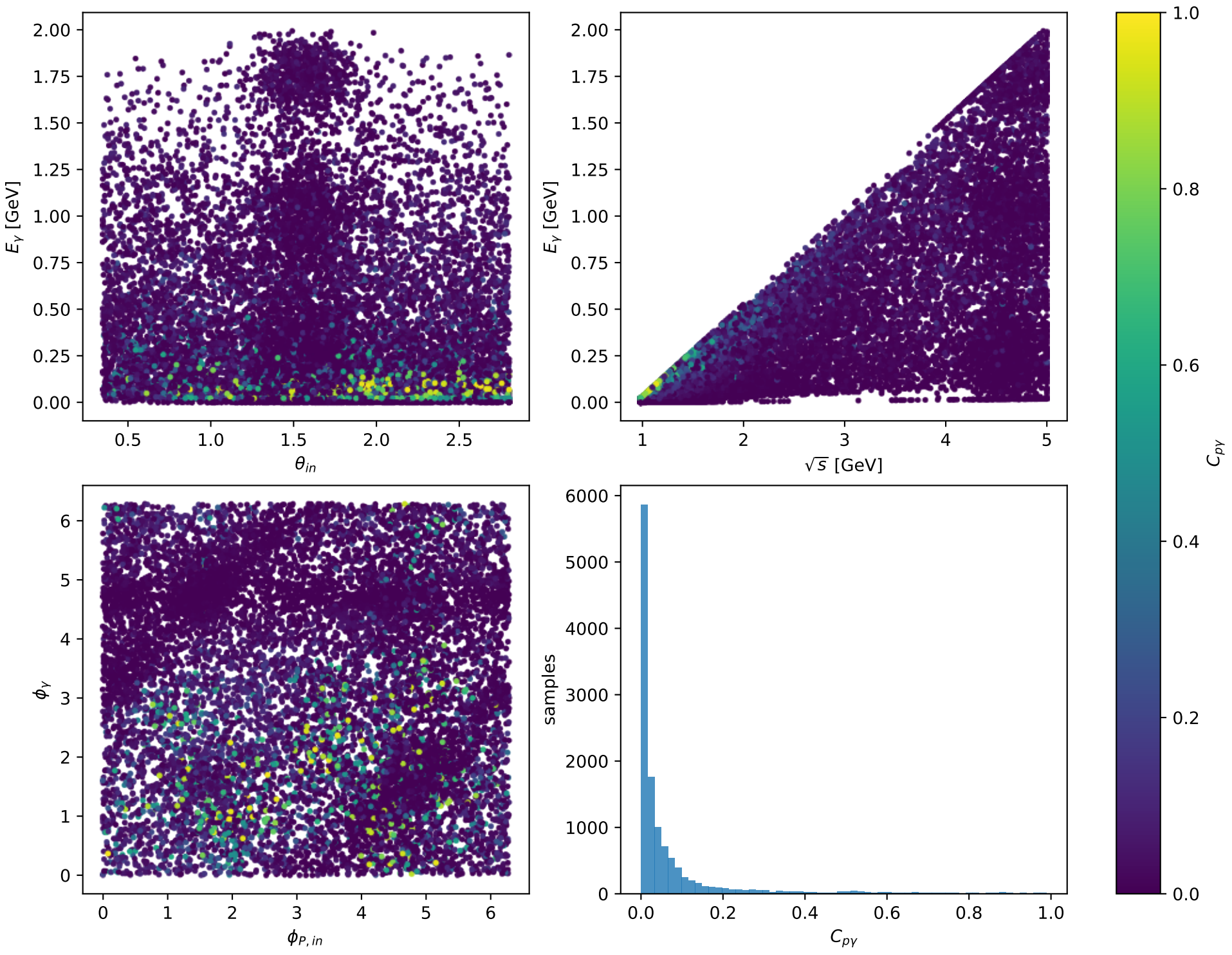
Phase-space scan: L electron + L proton [LL], max C_{p\gamma}=0.98992
