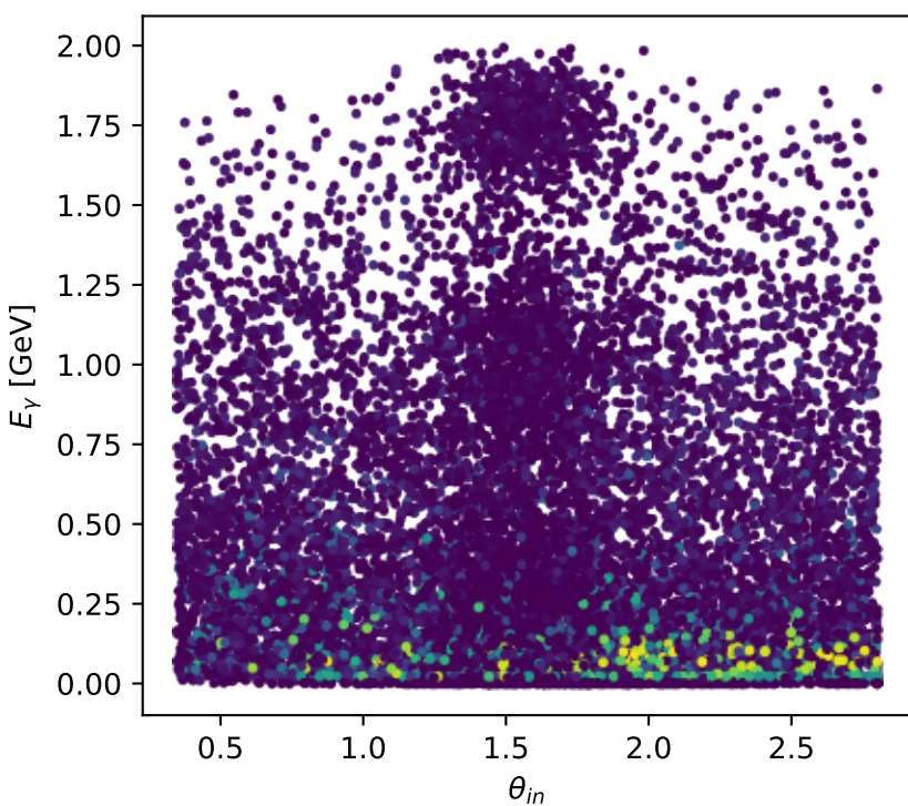
Phase-space scan: L electron + L proton [LL], max C_{\gamma|ep}=0.98993
