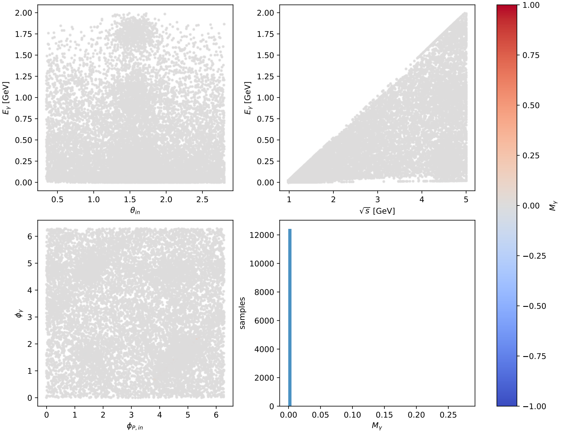
Phase-space scan: L electron + L proton [LL], max M_\gamma=0.27785
