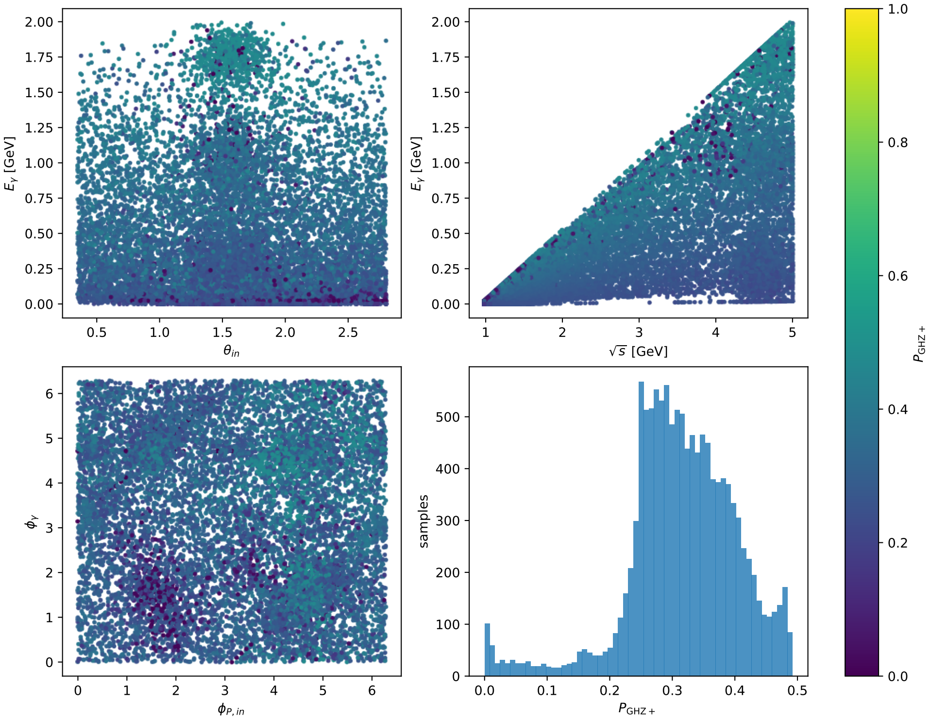
Phase-space scan: L electron + L proton [LL], max P_{\text{GHZ}+}=0.49212
