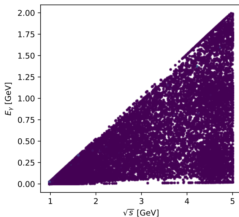
Phase-space scan: L electron + L proton [LL], max C_{e|py}=0.96338
