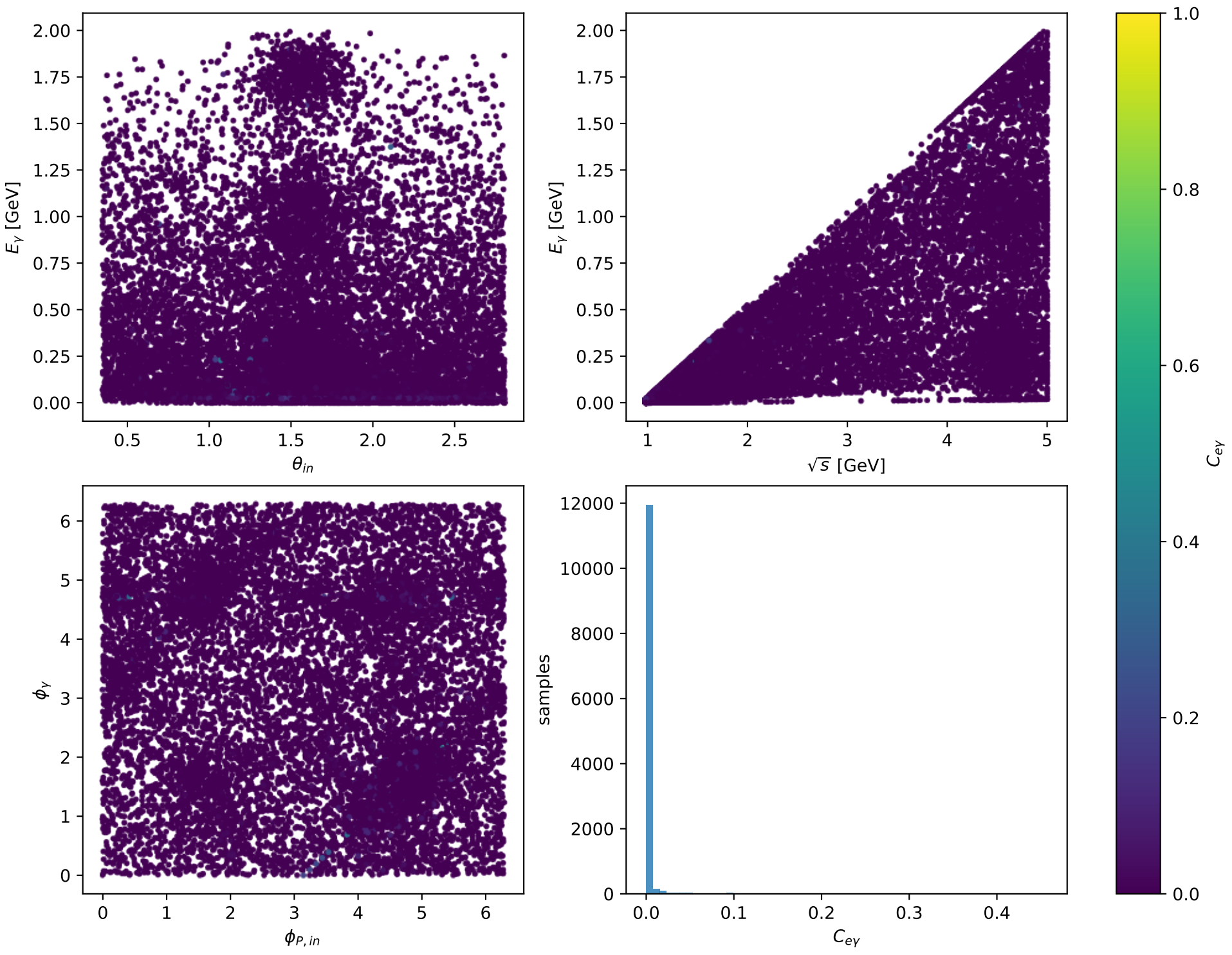
Phase-space scan: L electron + L proton [LL], max C_{e\gamma}=0.45726
