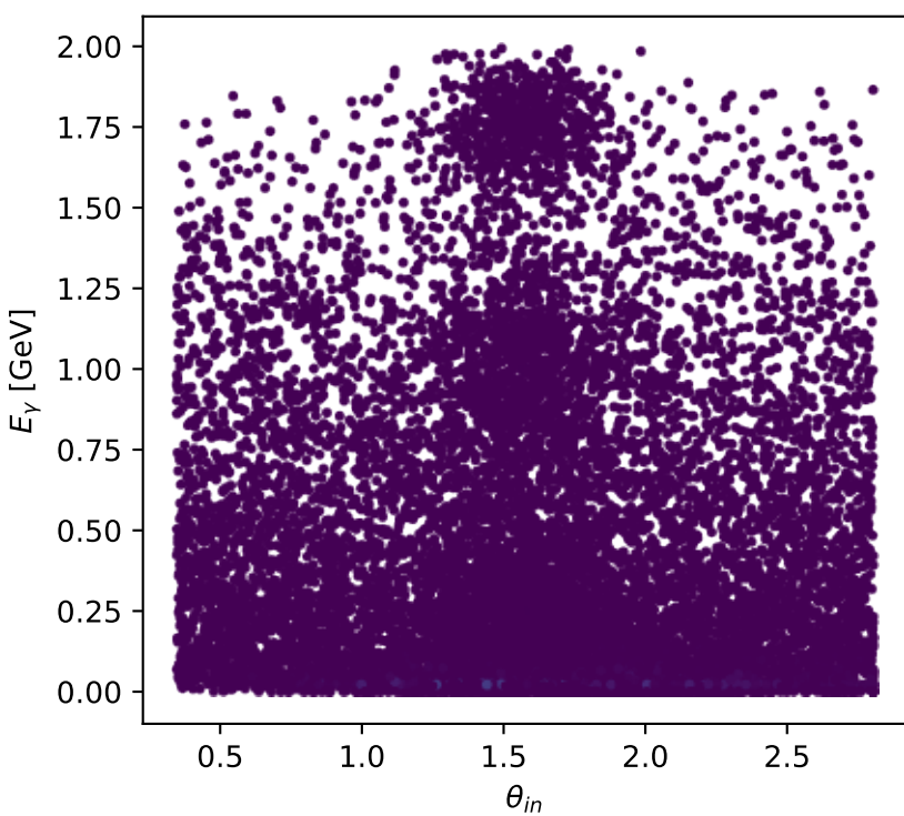
Phase-space scan: L electron + L proton [LL], max F_3=0.56861
