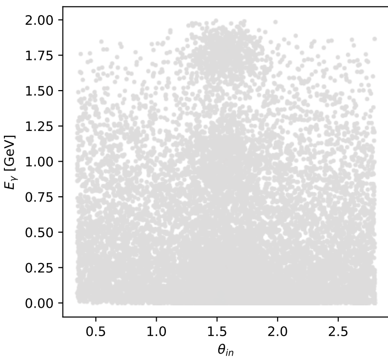
Phase-space scan: L electron + L proton [LL], max M_e=0.27785
