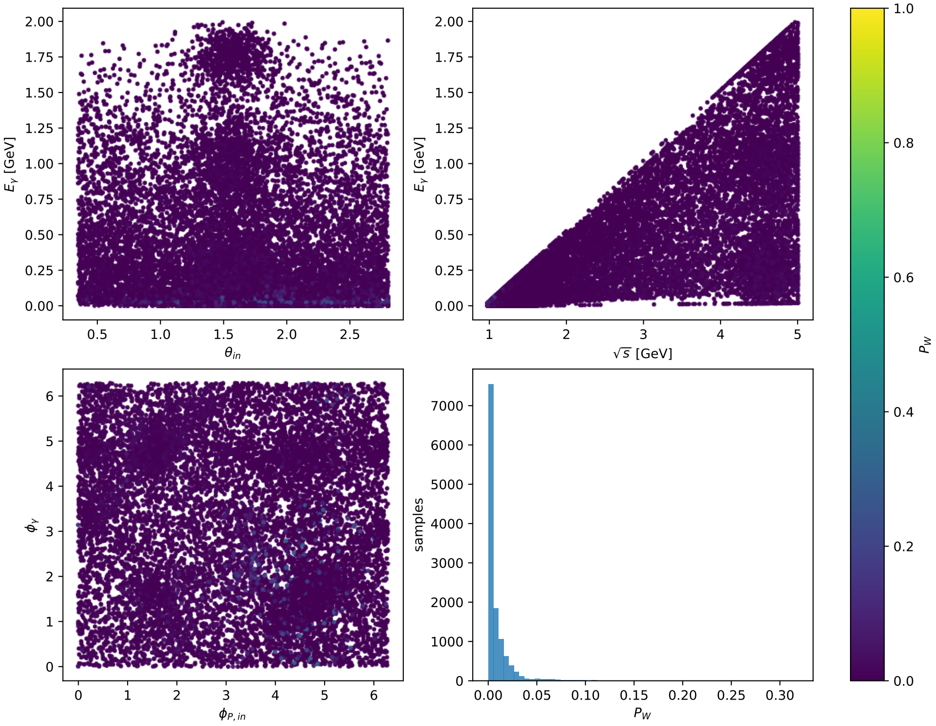
Phase-space scan: L electron + L proton [LL], max P_W=0.31821
