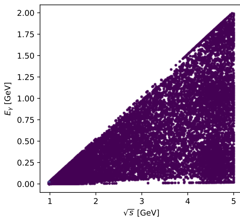
Phase-space scan: L electron + L proton [LL], max C_{ep}=0.83779
