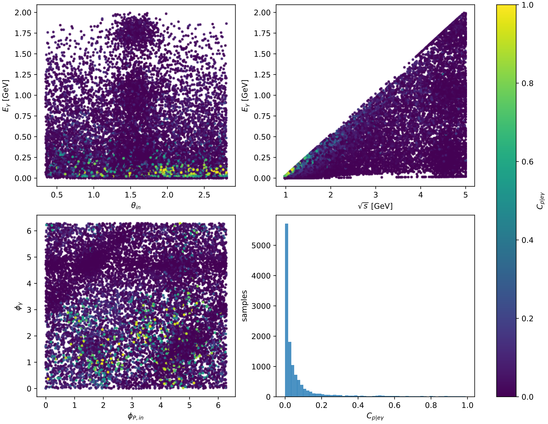
Phase-space scan: L electron + L proton [LL], max C_{p|ey}=0.98993
