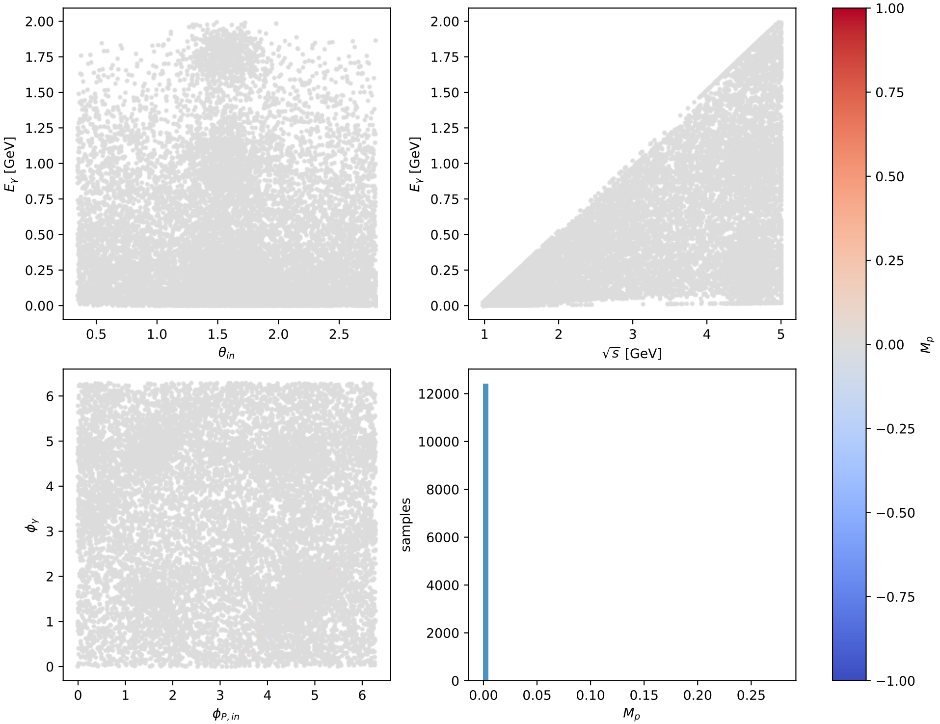
Phase-space scan: L electron + L proton [LL], max M_p=0.27785
