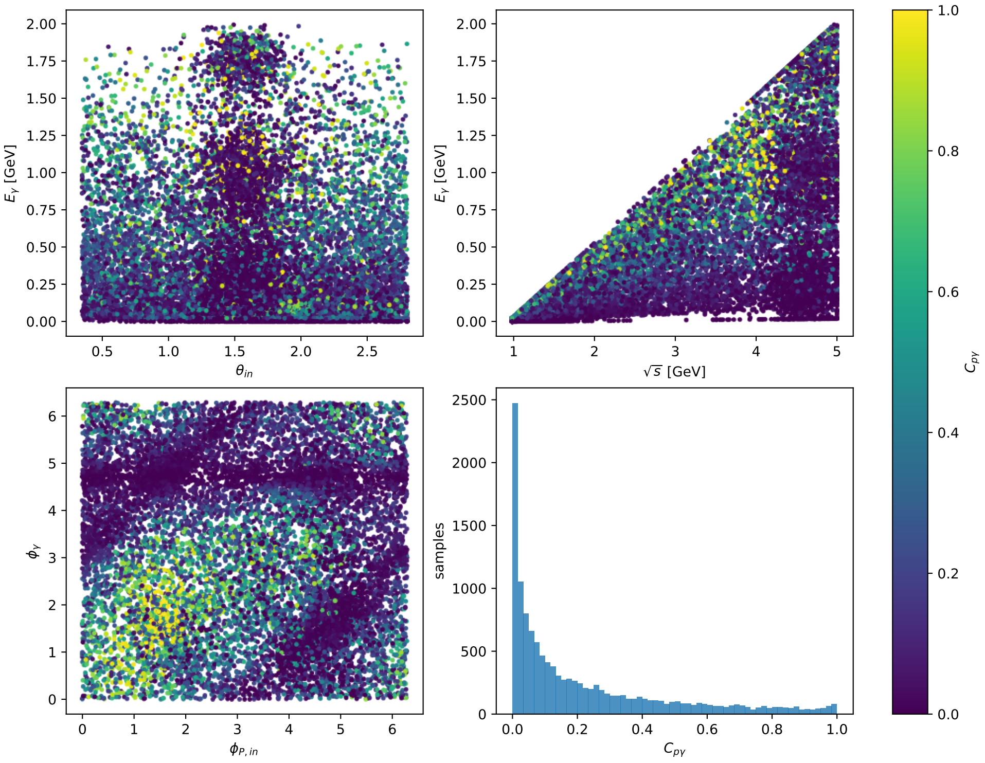
Phase-space scan: L electron + Tx proton [LTx], max C_{py}=0.99999
