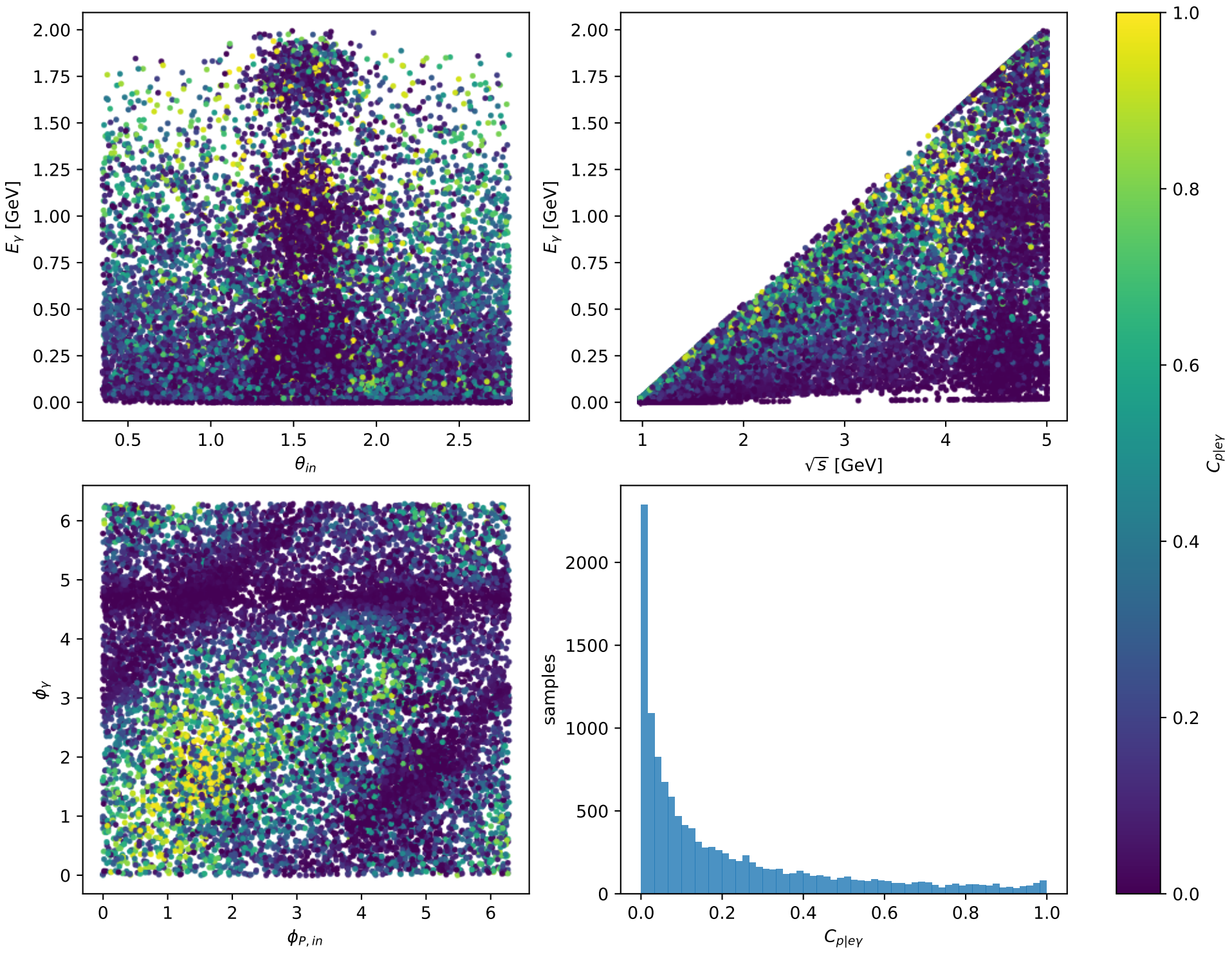
Phase-space scan: L electron + Tx proton [LTx], max C_{p|e\gamma}=0.99999
