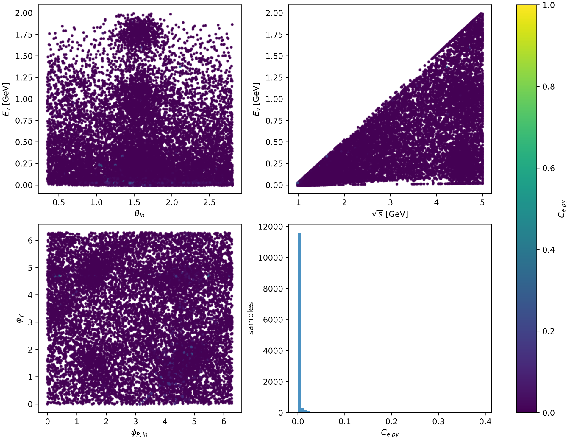
Phase-space scan: L electron + Tx proton [LTx], max C_{e|p\gamma}=0.39386
