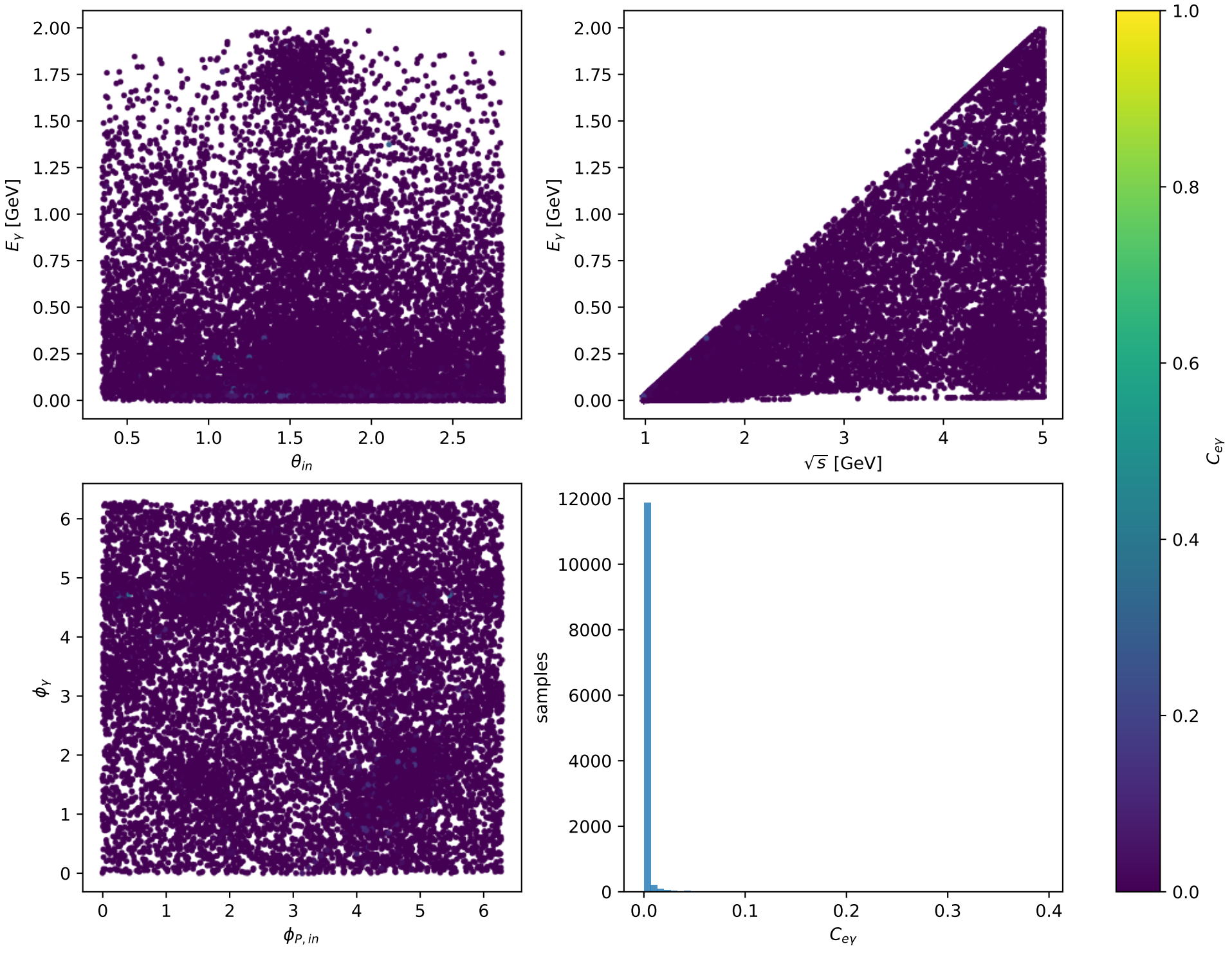
Phase-space scan: L electron + Tx proton [LTx], max C_{ey}=0.39386
