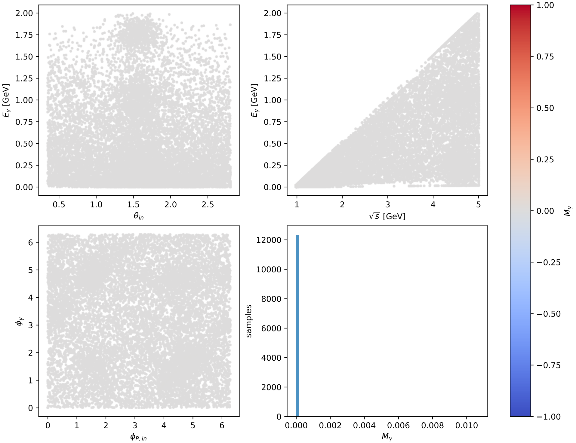
Phase-space scan: L electron + Tx proton [LTx], max M_\gamma=0.010701
