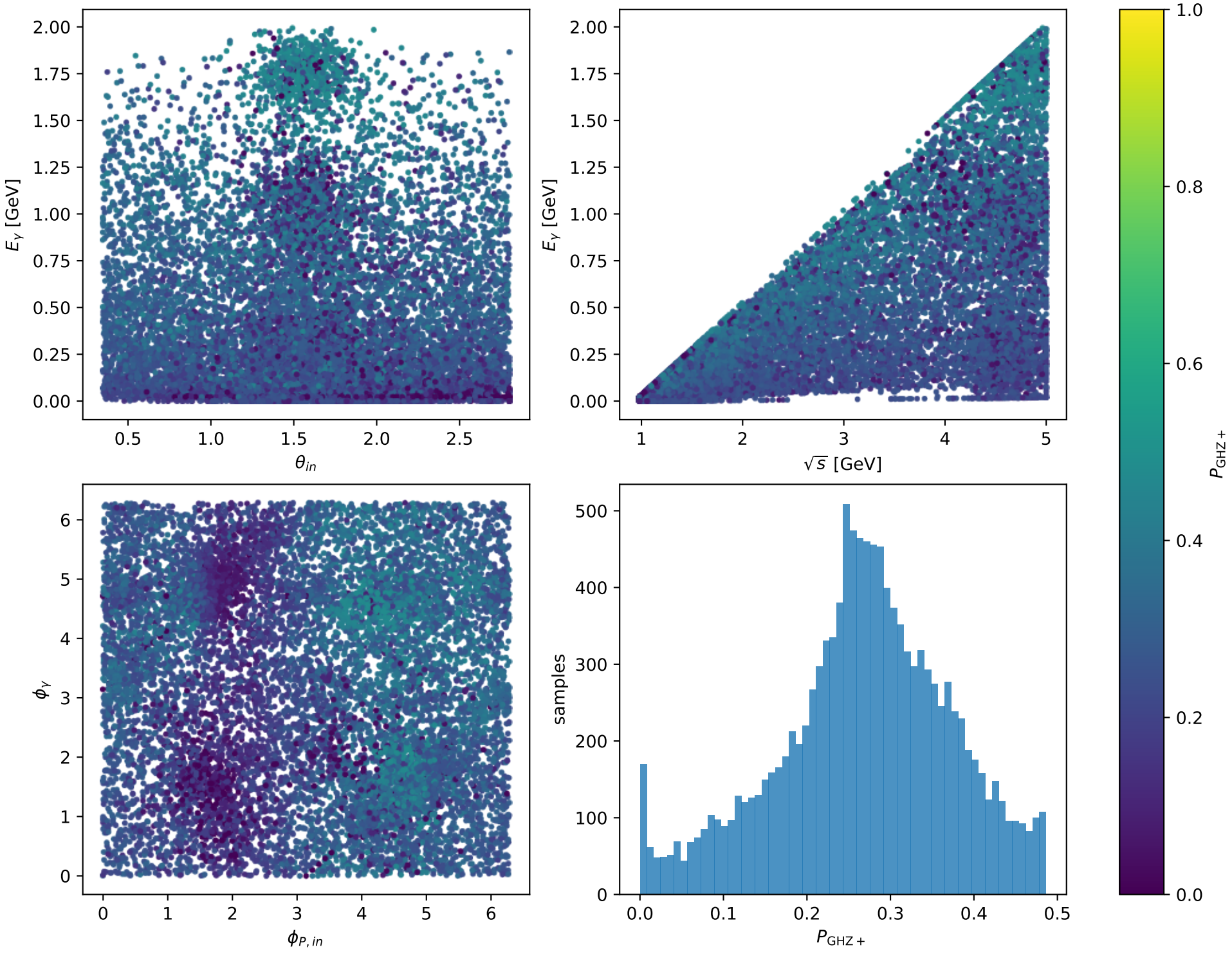
Phase-space scan: L electron + Tx proton [LTx], max P_{\text{GHZ}+}=0.48657
