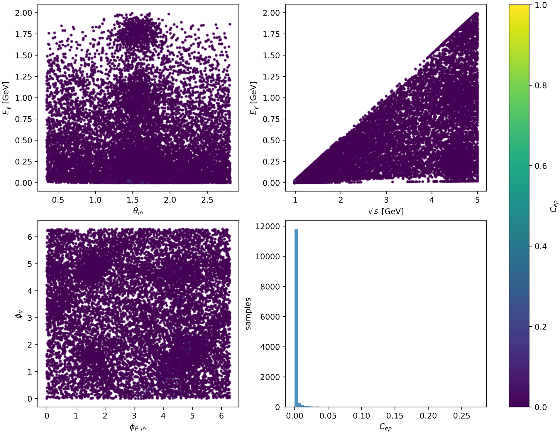
Phase-space scan: L electron + Tx proton [LTx], max C_{ep}=0.27355
