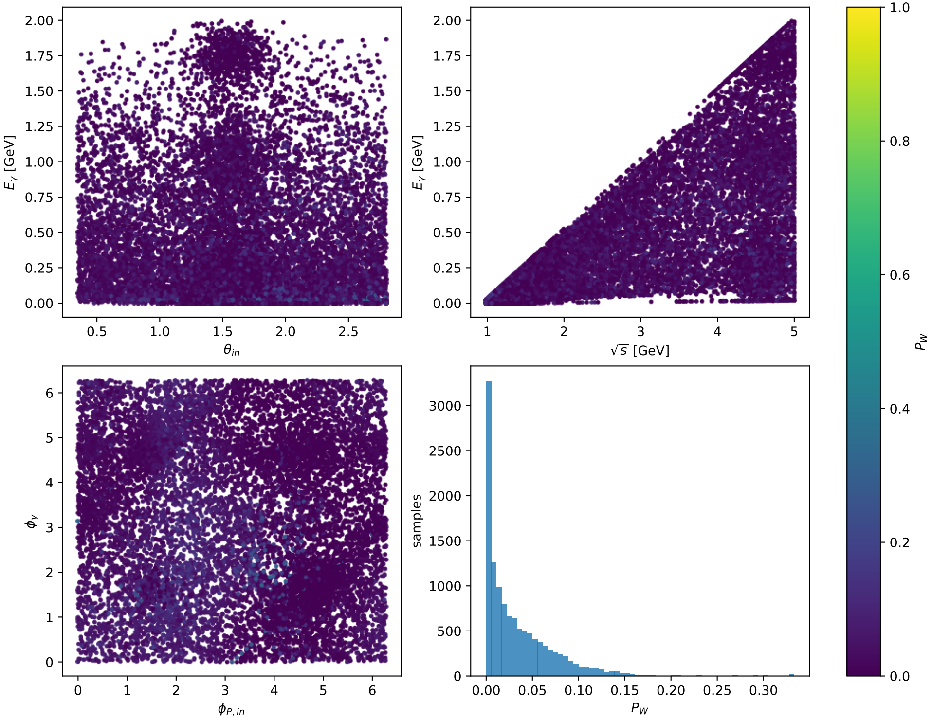
Phase-space scan: L electron + Tx proton [LTx], max P_W=0.33332
