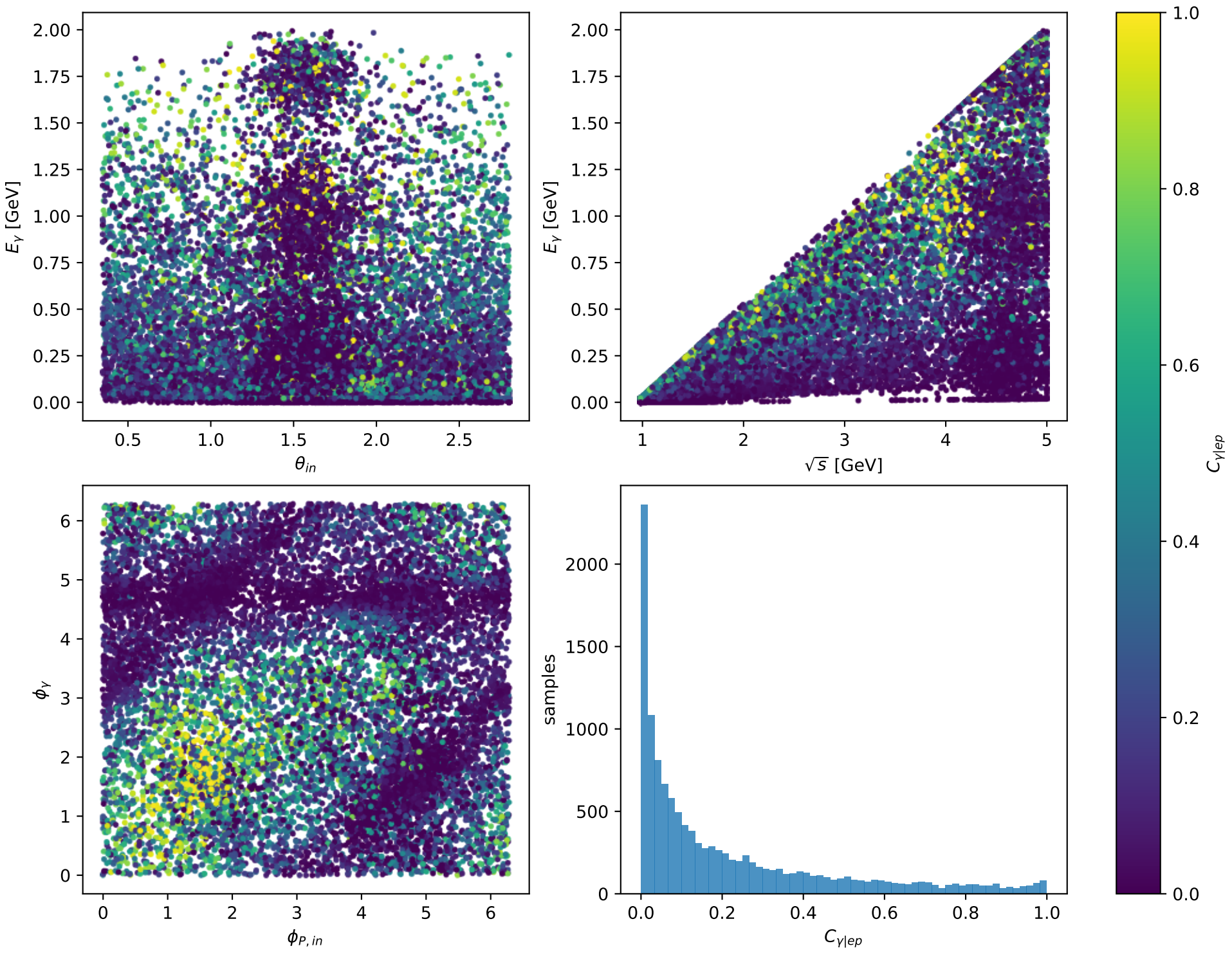
Phase-space scan: L electron + Tx proton [LTx], max C_{\gamma|ep}=0.99999
