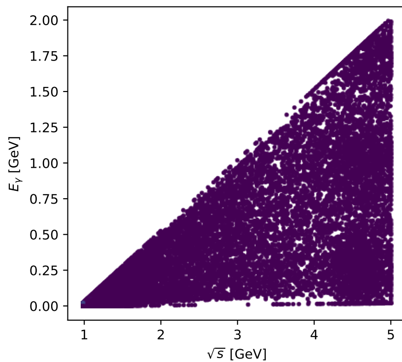
Phase-space scan: L electron + Tx proton [LTx], max F_3=0.26764
