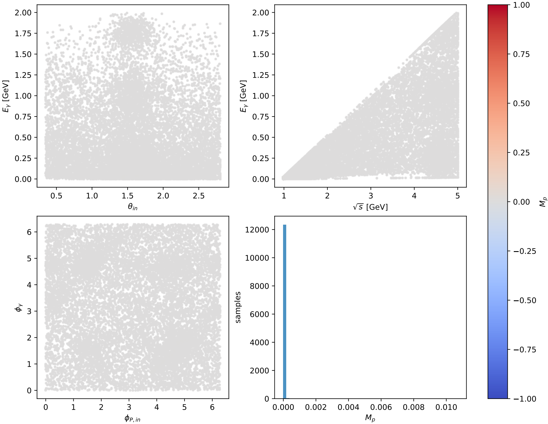
Phase-space scan: L electron + Tx proton [LTx], max M_p=0.010701
