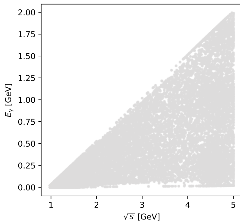
Phase-space scan: L electron + Tx proton [LTx], max M_e=0.010701
