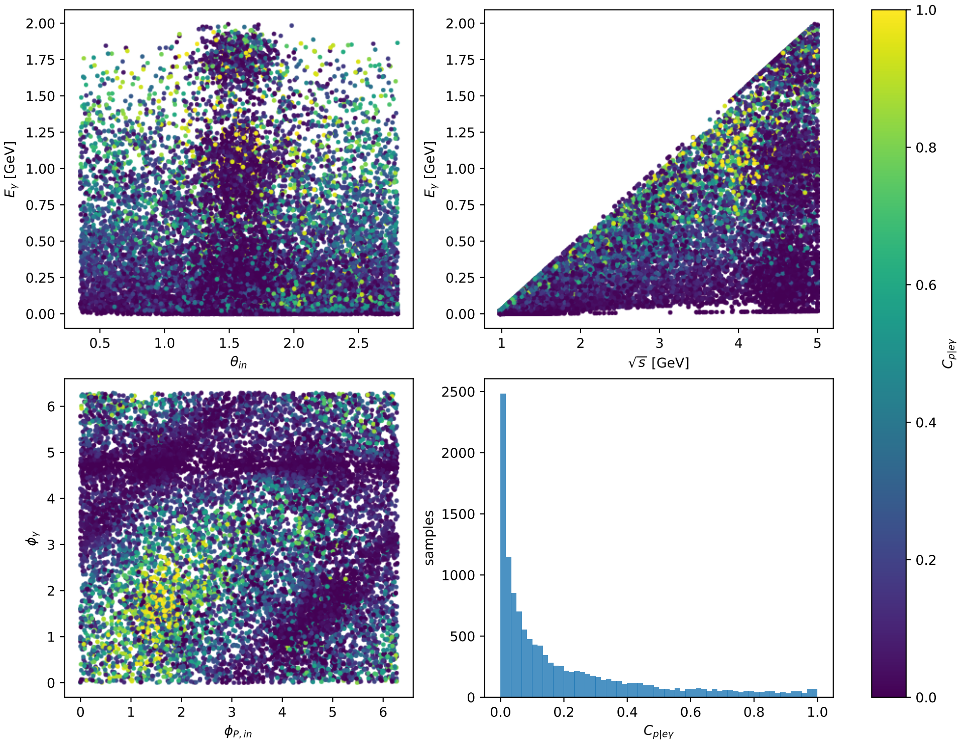
Phase-space scan: L electron + Ty proton [LTy], max C_{p|e\gamma}=0.99999
