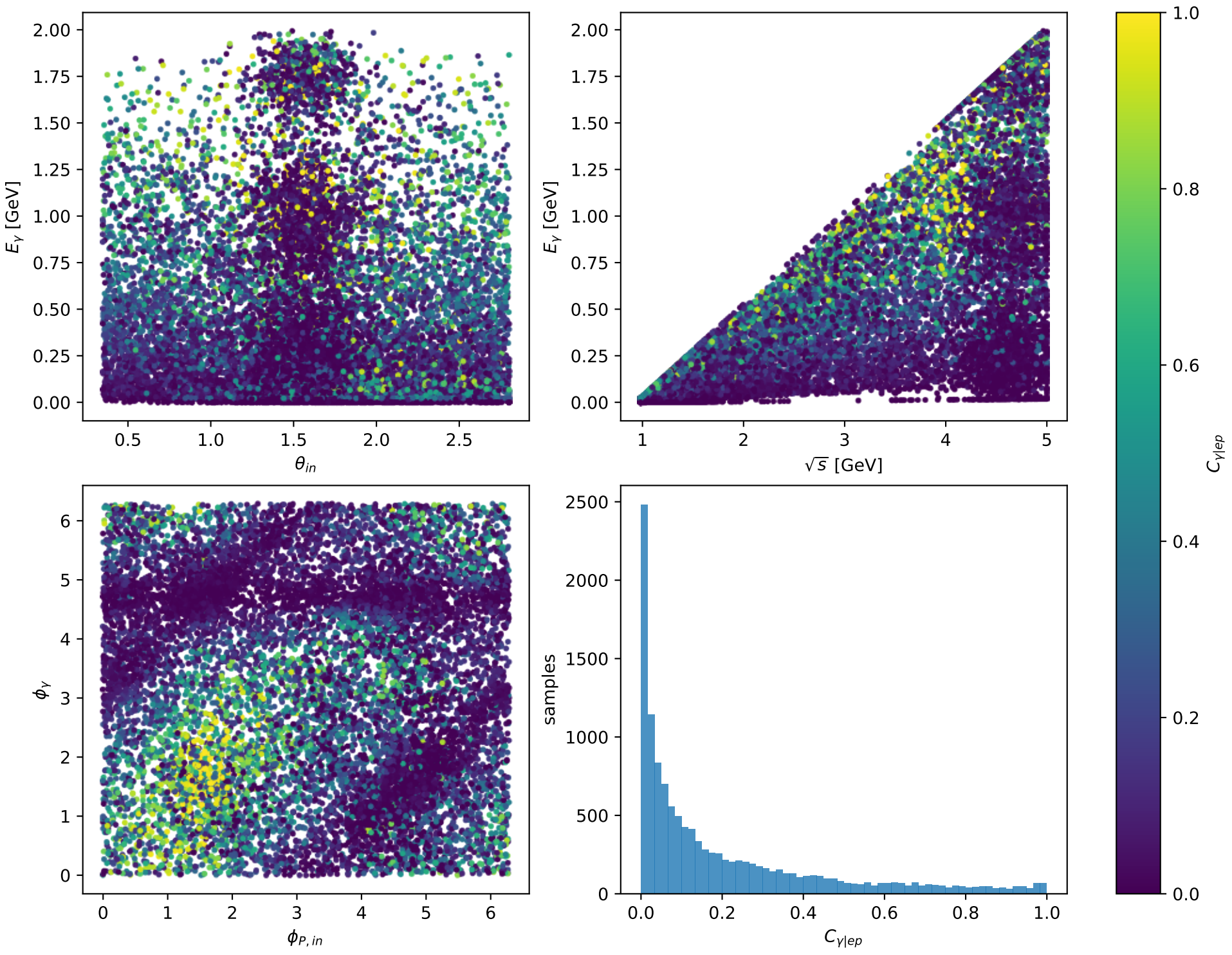
Phase-space scan: L electron + Ty proton [LTy], max C_{\gamma|ep}=0.99999
