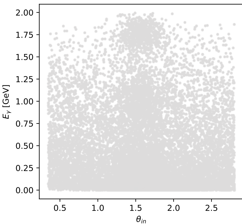
Phase-space scan: L electron + Ty proton [LTy], max M_e=0.016235
