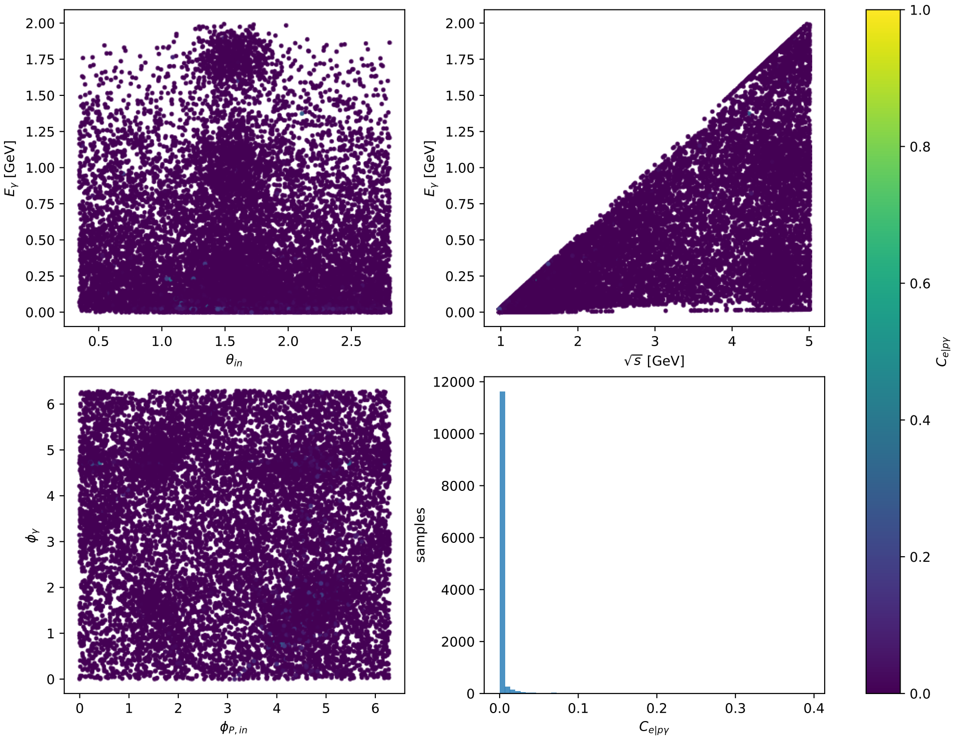
Phase-space scan: L electron + Ty proton [LTy], max C_{e|p\gamma}=0.39388
