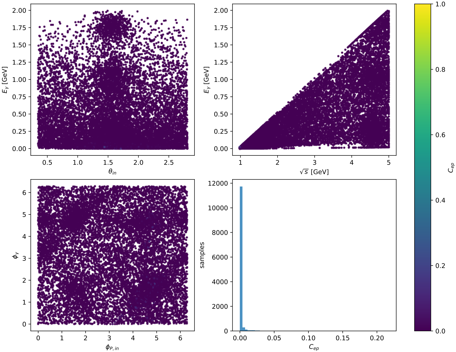
Phase-space scan: L electron + Ty proton [LTy], max C_{ep}=0.21729
