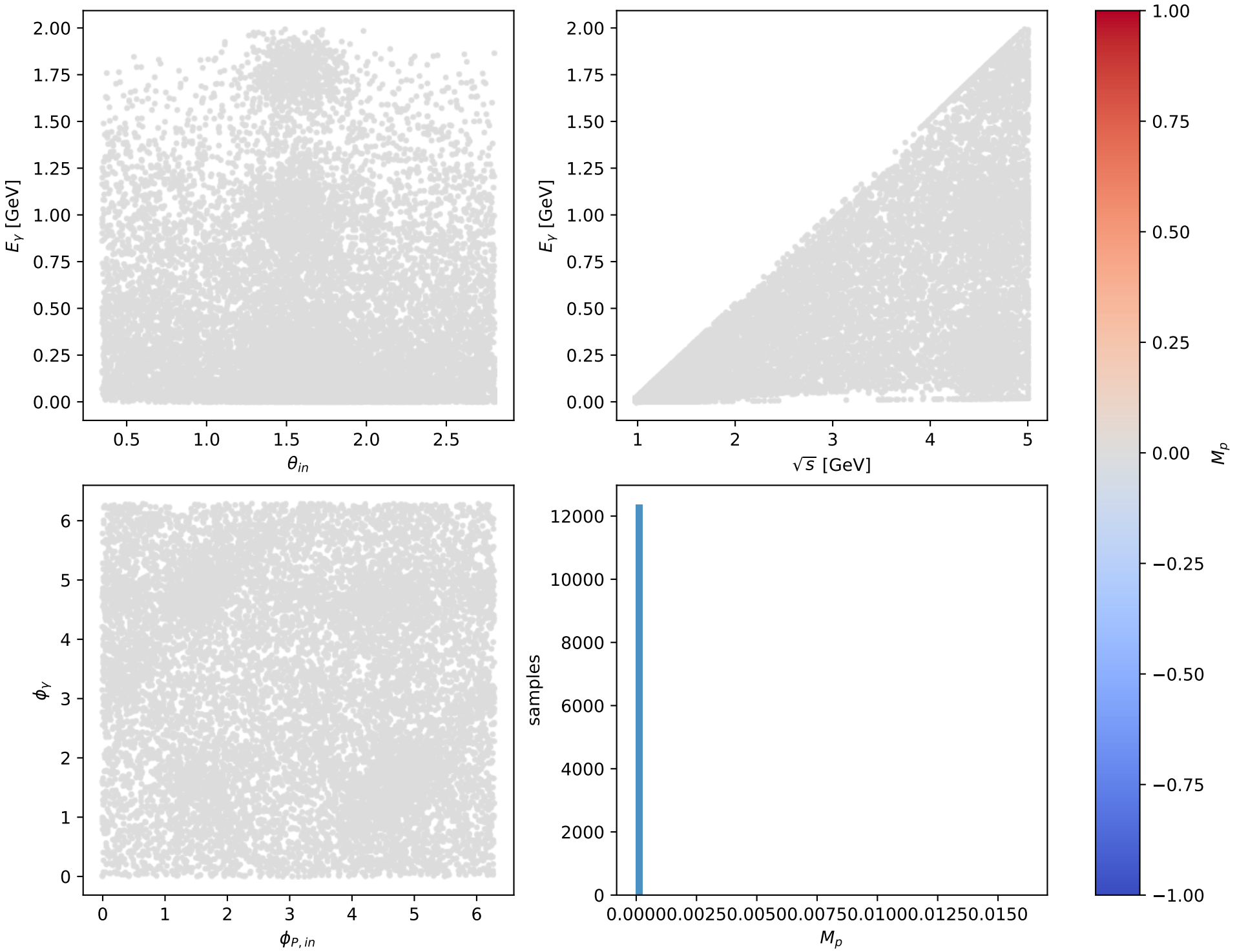
Phase-space scan: L electron + Ty proton [LTy], max M_p=0.016235
