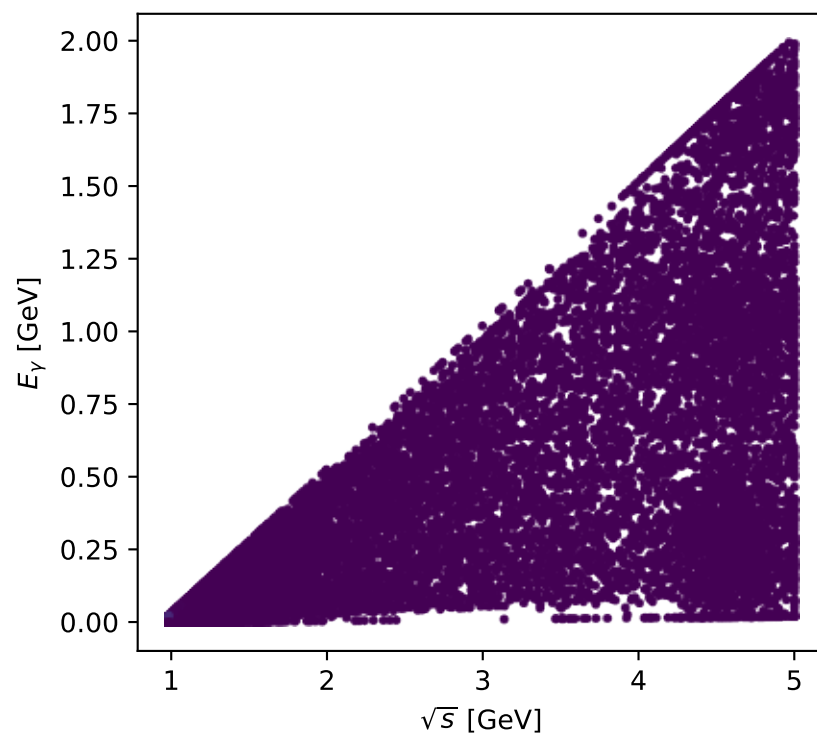
Phase-space scan: L electron + Ty proton [LTy], max F_3=0.2628
