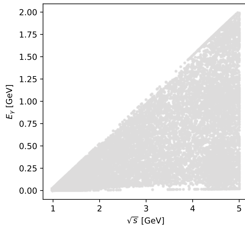
Phase-space scan: L electron + Ty proton [LTy], max M_\gamma=0.016235
