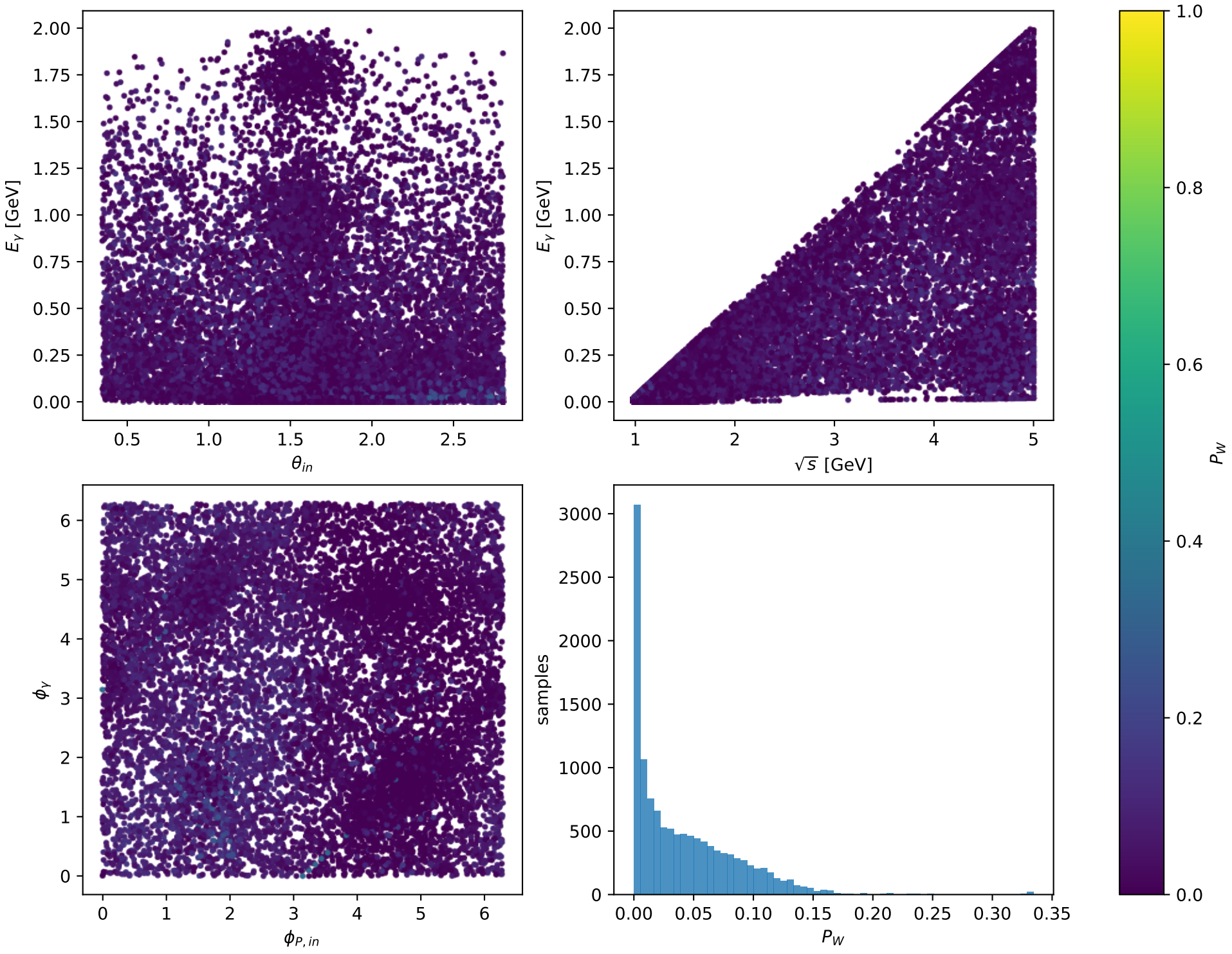
Phase-space scan: L electron + Ty proton [LTy], max P_W=0.33446
