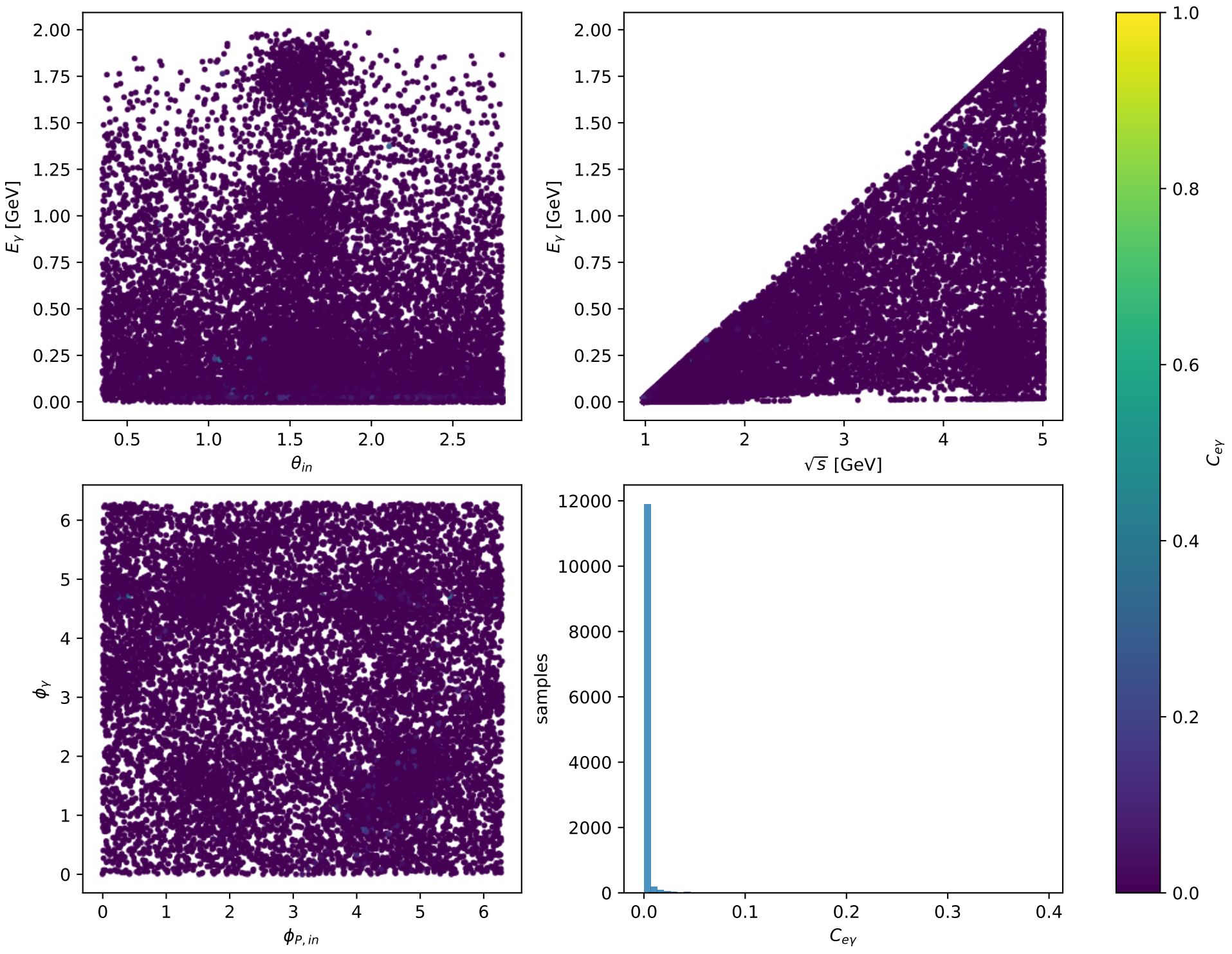
Phase-space scan: L electron + Ty proton [LTy], max C_{ey}=0.39388
