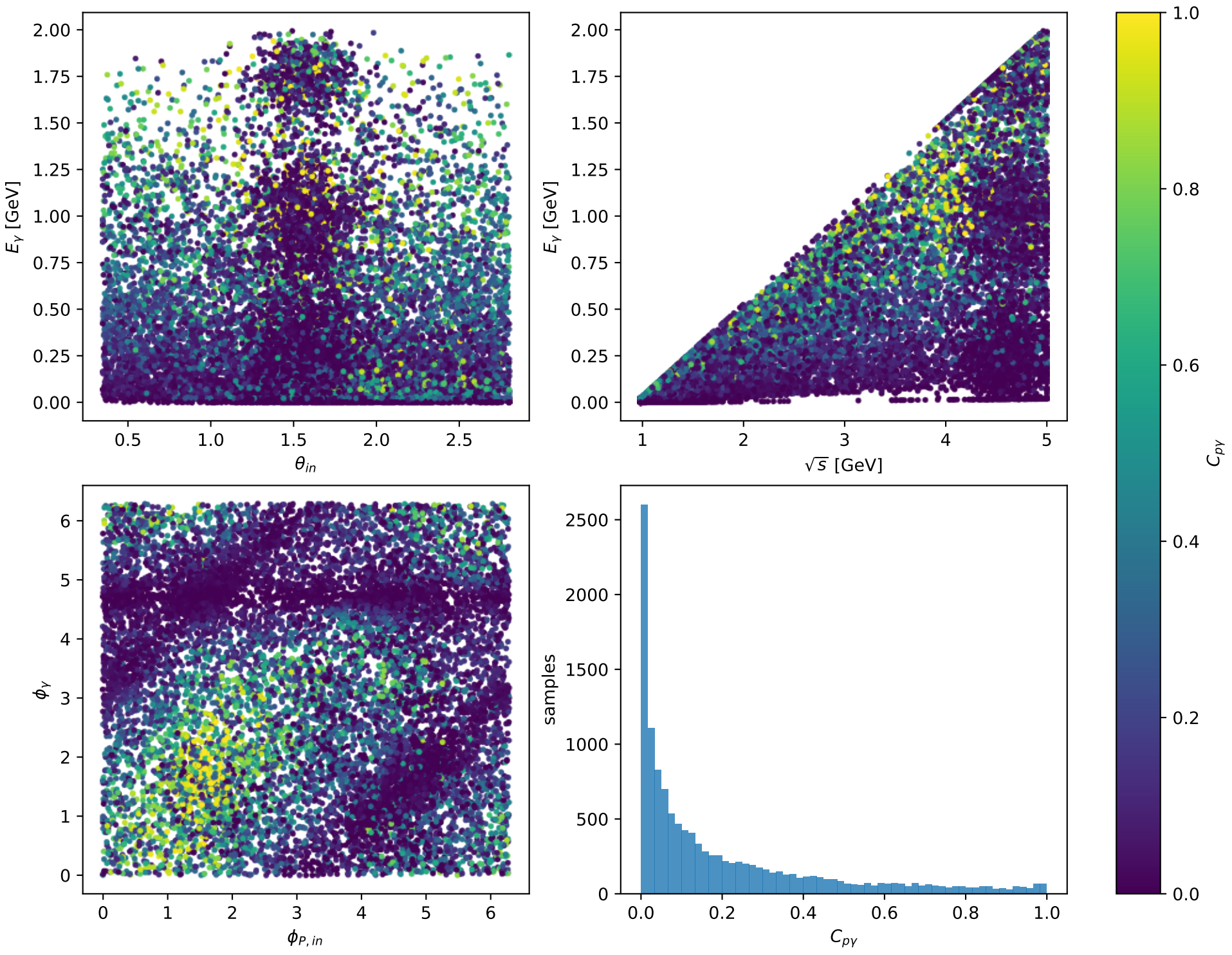
Phase-space scan: L electron + Ty proton [LTy], max C_{py}=0.99999
