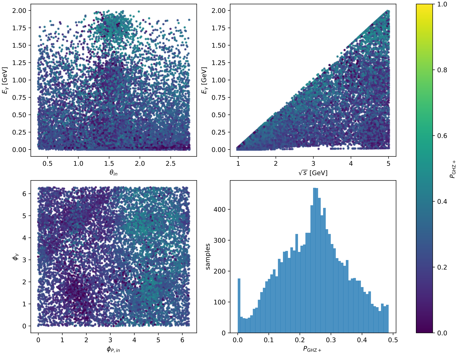
Phase-space scan: L electron + Ty proton [LTy], max P_{\text{GHZ}+}=0.4853
