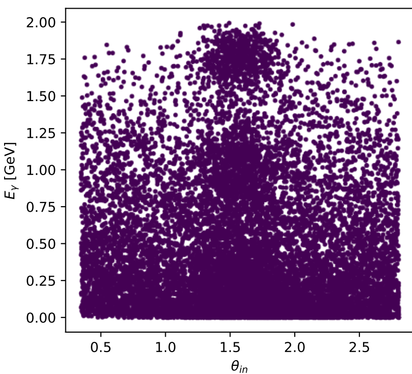
Phase-space scan: L electron [ L_{\text{electron}} ], max C_{e|p\gamma}=1.3657\text{e-}07
