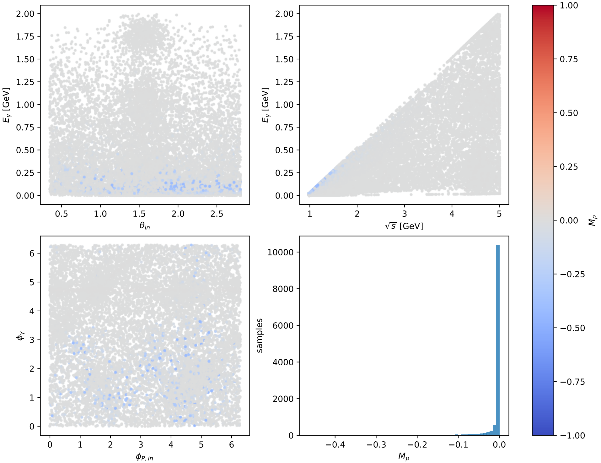
Phase-space scan: L electron [L_electron], max M_p=1.954\text{e-14}
