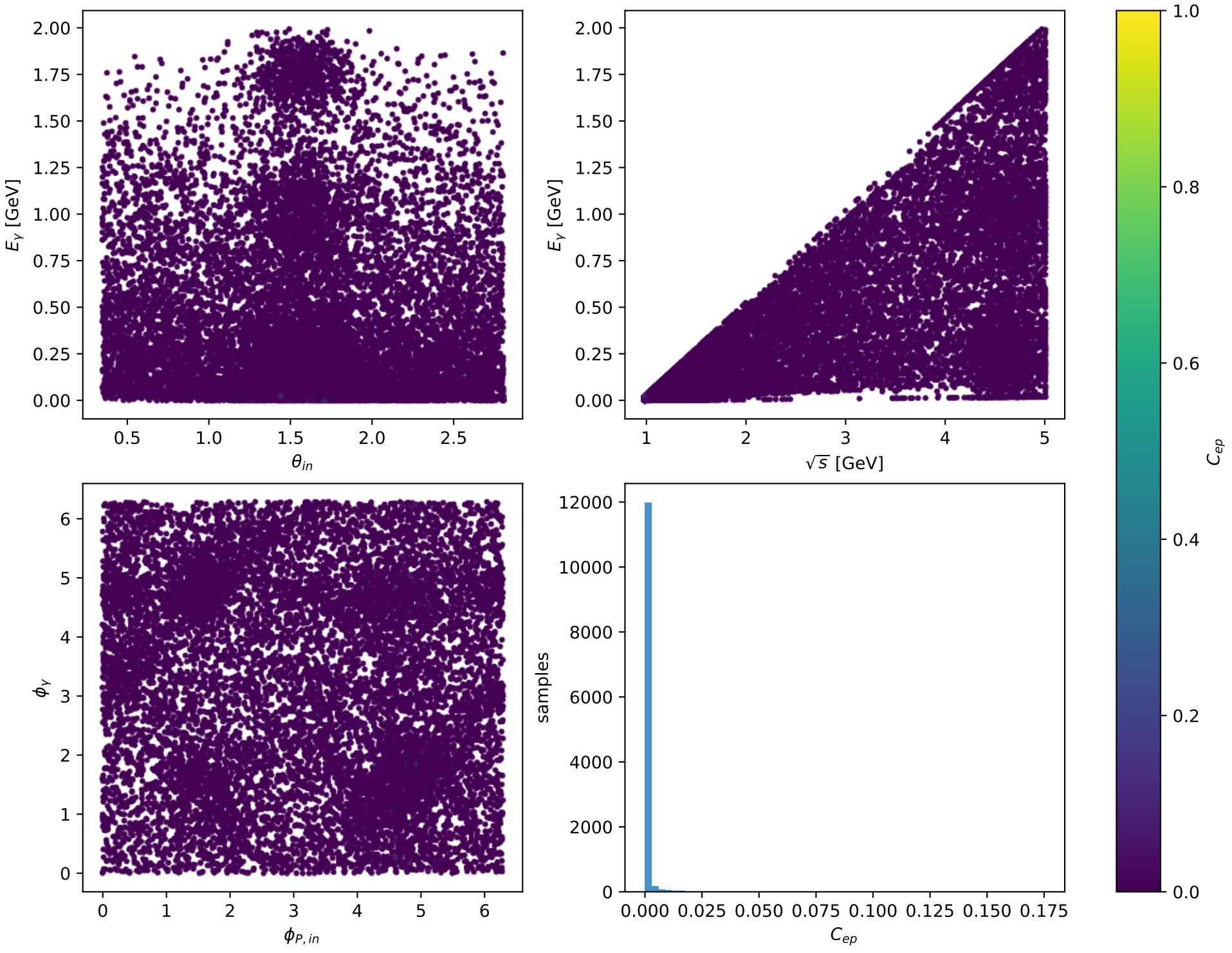
Phase-space scan: L electron [L electron ], max C_{ep} =0.17528
