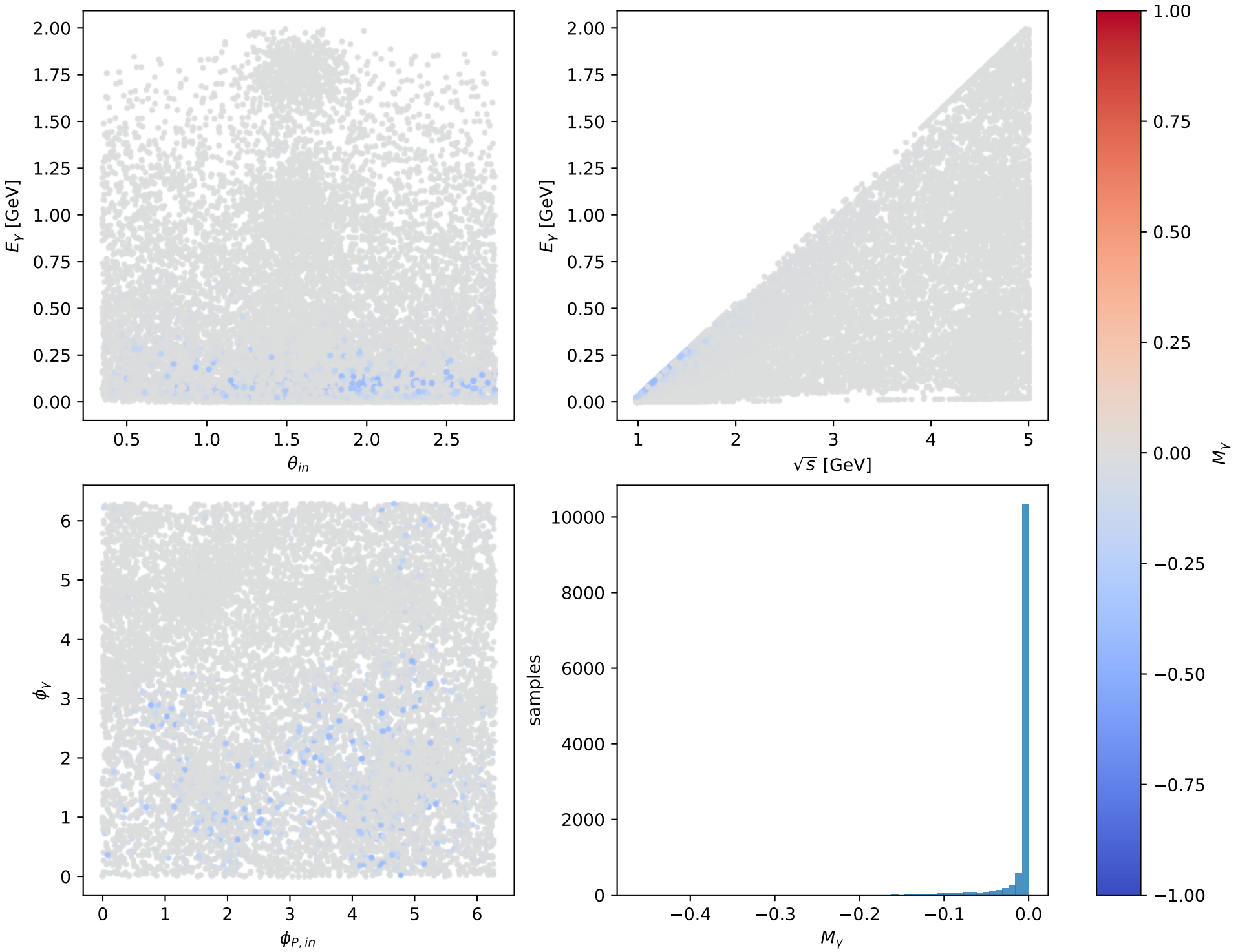
Phase-space scan: L electron [L_electron], max M_\gamma=1.8652\text{e-14}
