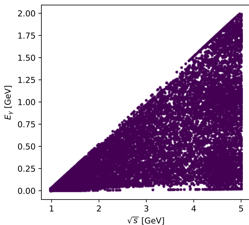
Phase-space scan: L electron [ L_{\text{electron}} ], max C_{e|p\gamma}=1.3657\text{e-}07
