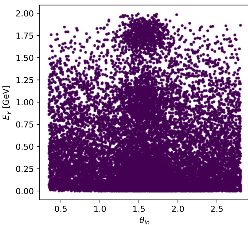
Phase-space scan: L electron [ L_{\text{electron}} ], max C_{\gamma|ep}=1.3657\text{e-}07
