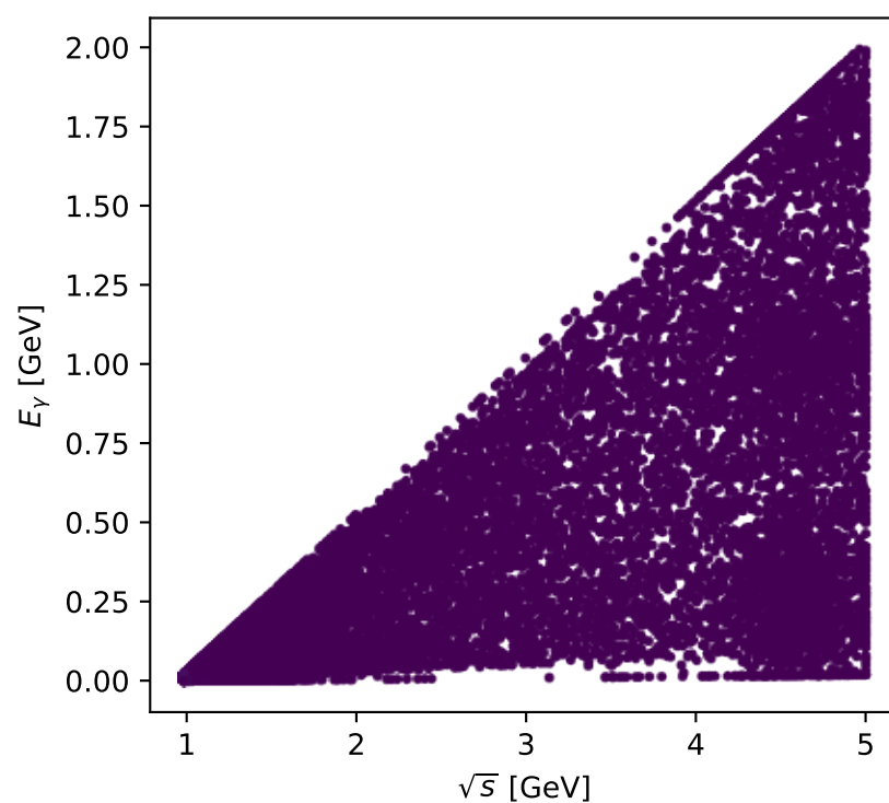
Phase-space scan: Tx electron [Tx_electron], max C_{ep}=0.18306
