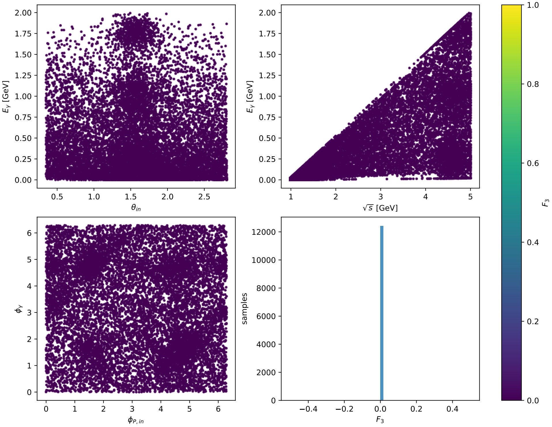
Phase-space scan: Tx electron [Tx_electron], max F_3=0
