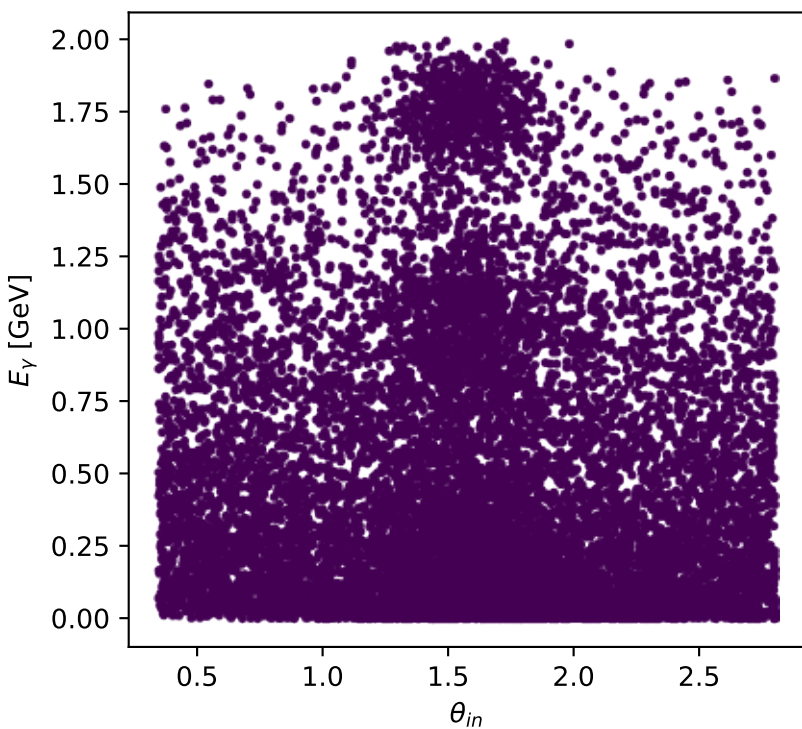
Phase-space scan: Tx electron [Tx_electron], max C_{p\gamma}=0.034289
