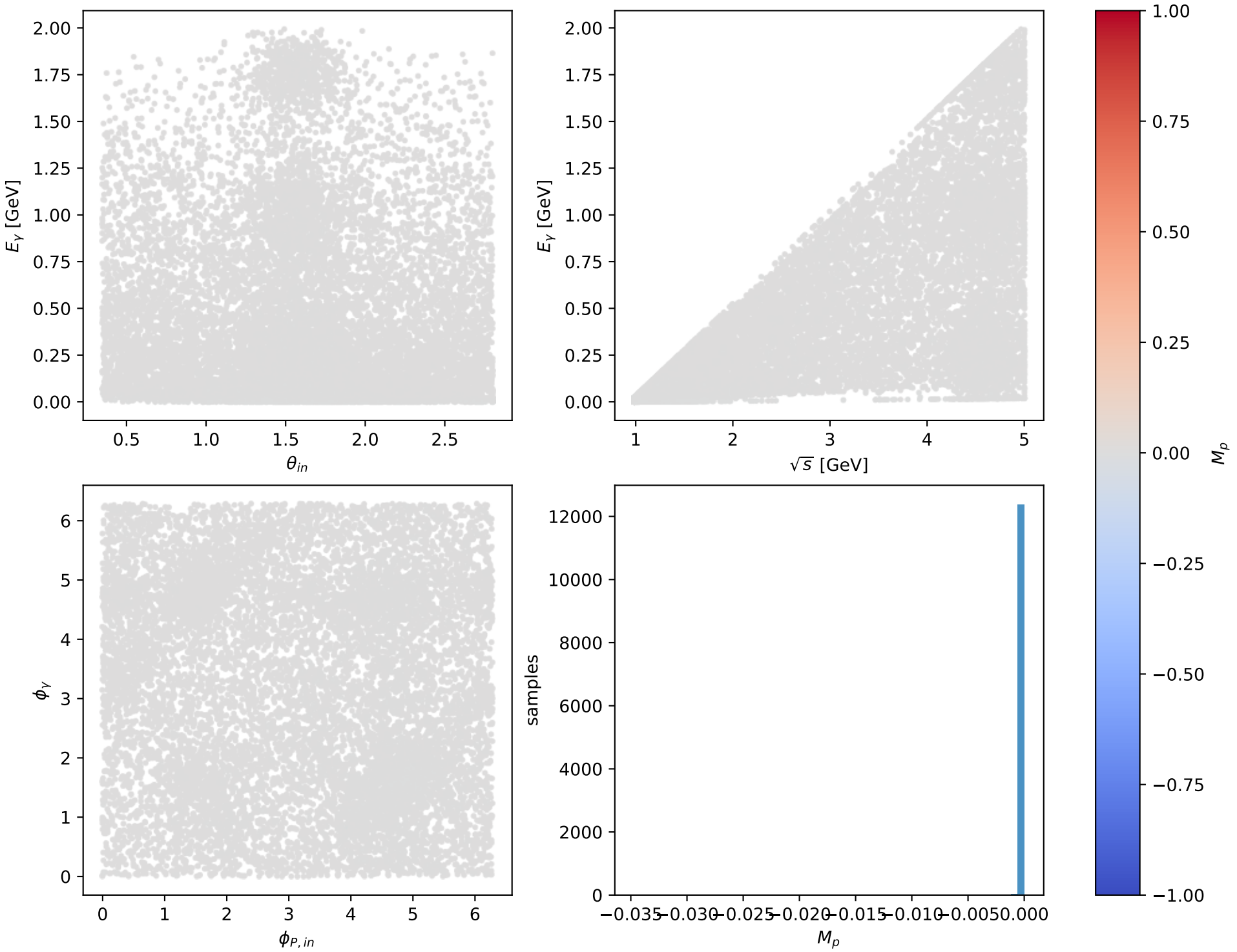
Phase-space scan: Tx electron [Tx_electron], max M_p=-0
