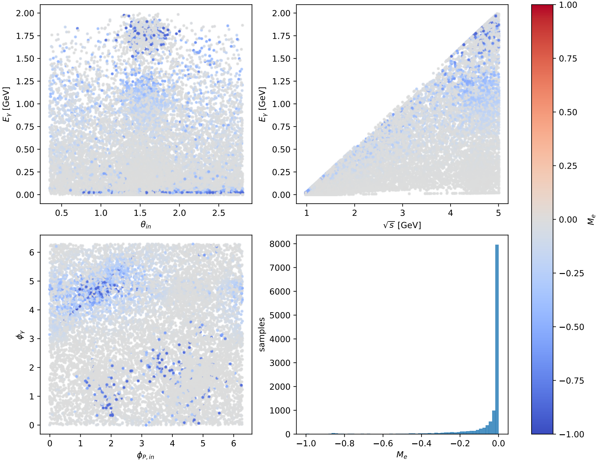
Phase-space scan: Tx electron [Tx_electron], max M_e = -0
