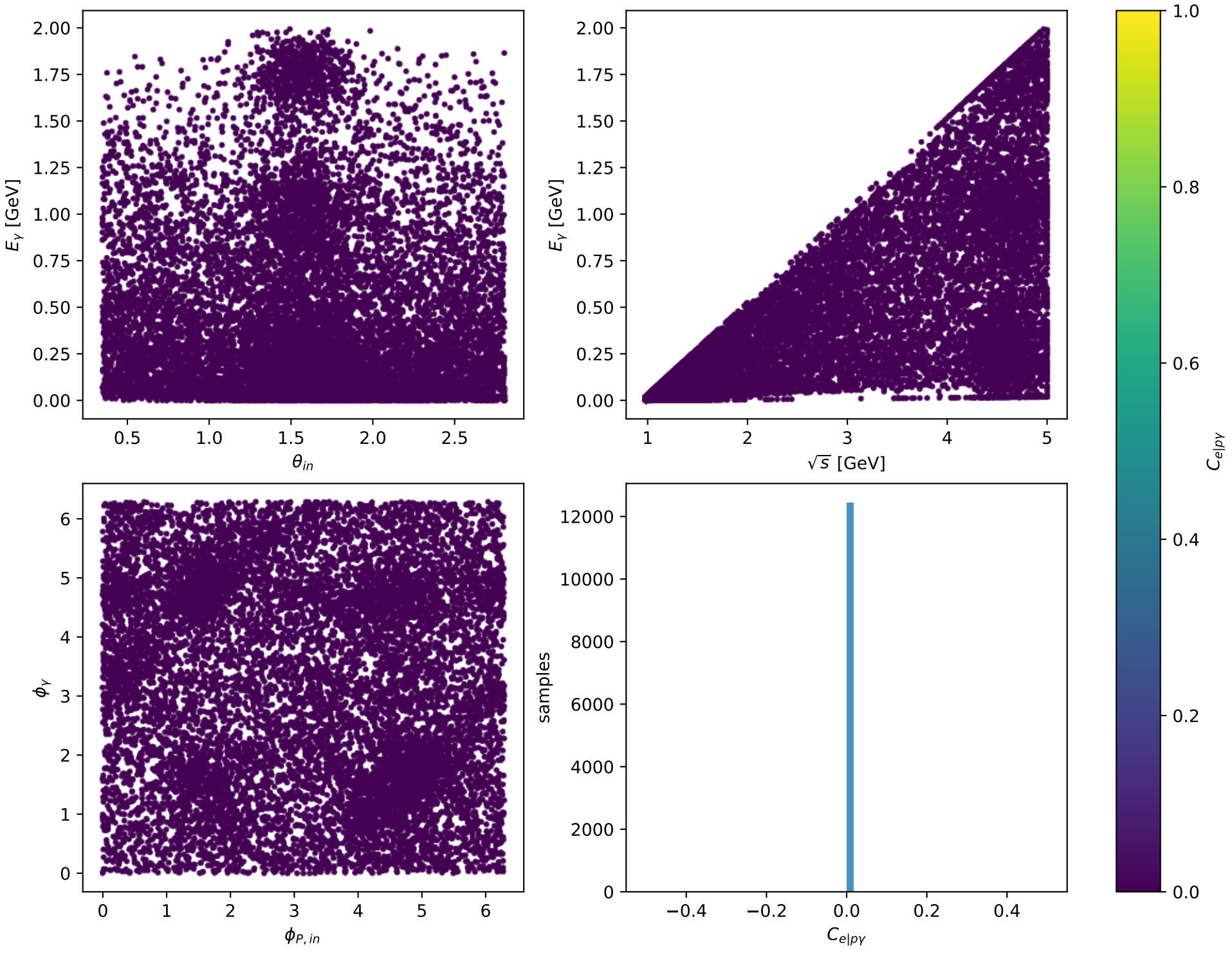
Phase-space scan: Tx electron [Tx_electron], max C_{e|p\gamma}=0
