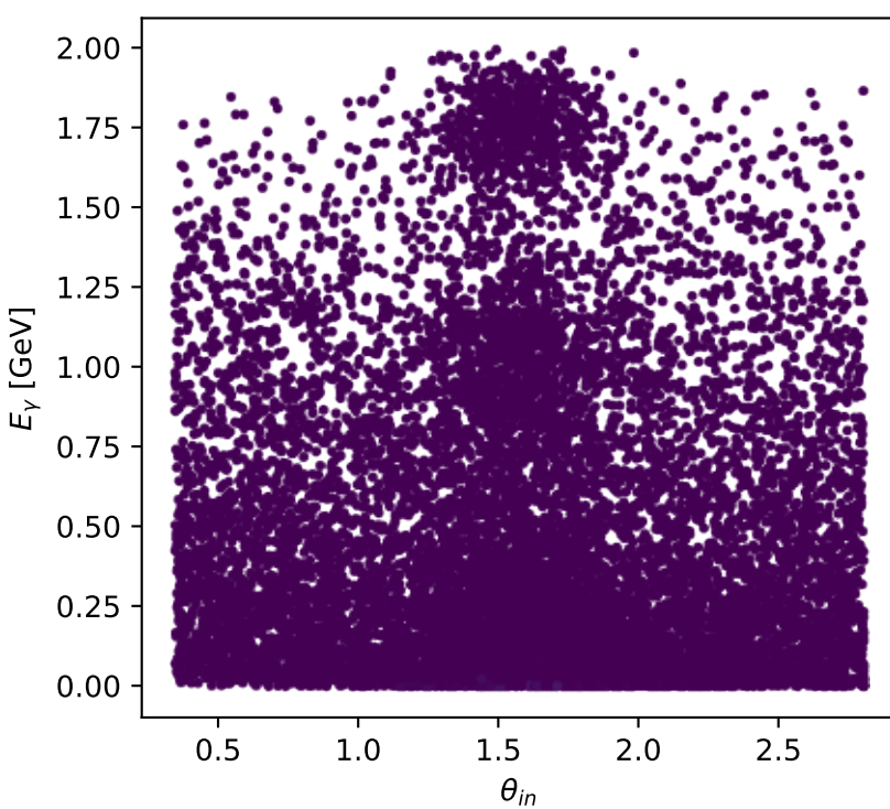
Phase-space scan: Tx electron [Tx_electron], max C_{ep}=0.18306
