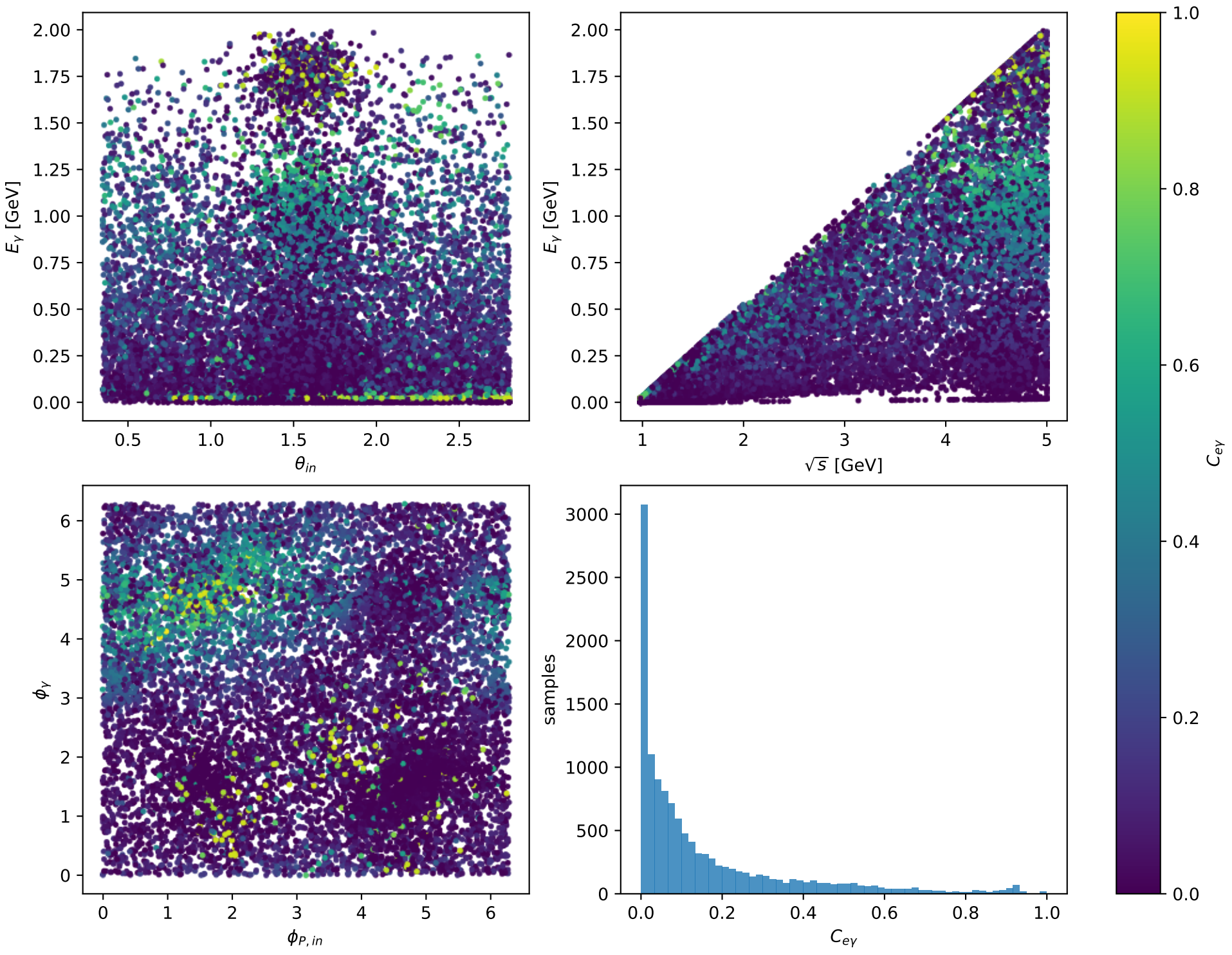
Phase-space scan: Tx electron [Tx_electron], max C_{ey}=0.99998
