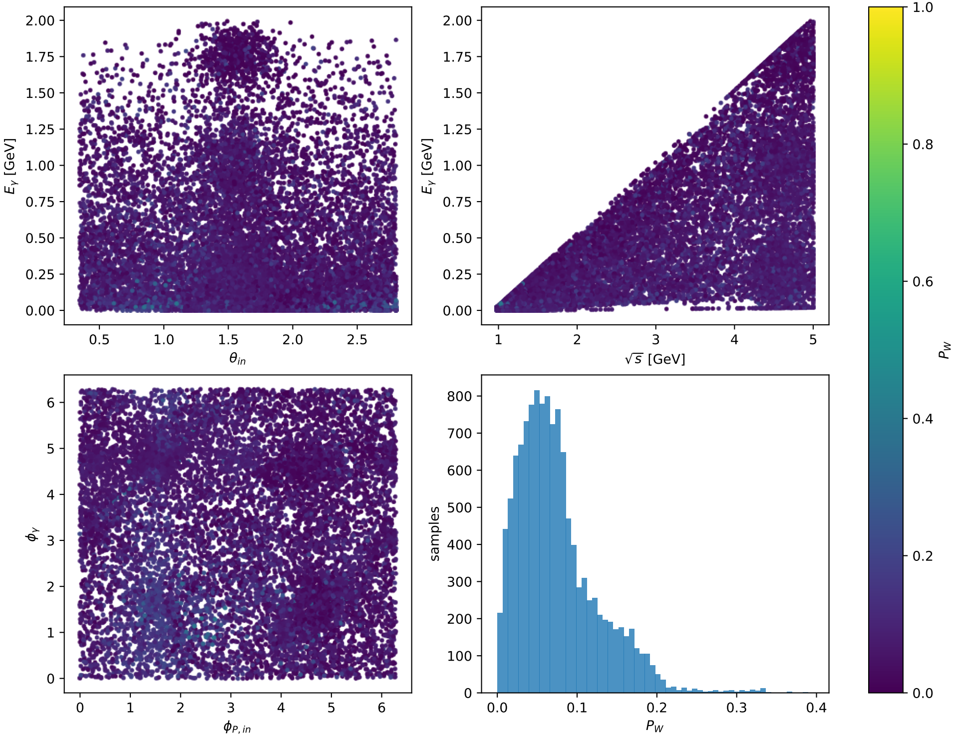
Phase-space scan: Tx electron [Tx_electron], max P_W=0.39586
