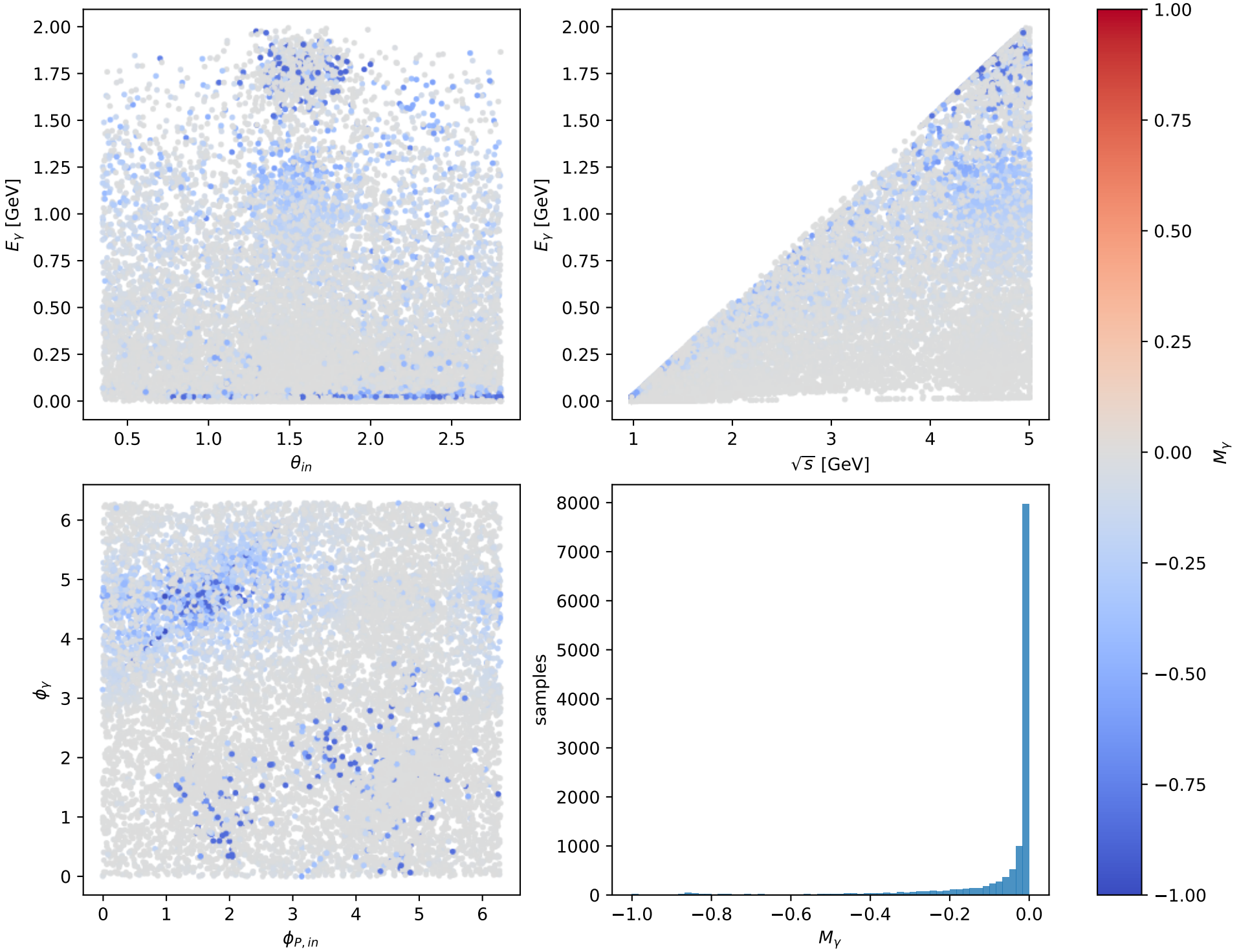
Phase-space scan: Tx electron [Tx_electron], max M_Y=-0
