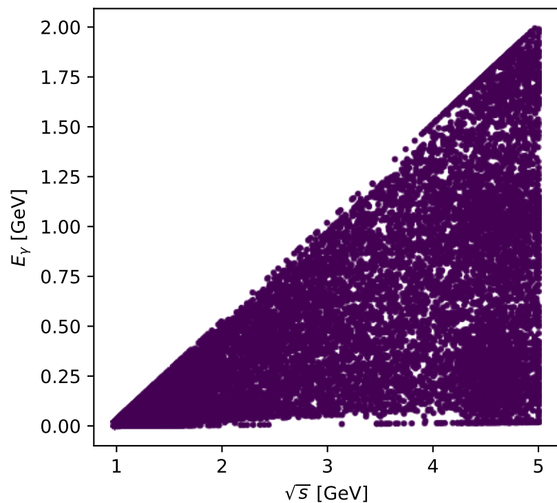
Phase-space scan: Tx electron [Tx_electron], max C_{p\gamma}=0.034289
