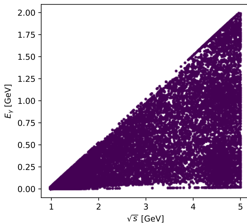
Phase-space scan: Tx electron [Tx_electron], max C_{p|e\gamma}=0
