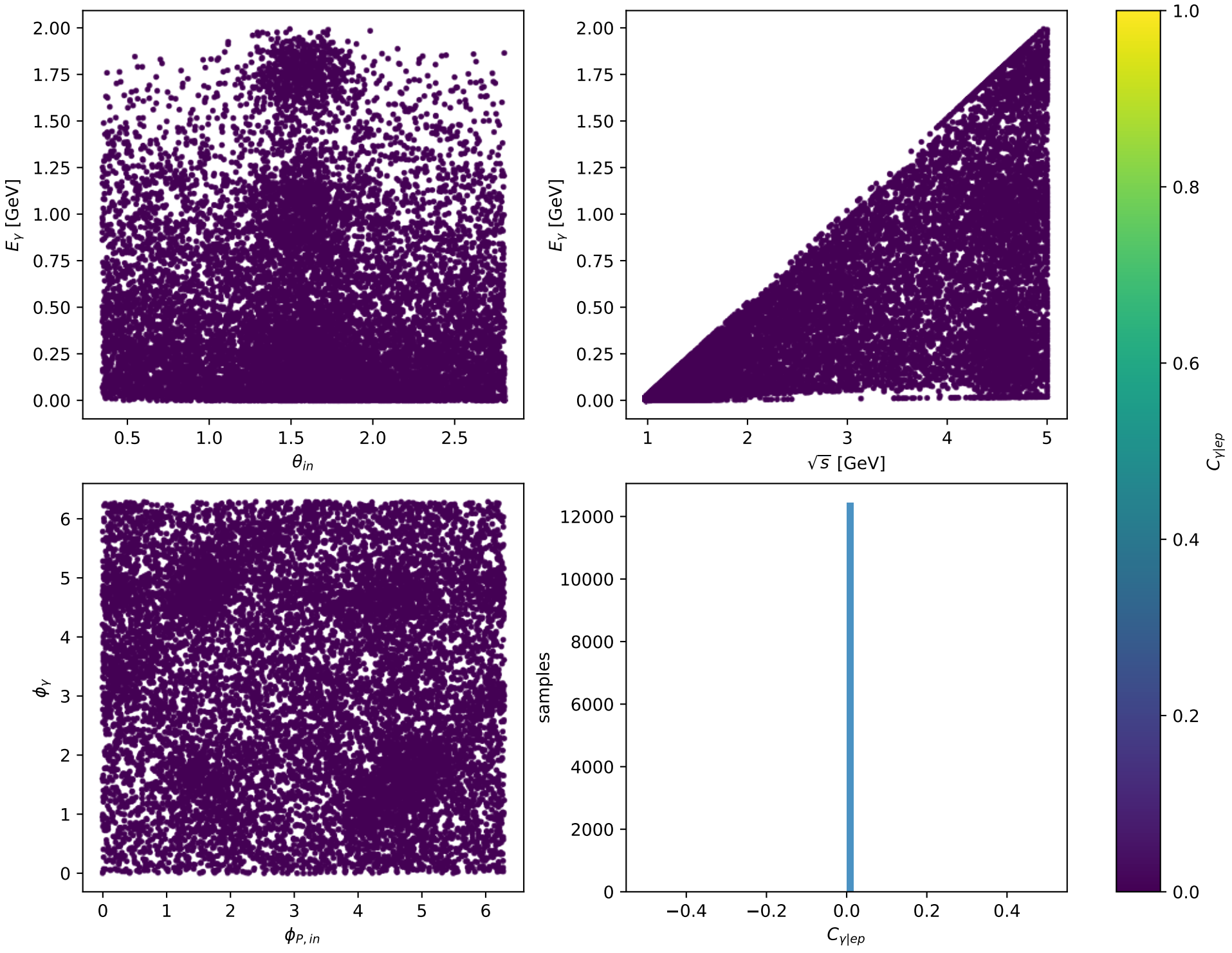
Phase-space scan: Ty electron [Ty_electron], max C_{\gamma|ep}=0
