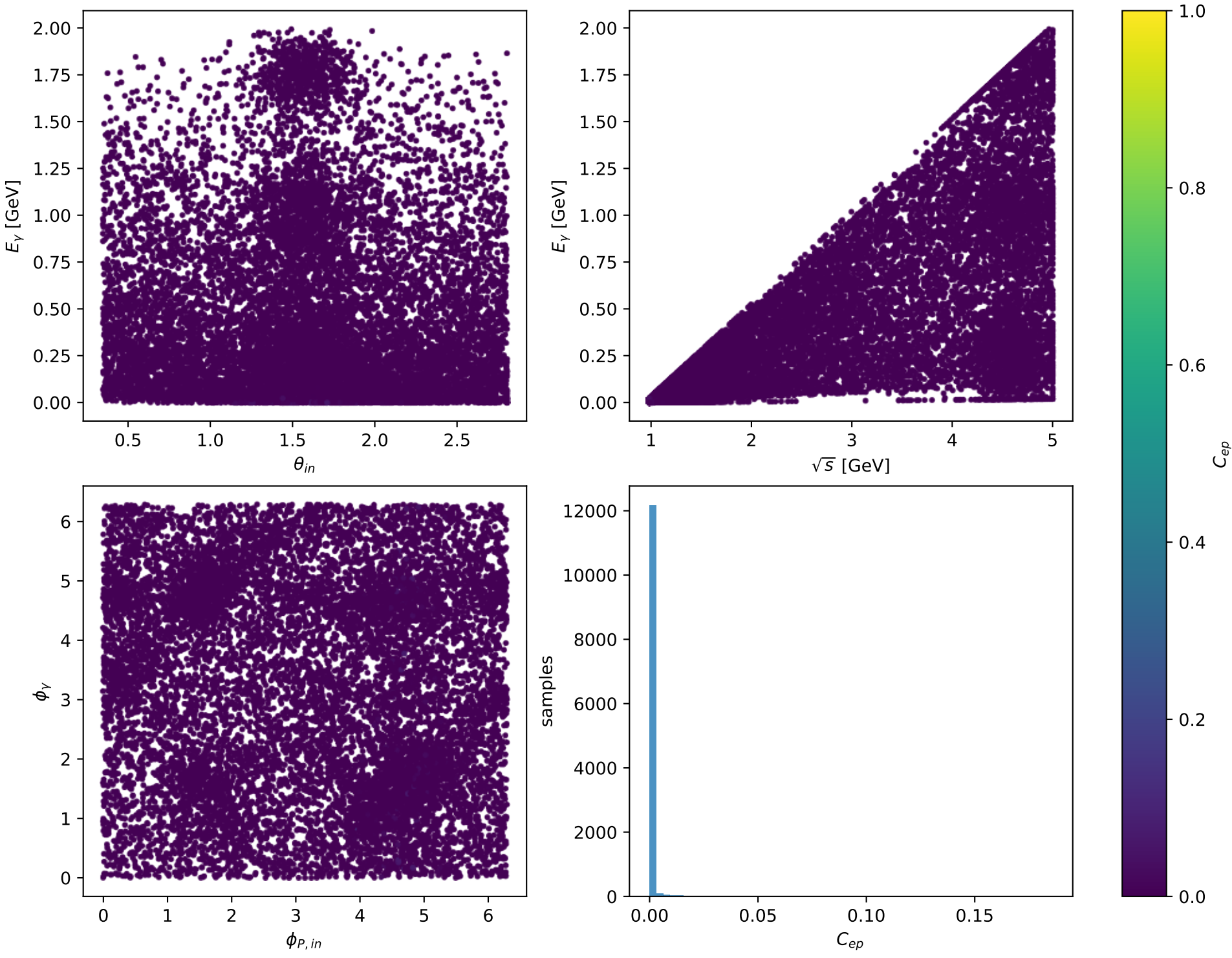
Phase-space scan: Ty electron [Ty_electron], max C_{ep}=0.18592
