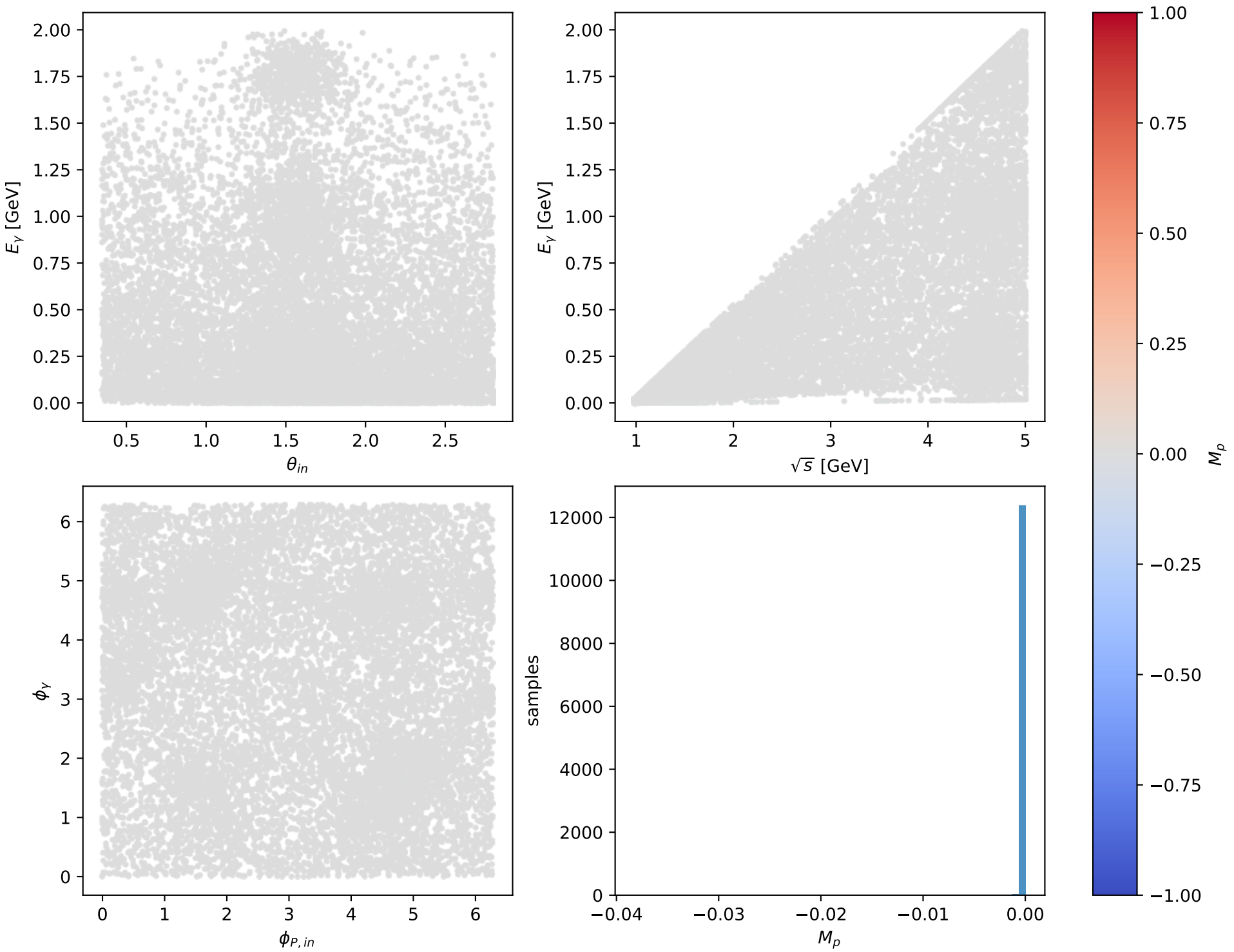
Phase-space scan: Ty electron [Ty_electron], max M_p=-0
