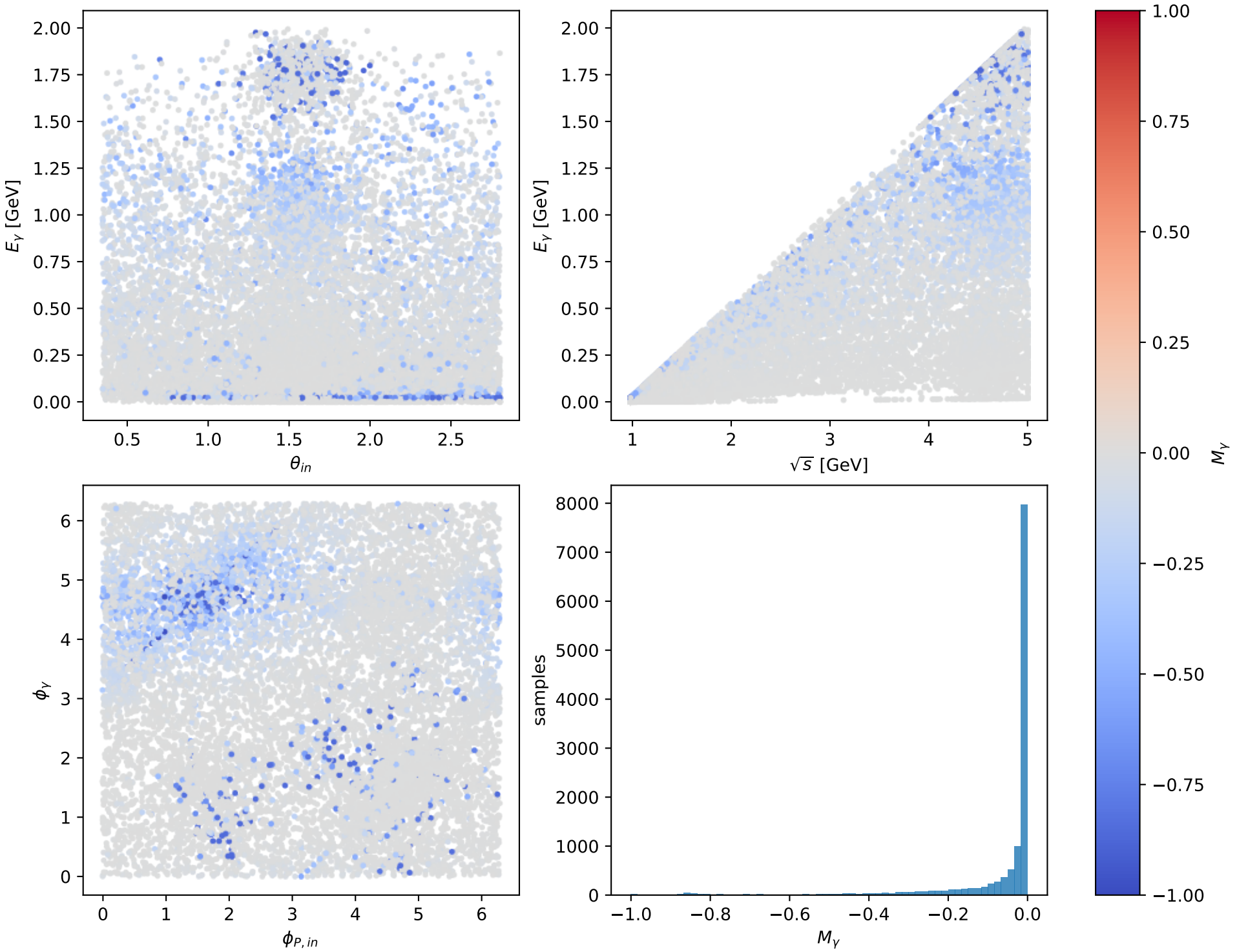
Phase-space scan: Ty electron [Ty_electron], max M_Y=-0
