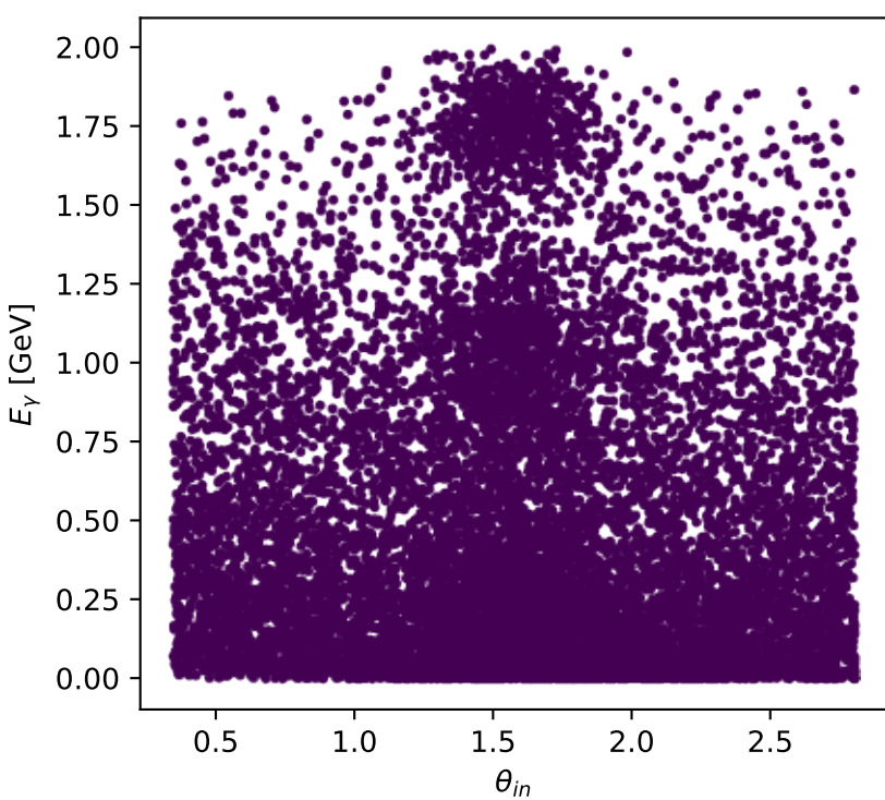
Phase-space scan: Ty electron [Ty_electron], max C_{e|p\gamma}=0
