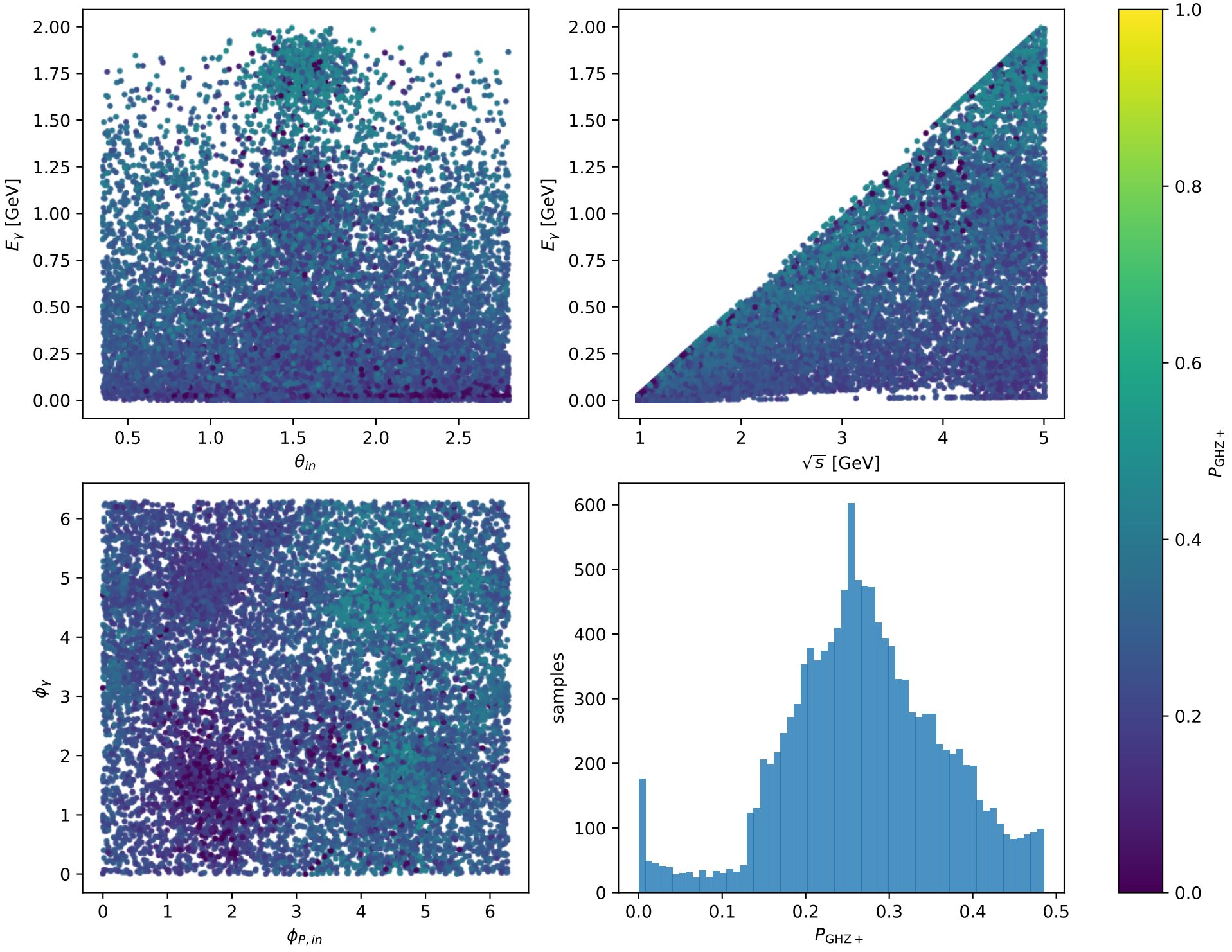
Phase-space scan: Ty electron [Ty_electron], max P_{\text{GHZ}+}=0.48525
