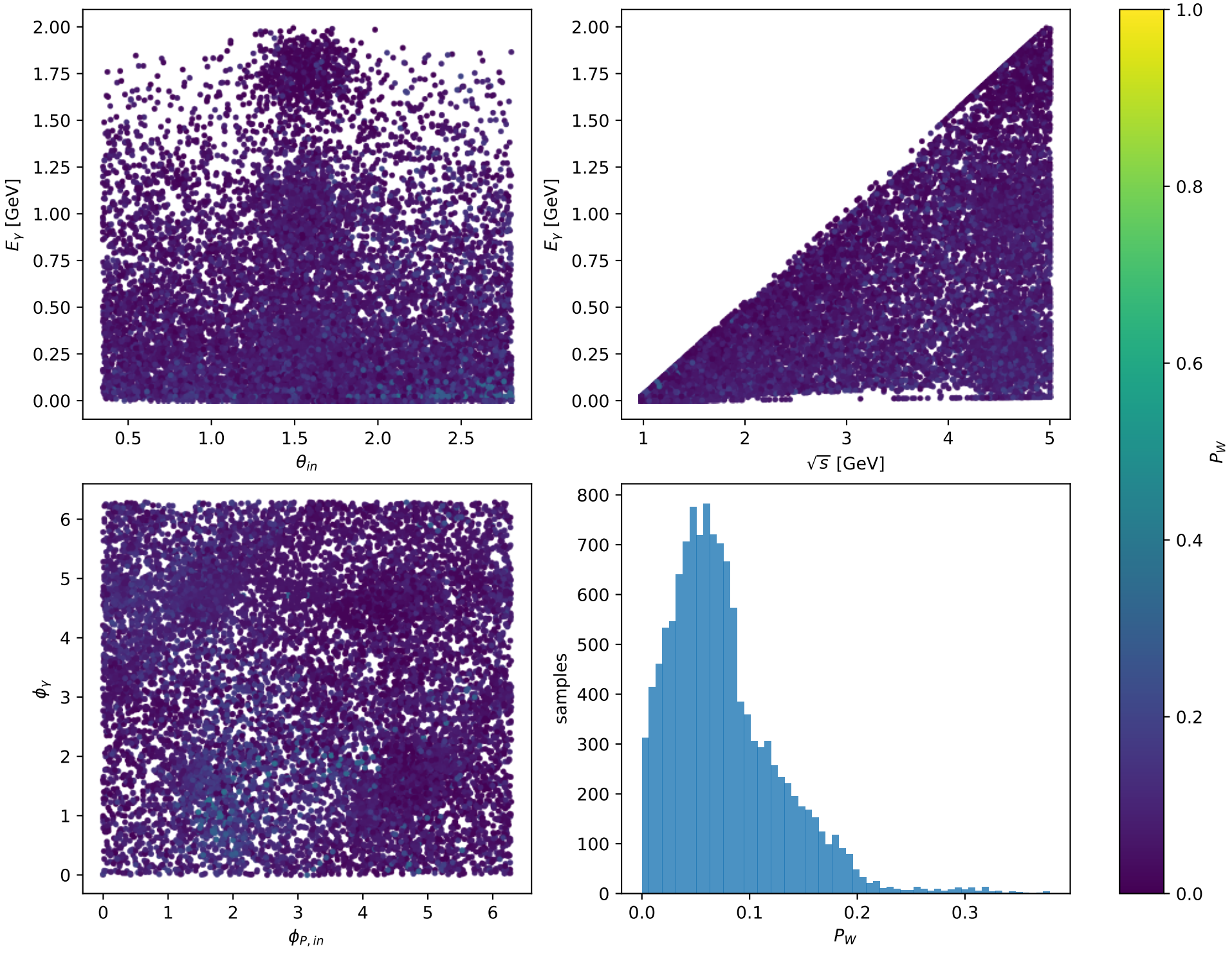
Phase-space scan: Ty electron [Ty_electron], max P_W=0.37879
