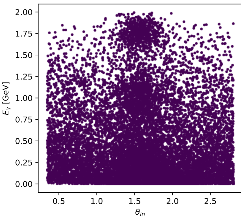
Phase-space scan: Ty electron [Ty_electron], max F_3=0
