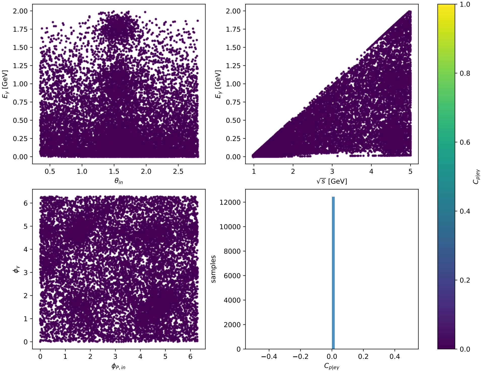
Phase-space scan: Ty electron [Ty_electron], max C_{p|e\gamma}=0
