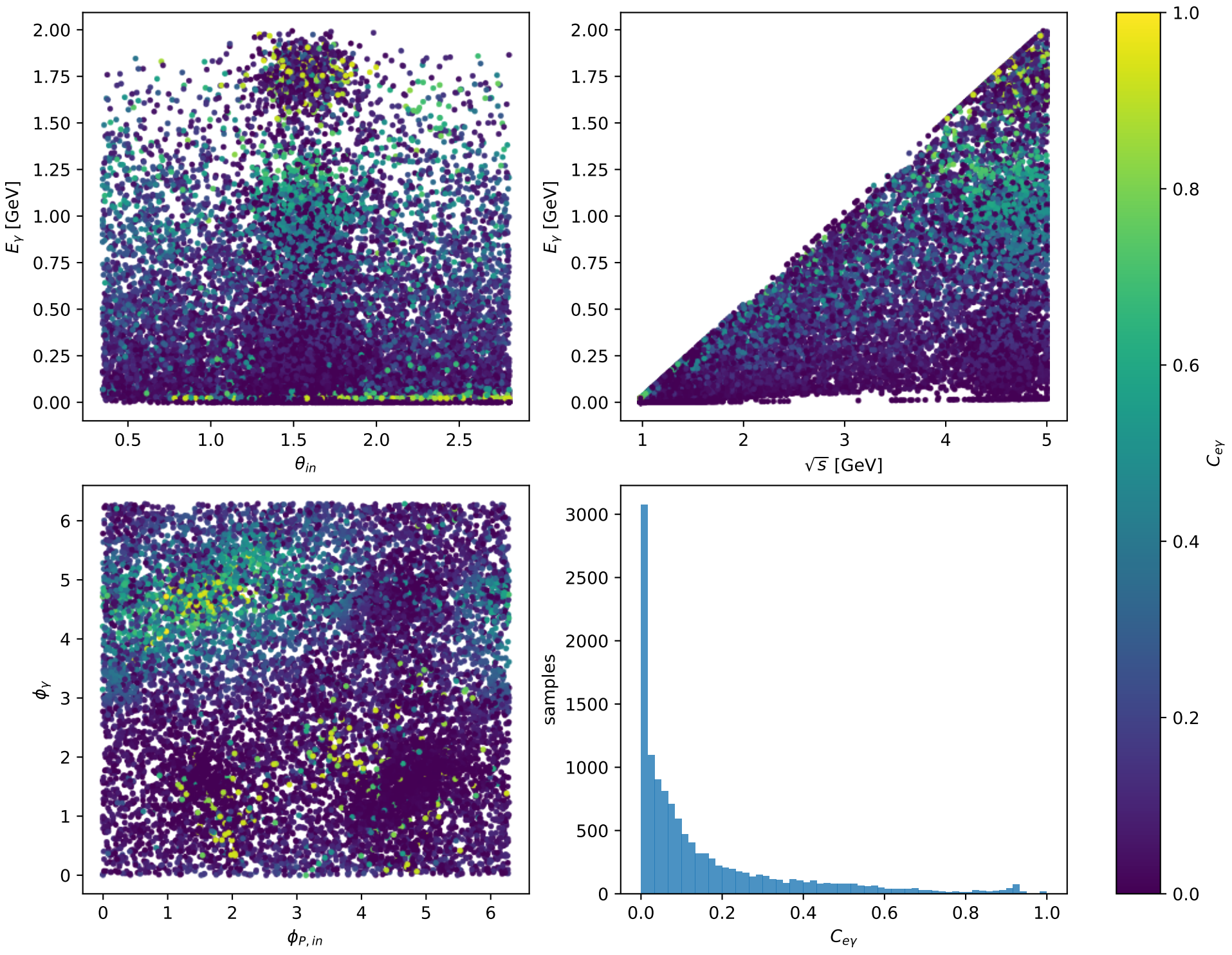
Phase-space scan: Ty electron [Ty_electron], max C_{ey}=0.99998
