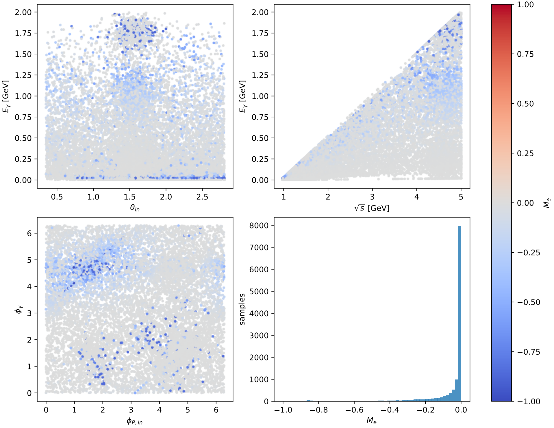
Phase-space scan: Ty electron [Ty_electron], max M_e = -0
