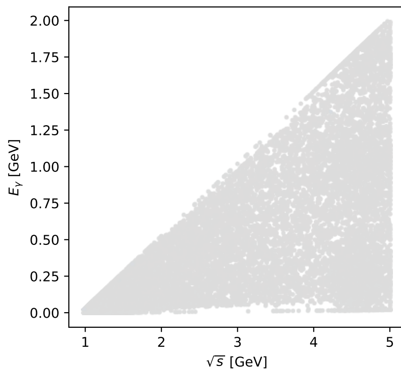
Phase-space scan: L proton [L_proton], max M_e=9.8586\text{e-14}
