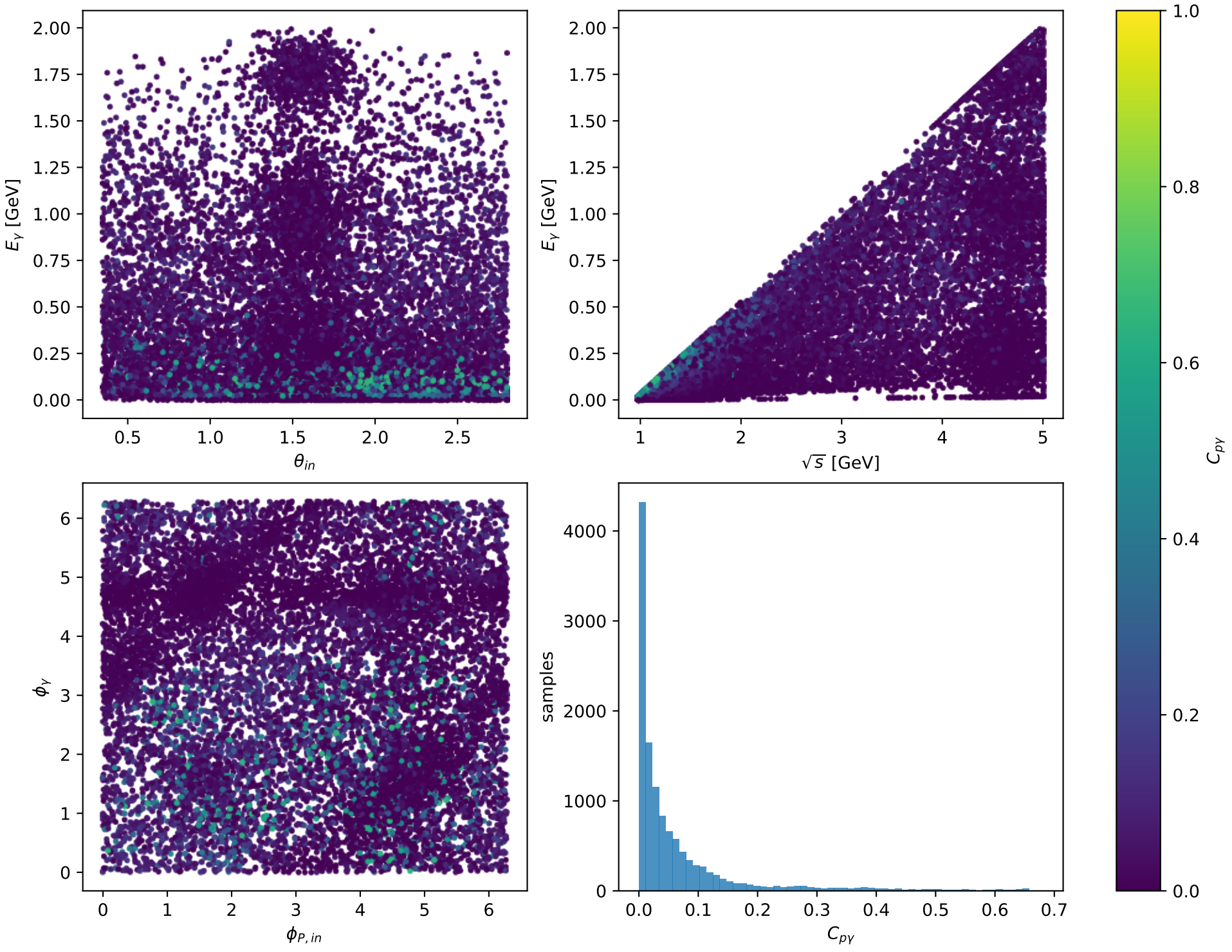
Phase-space scan: L proton [L_proton], max C_{p\gamma}=0.68084
