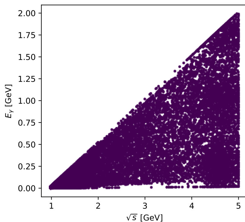
Phase-space scan: L proton [ L_{\text{proton}} ], max C_{\gamma|ep}=3.437\text{e-}07
