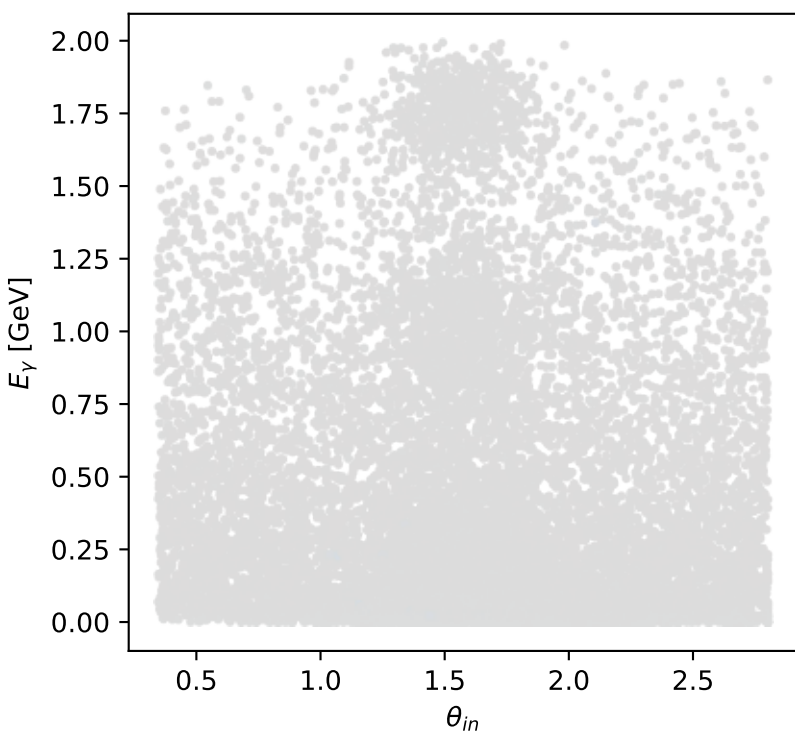
Phase-space scan: L proton [L_proton], max M_e=9.8586\text{e-14}
