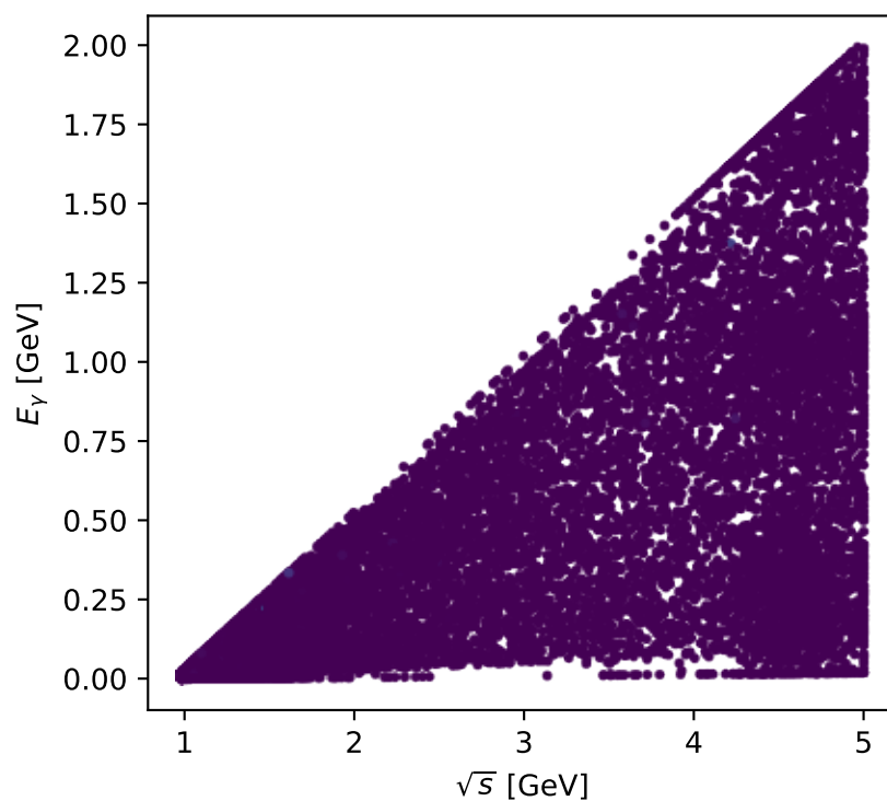
Phase-space scan: L proton [L_proton], max C_{ey}=0.30396
