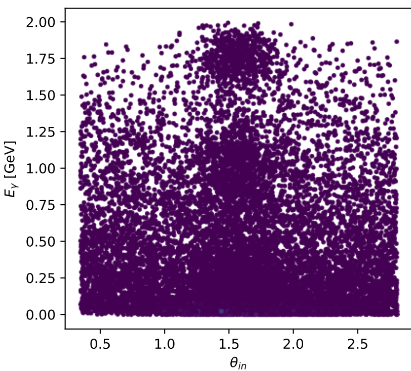
Phase-space scan: L proton [L_proton], max C_{ep}=0.21918
