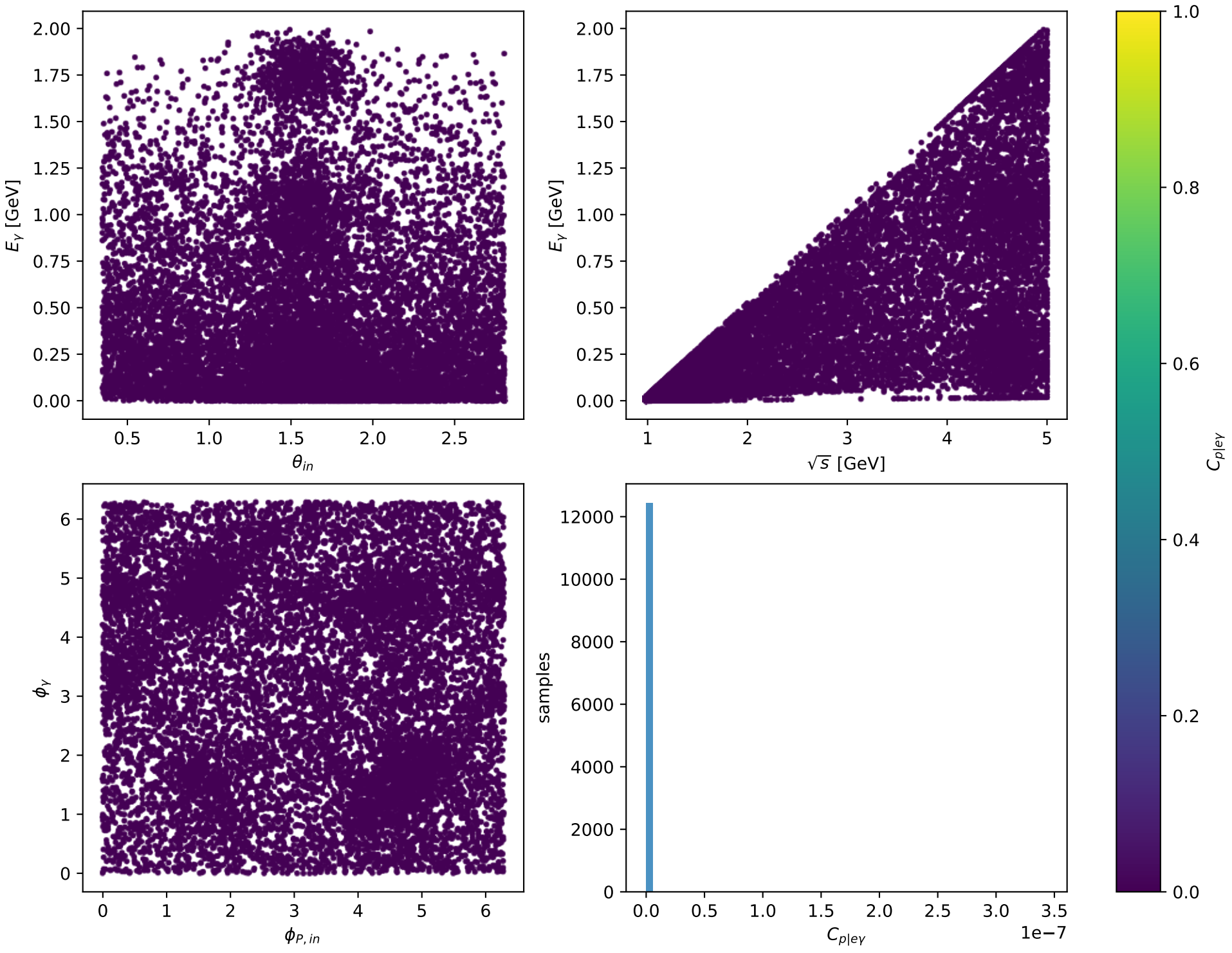
Phase-space scan: L proton [ L_{\text{proton}} ], max C_{p|e\gamma}=3.437\text{e-}07
