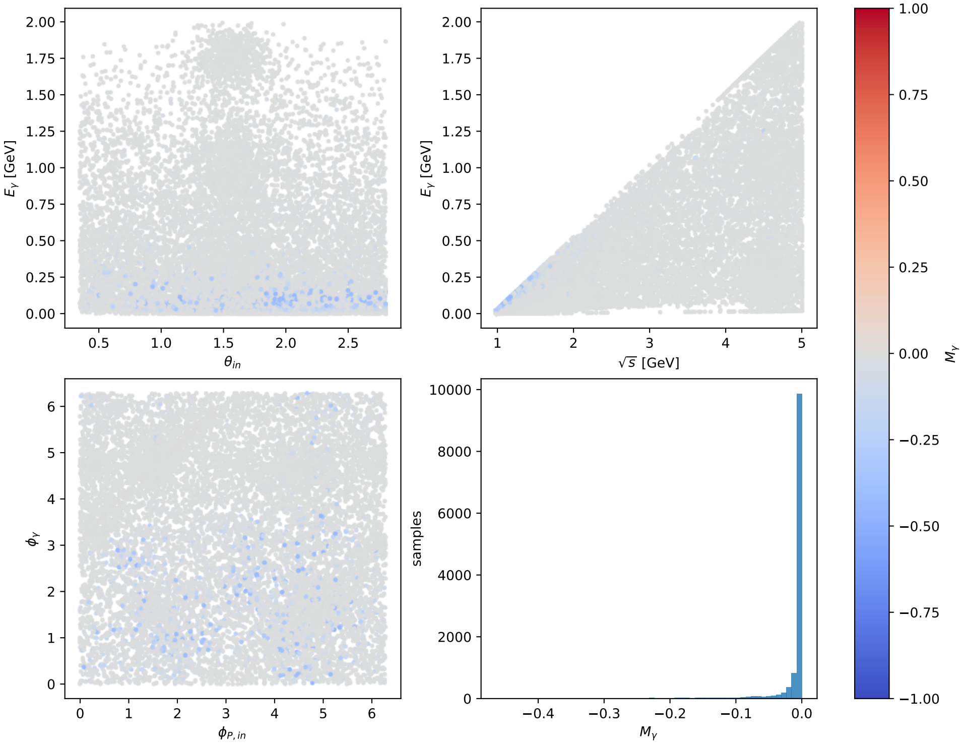
Phase-space scan: L proton [L_proton], max M_\gamma=1.1813\text{e-}13
