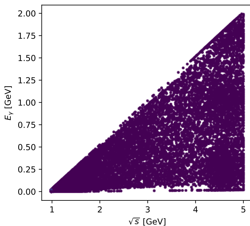
Phase-space scan: L proton [L_proton], max C_{ep}=0.21918
