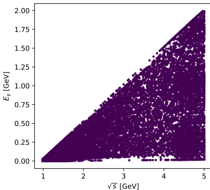
Phase-space scan: L proton [L_proton], max F_3=1.1067\text{e-13}
