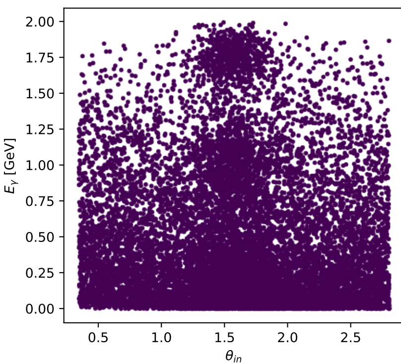
Phase-space scan: L proton [ L_{\text{proton}} ], max C_{\gamma|ep}=3.437\text{e-}07
