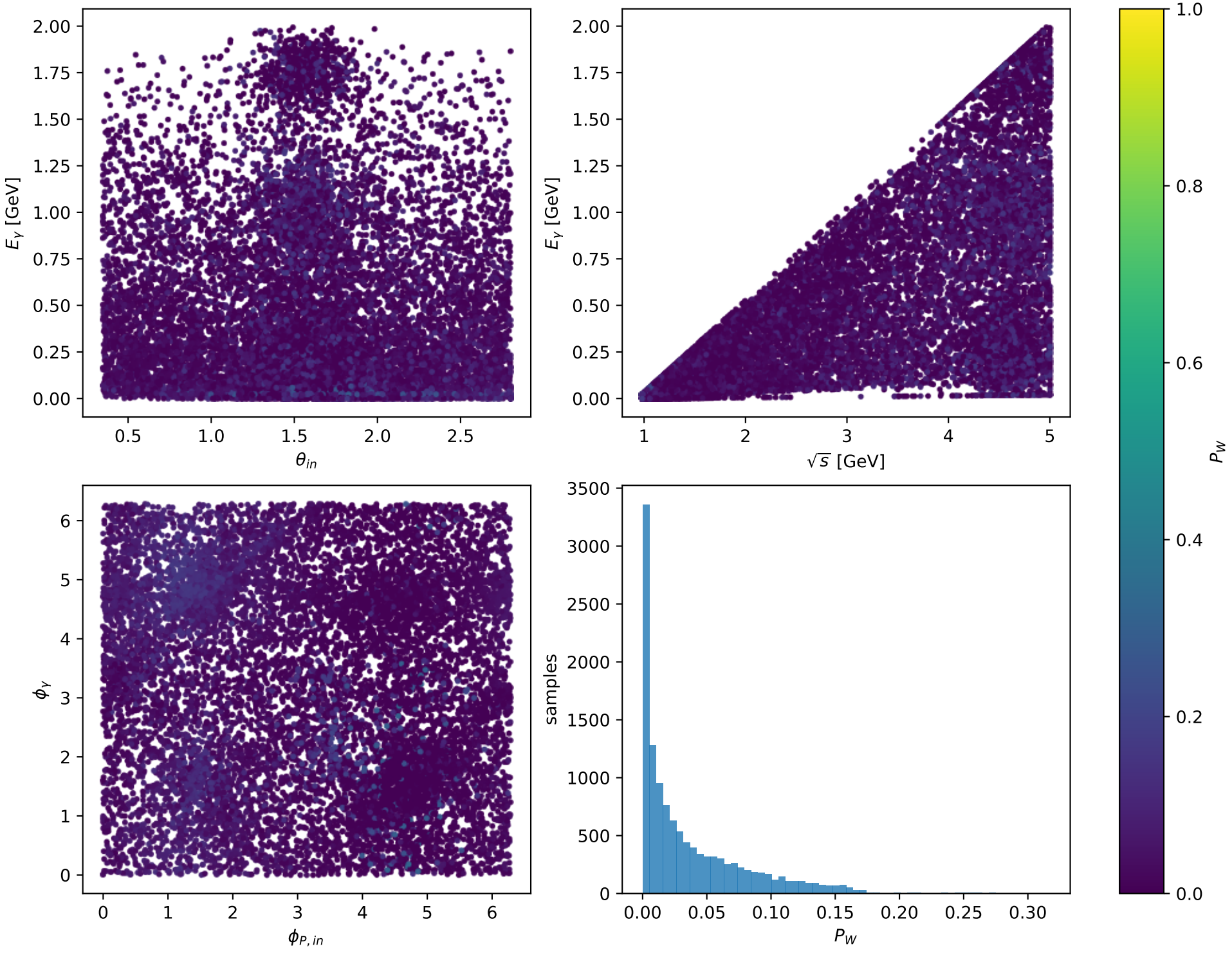
Phase-space scan: L proton [L_proton], max P_W=0.31713
