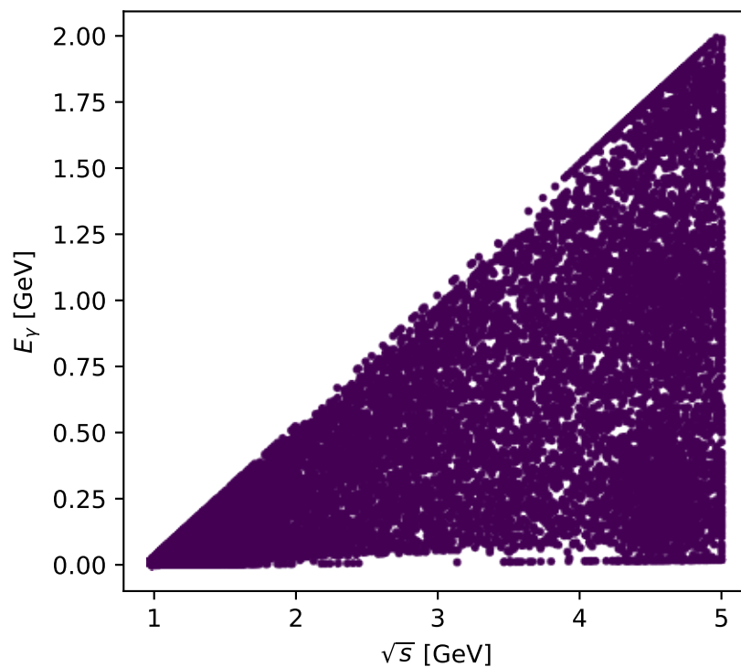
Phase-space scan: Tx proton [Tx_proton], max C_{\gamma|ep}=0
