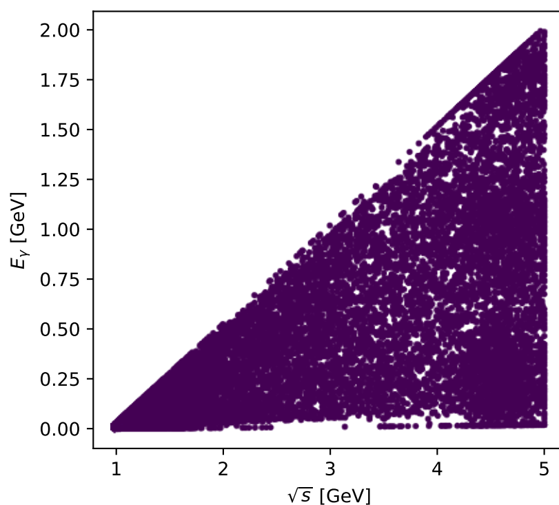
Phase-space scan: Tx proton [Tx_proton], max C_{ey}=0.12179
