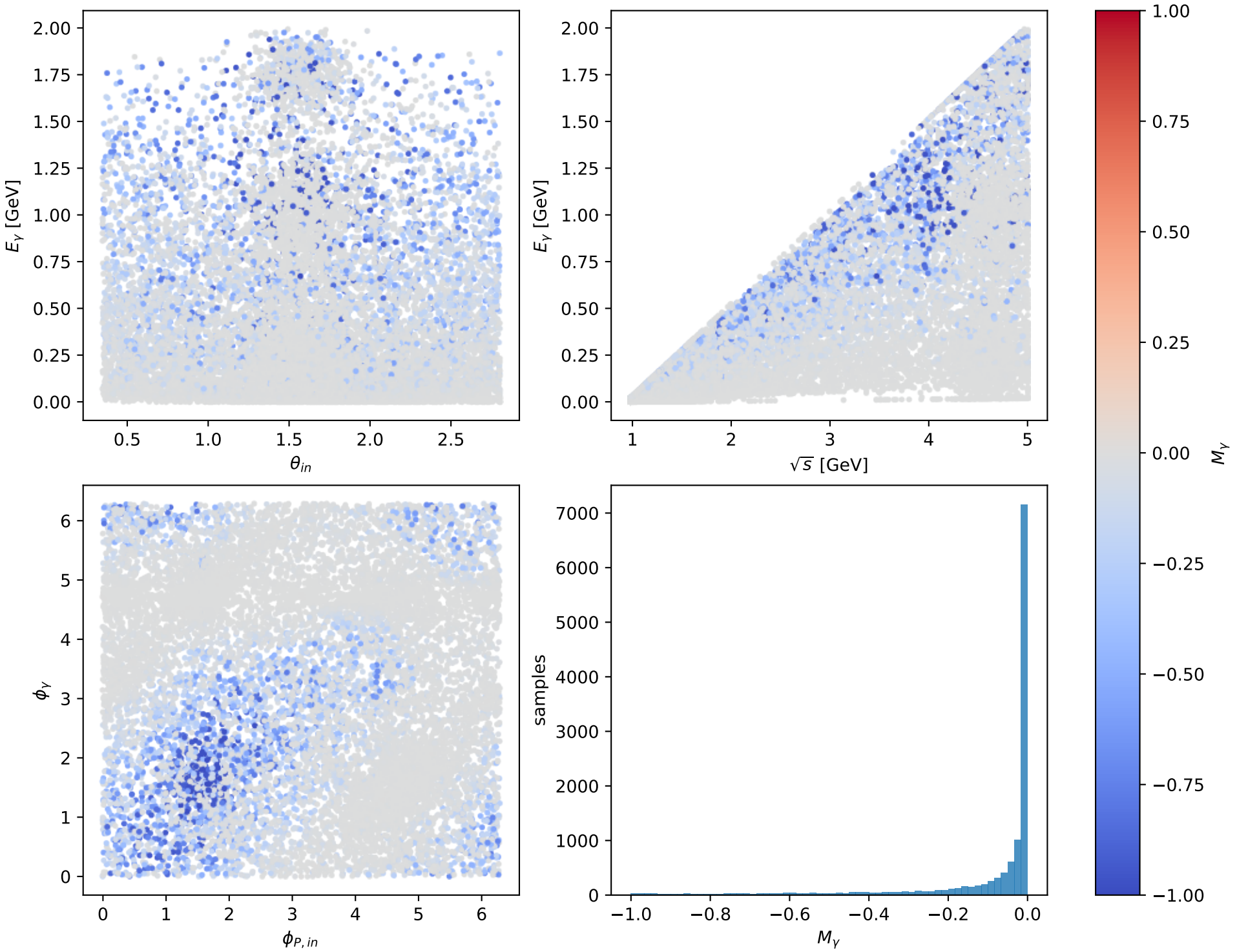
Phase-space scan: Tx proton [Tx_proton], max M_Y = -0
