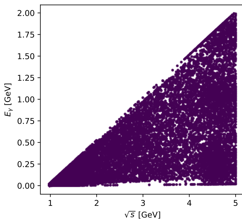
Phase-space scan: Tx proton [Tx_proton], max C_{p|e\gamma}=0
