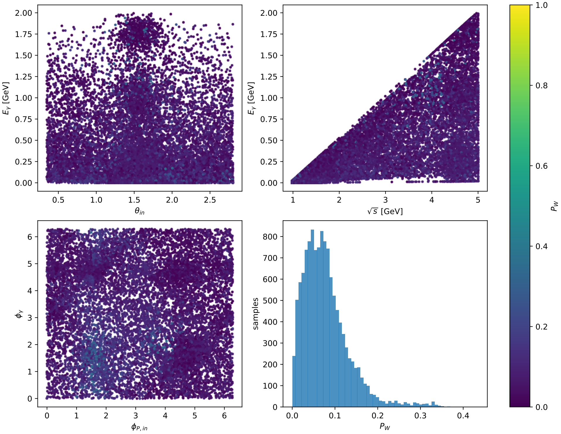
Phase-space scan: Tx proton [Tx_proton], max P_W=0.43477
