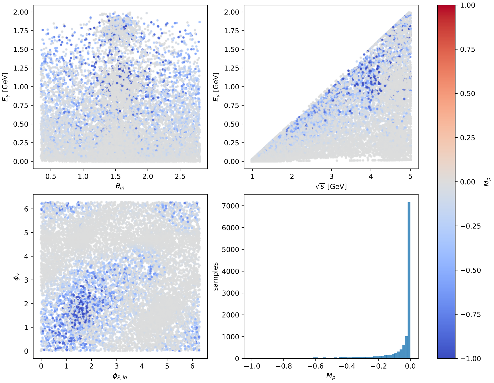
Phase-space scan: Tx proton [Tx_proton], max M_p = -0
