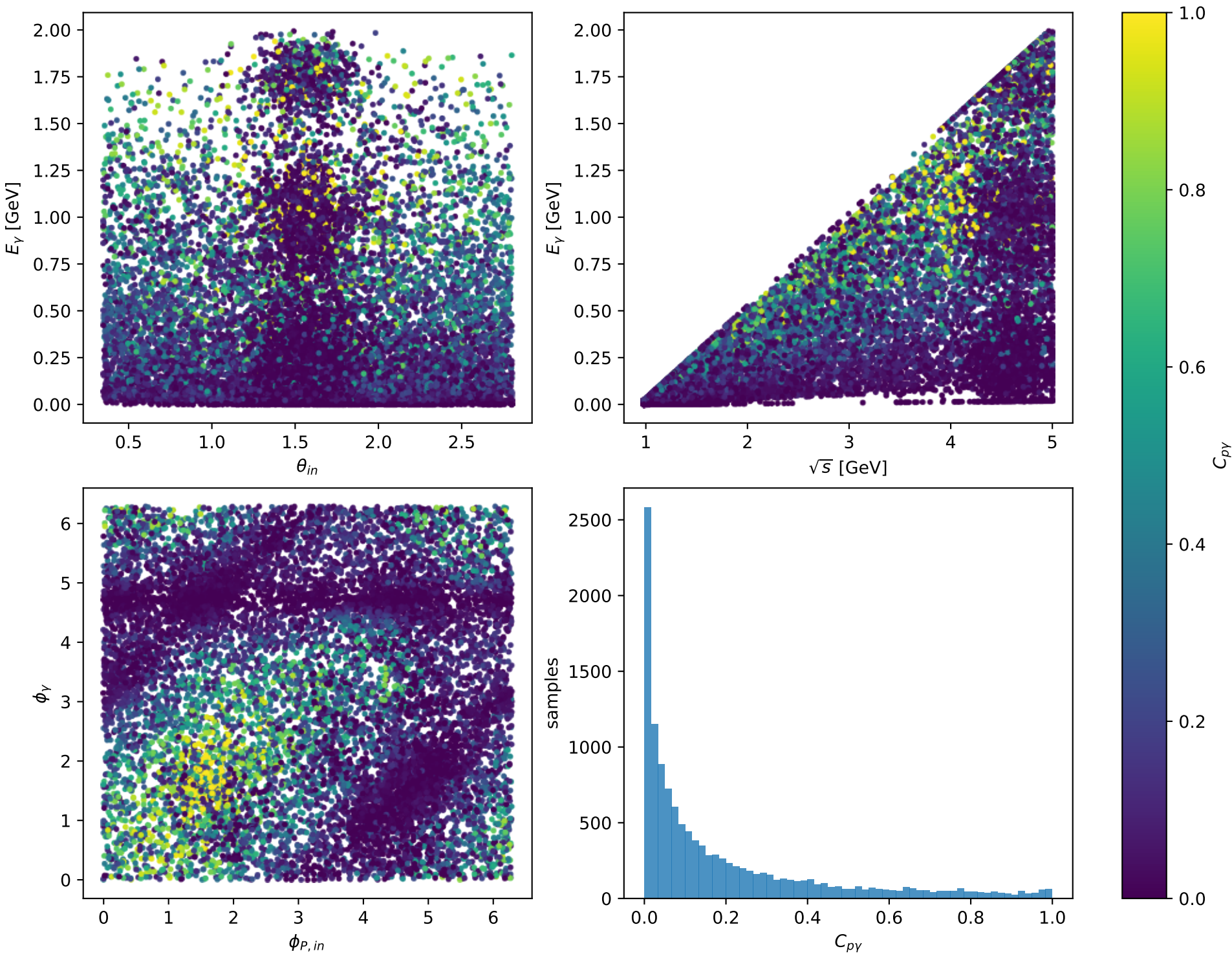
Phase-space scan: Tx proton [Tx_proton], max C_{p\gamma}=0.99999
