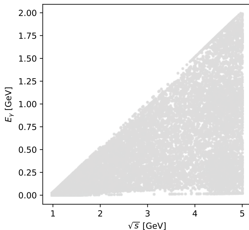
Phase-space scan: Tx proton [Tx_proton], max M_e = -0
