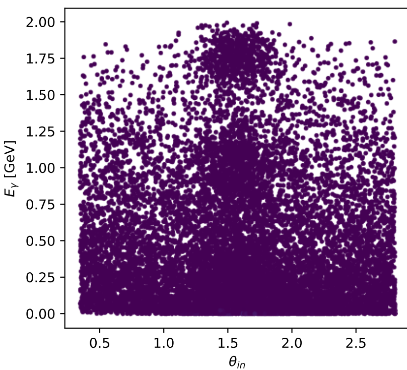
Phase-space scan: Tx proton [Tx_proton], max C_{ep}=0.17813
