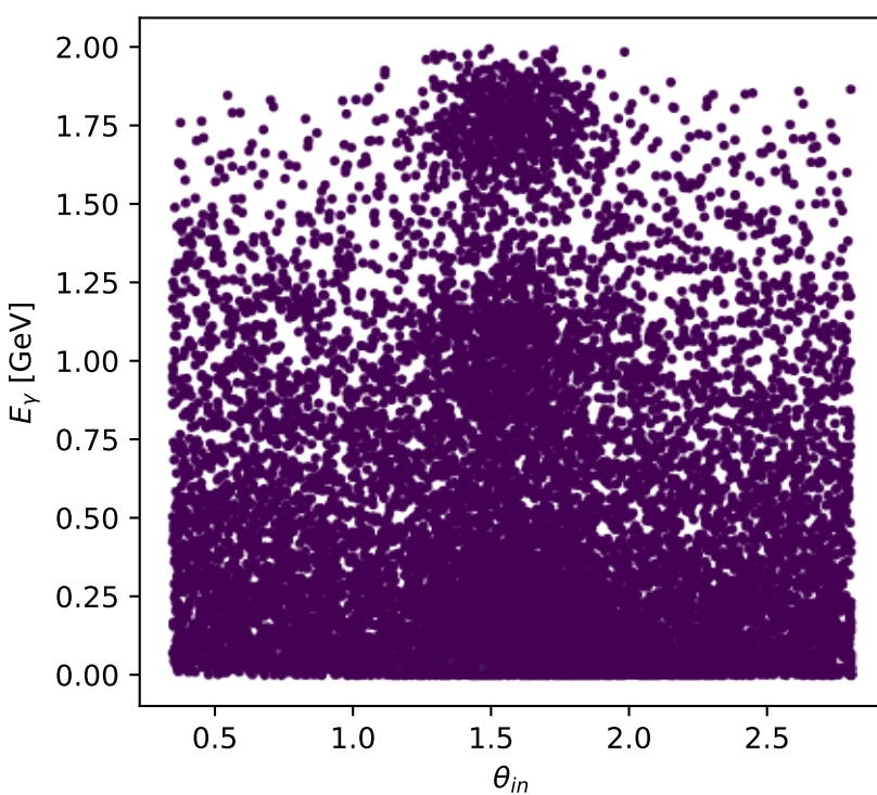
Phase-space scan: Tx proton [Tx_proton], max C_{ey}=0.12179
