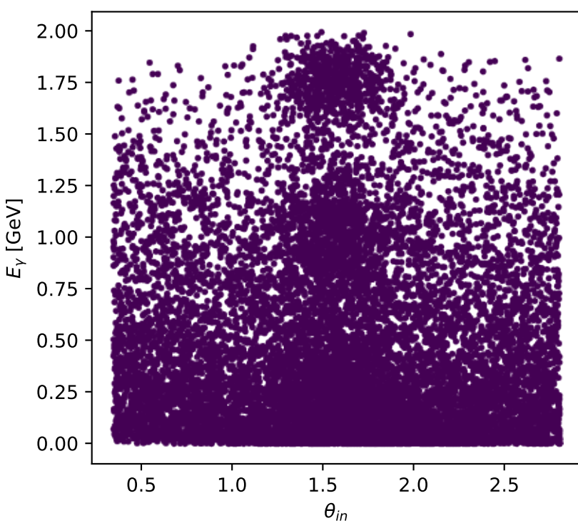
Phase-space scan: Tx proton [Tx_proton], max C_{e|p\gamma}=0
