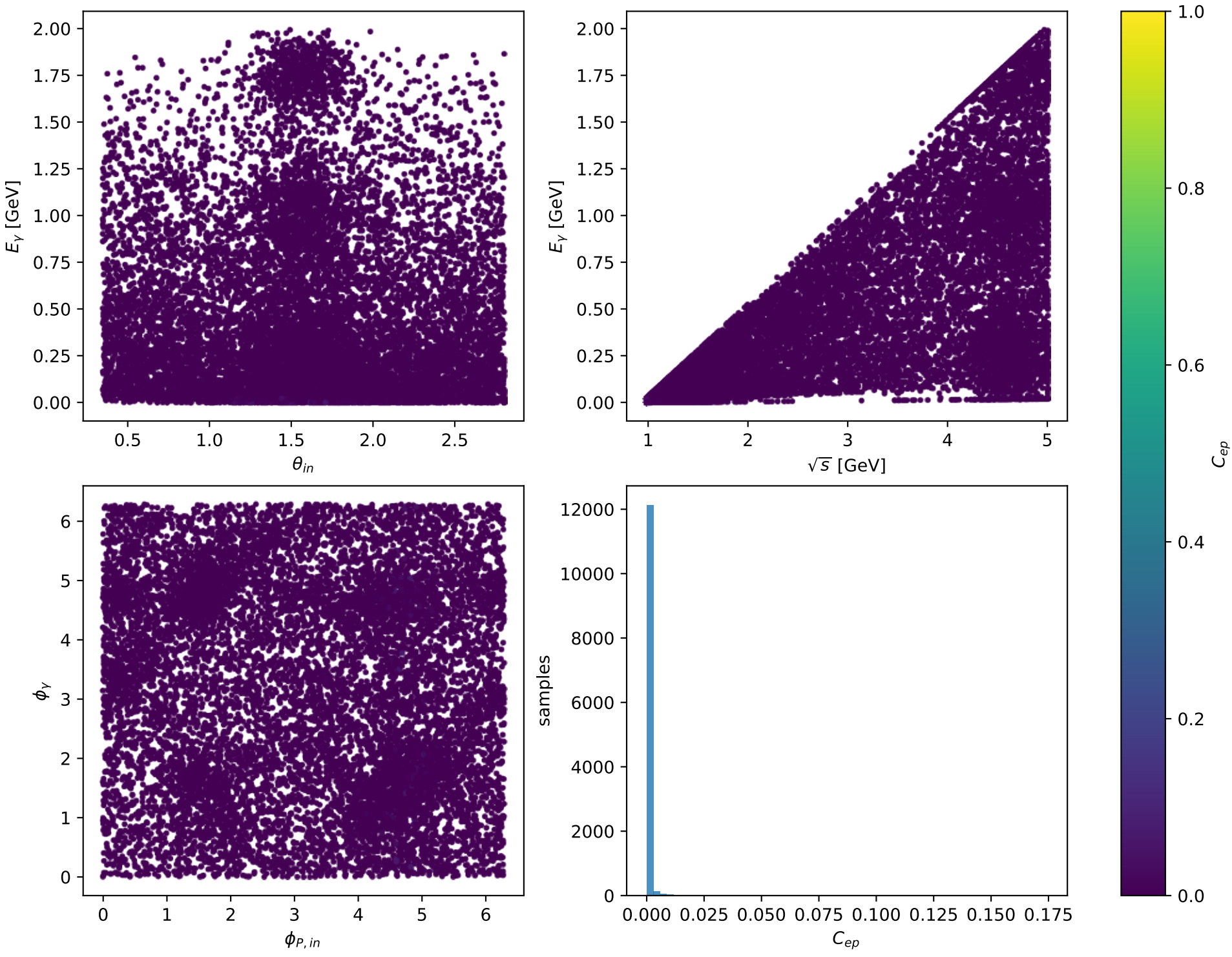
Phase-space scan: Ty proton [Ty_proton], max C_{ep}=0.1745
