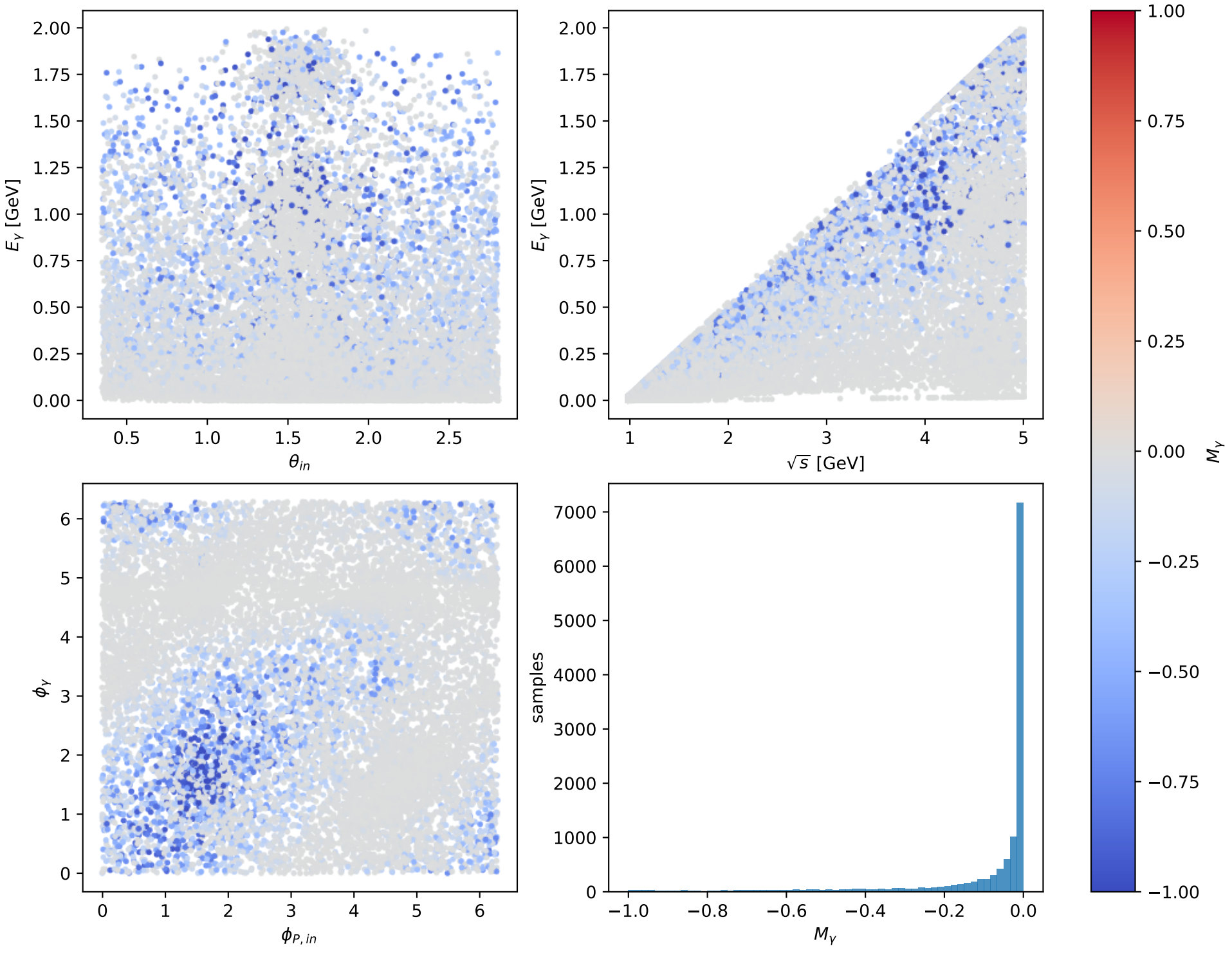
Phase-space scan: Ty proton [Ty_proton], max M_\gamma = -0
