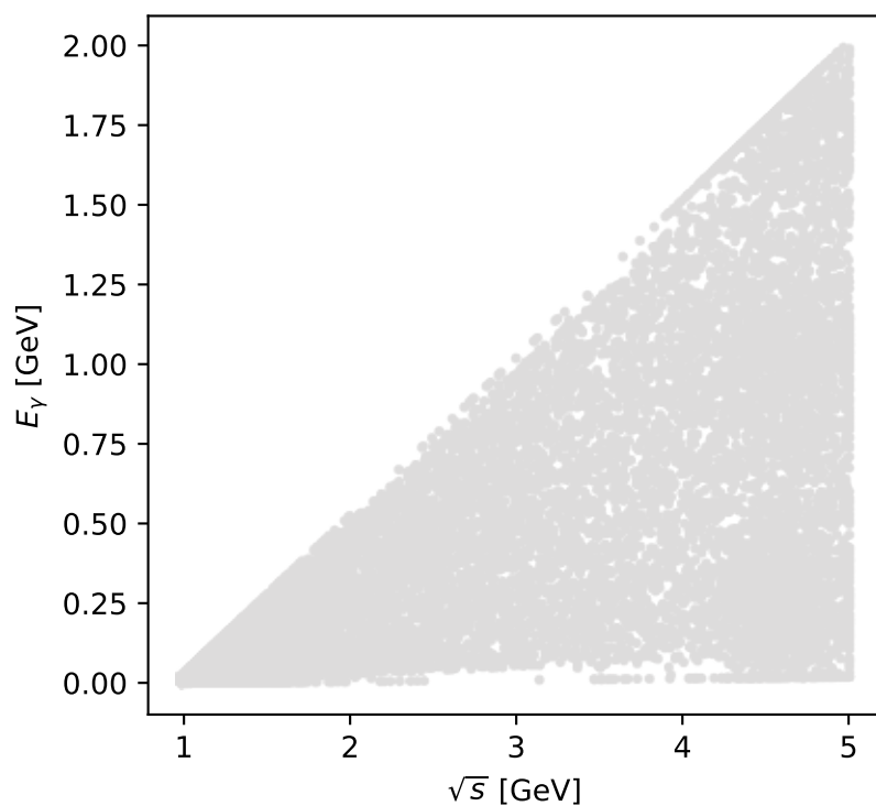
Phase-space scan: Unpolarized [unpolarized], max M_Y = -0
