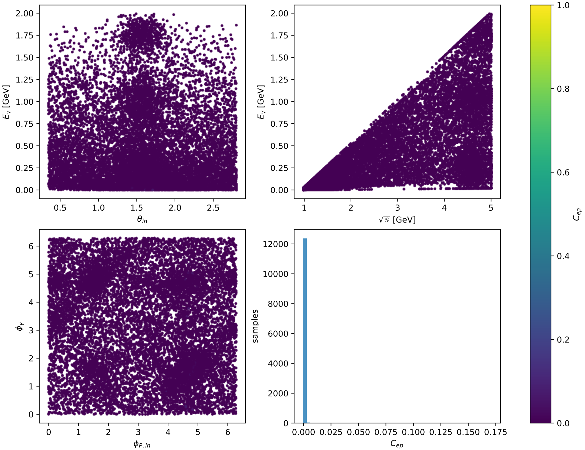
Phase-space scan: Unpolarized [unpolarized], max C_{ep}=0.17075
