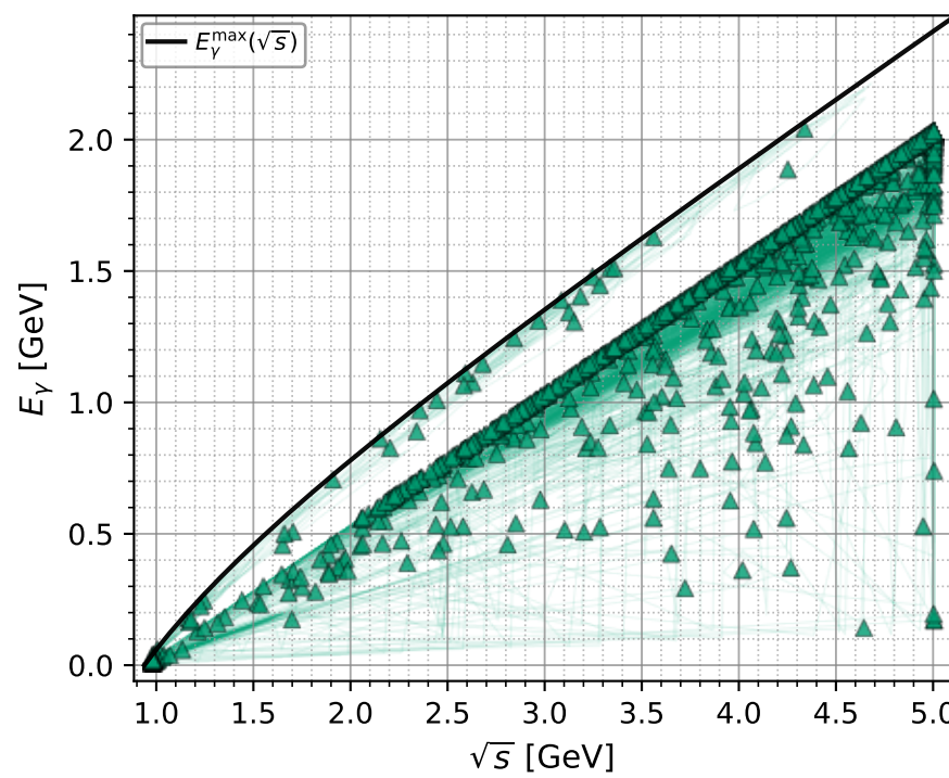
electron: full low-1 - C_{e\gamma} phase space with projected 8D contours
