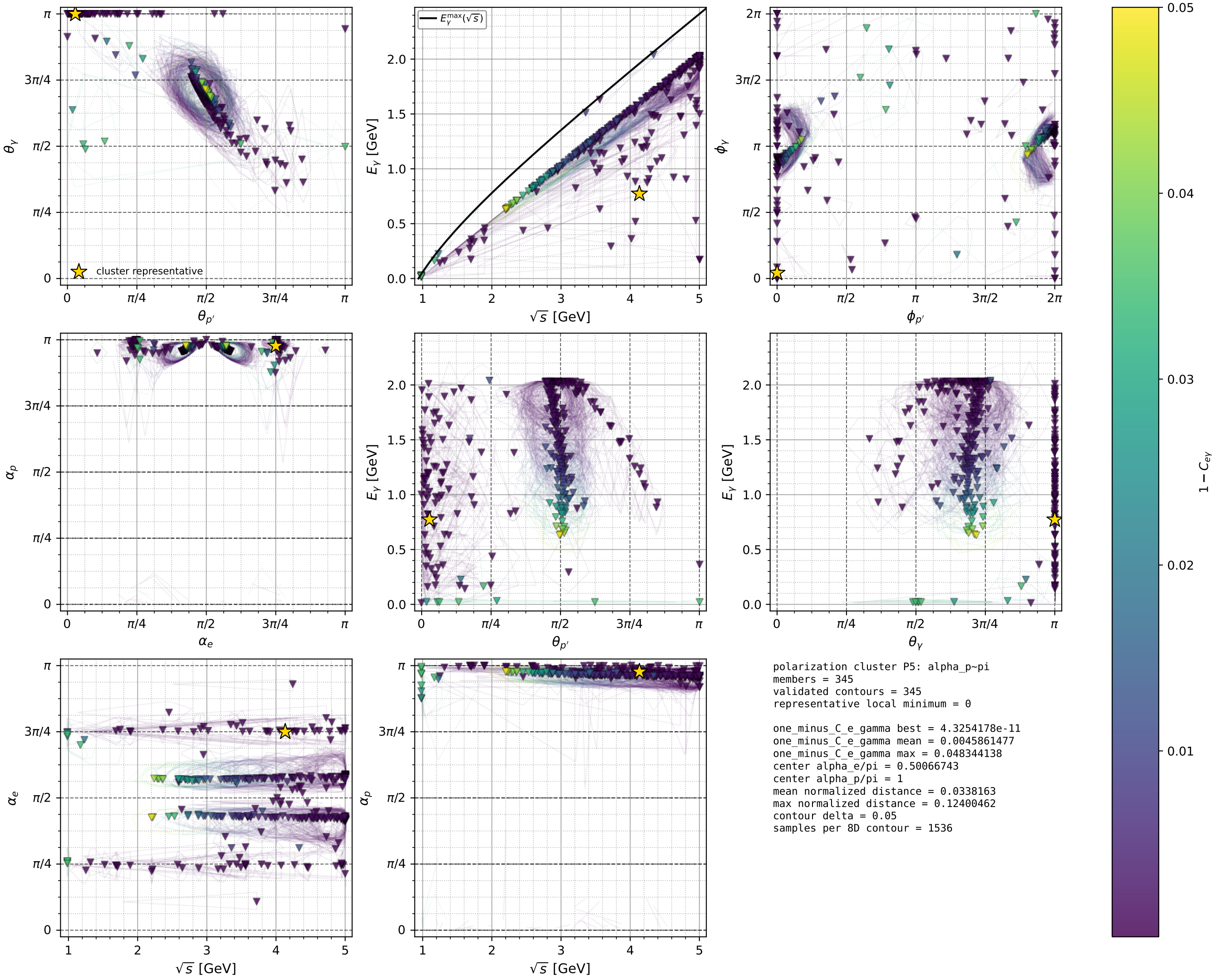
electron: polarization cluster P5 with projected 8D contours
