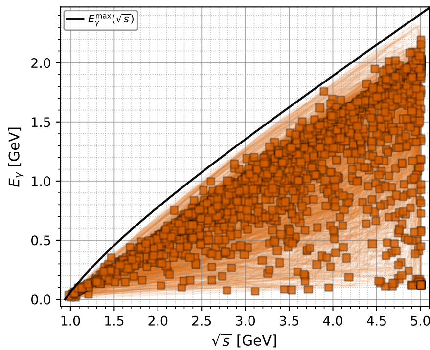
electron: full low-1 - C_{p\gamma} phase space with projected 8D contours
