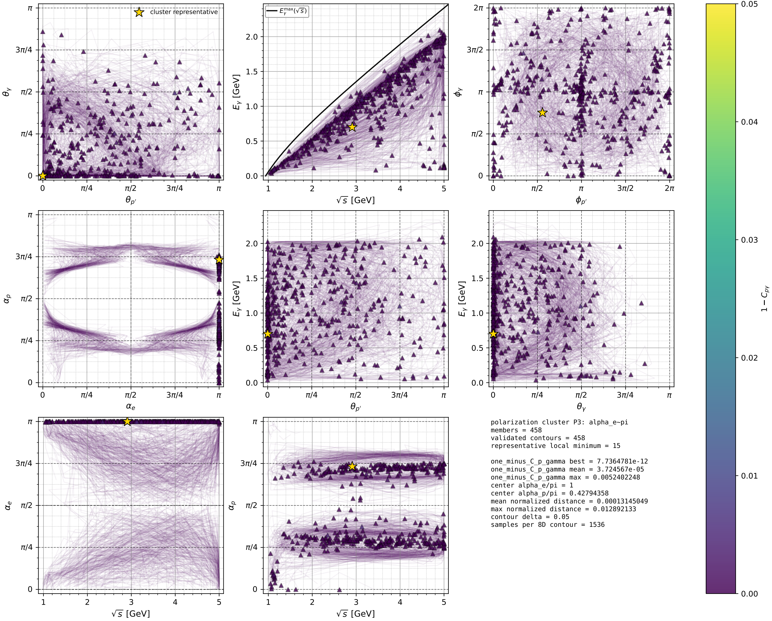
electron: polarization cluster P3 with projected 8D contours
