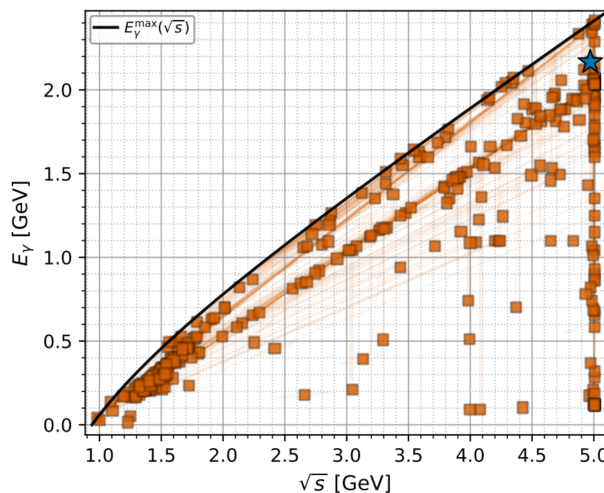
electron: full low- d_{\text{GHZ}} phase space with projected 8D contours
