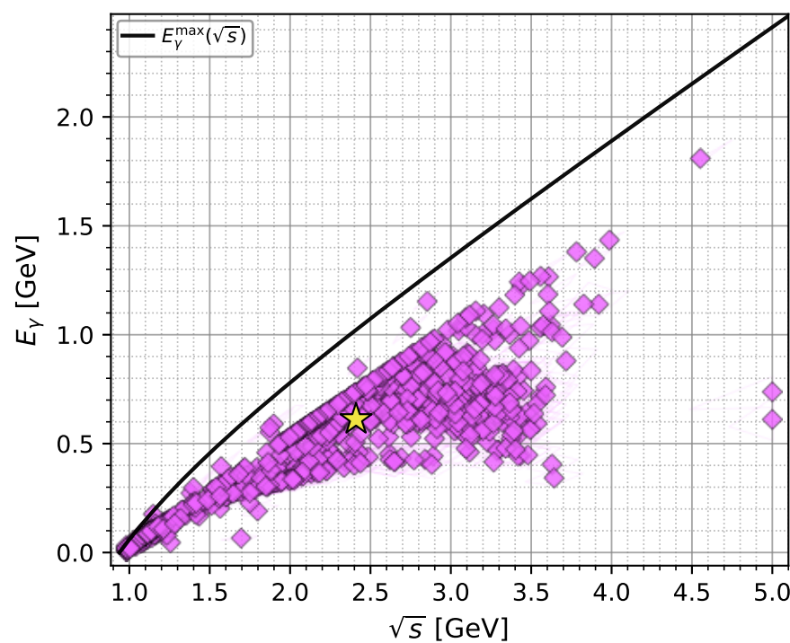
electron: full low- D_W phase space with projected 8D contours
