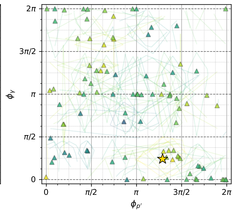
electron: polarization cluster P3 with projected 8D contours
