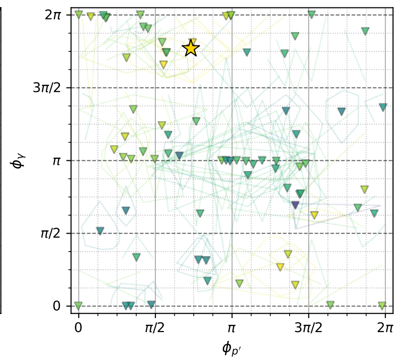
electron: polarization cluster P5 with projected 8D contours
