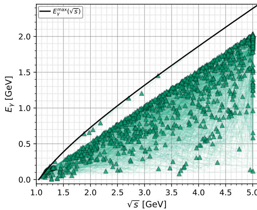
muon: full low-1 - C_{e\gamma} phase space with projected 8D contours
