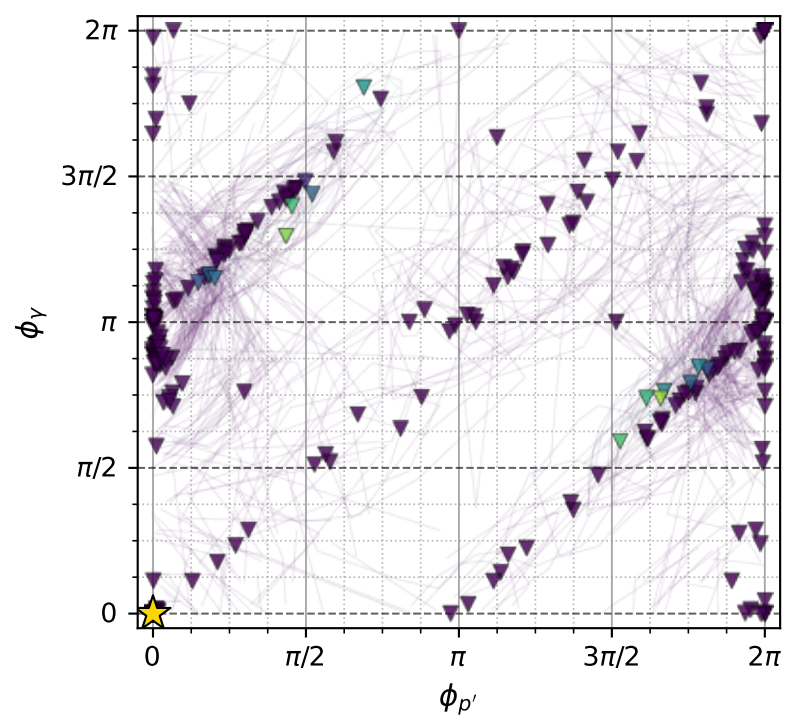
muon: polarization cluster P5 with projected 8D contours
