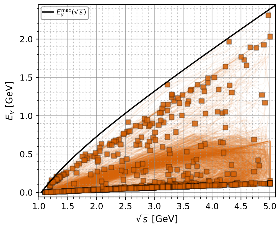
muon: full low-1 - C_{ep} phase space with projected 8D contours
