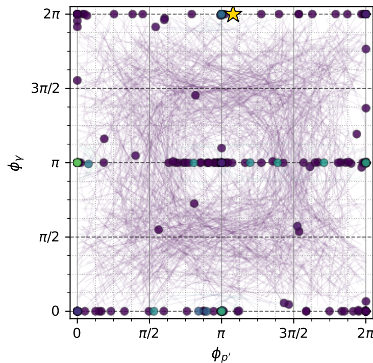
muon: polarization cluster P1 with projected 8D contours
