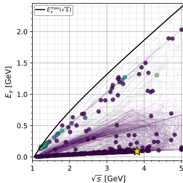
muon: polarization cluster P1 with projected 8D contours
