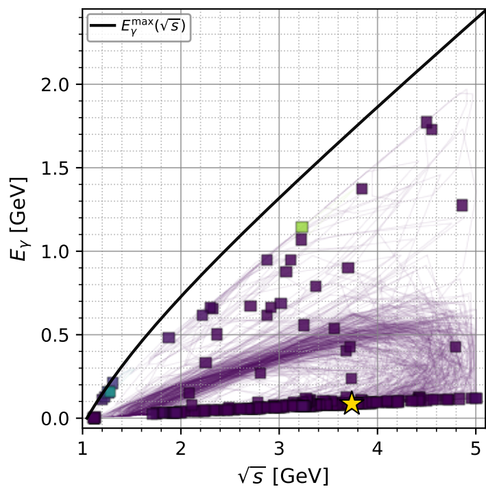
muon: polarization cluster P2 with projected 8D contours
