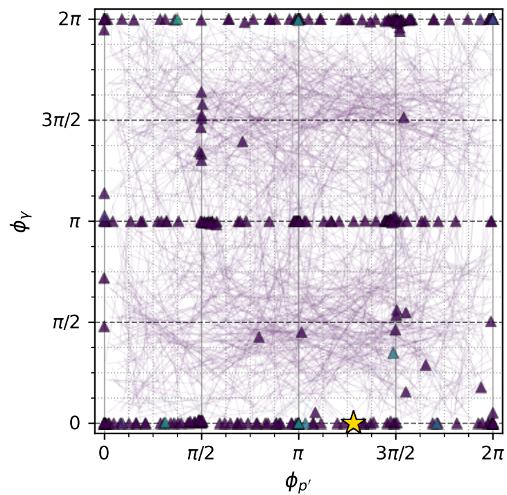
muon: polarization cluster P3 with projected 8D contours
