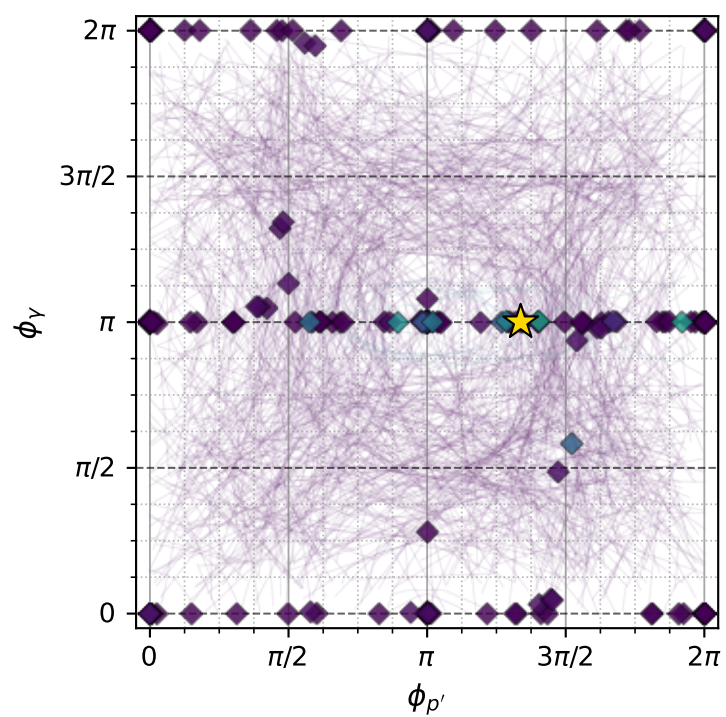
muon: polarization cluster P4 with projected 8D contours
