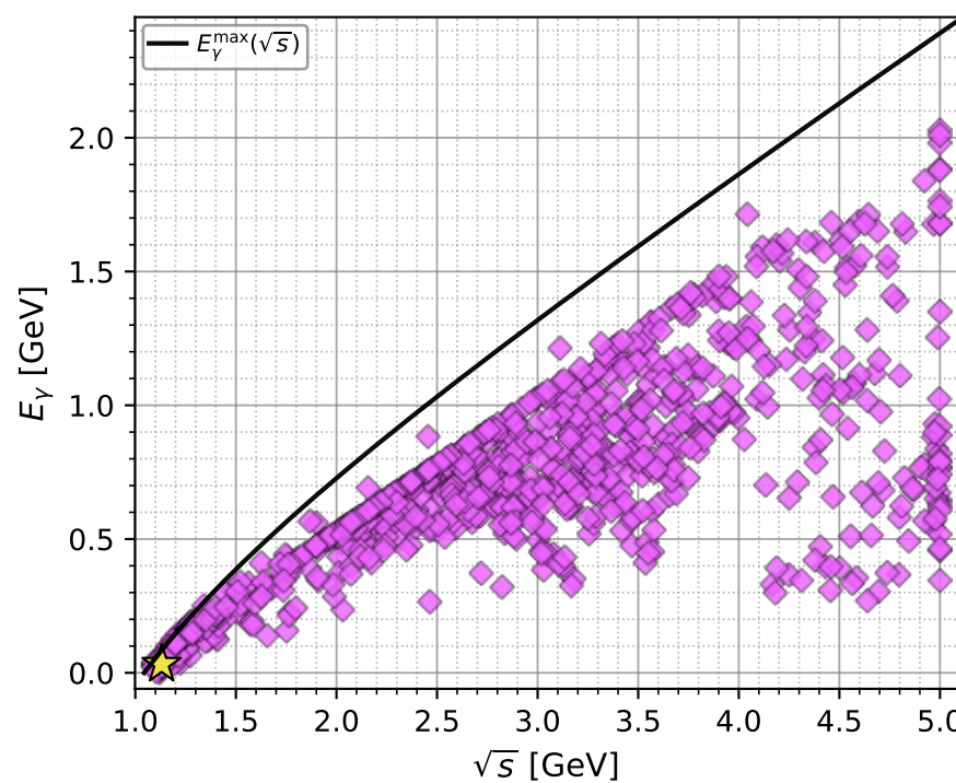
muon: full low- D_W phase space (contours omitted)
