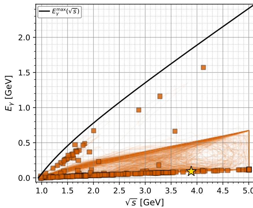
electron: full low-1 - C_{ep} phase space with projected 8D contours
