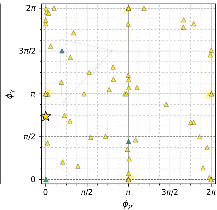
electron: polarization cluster P3 with projected 8D contours
