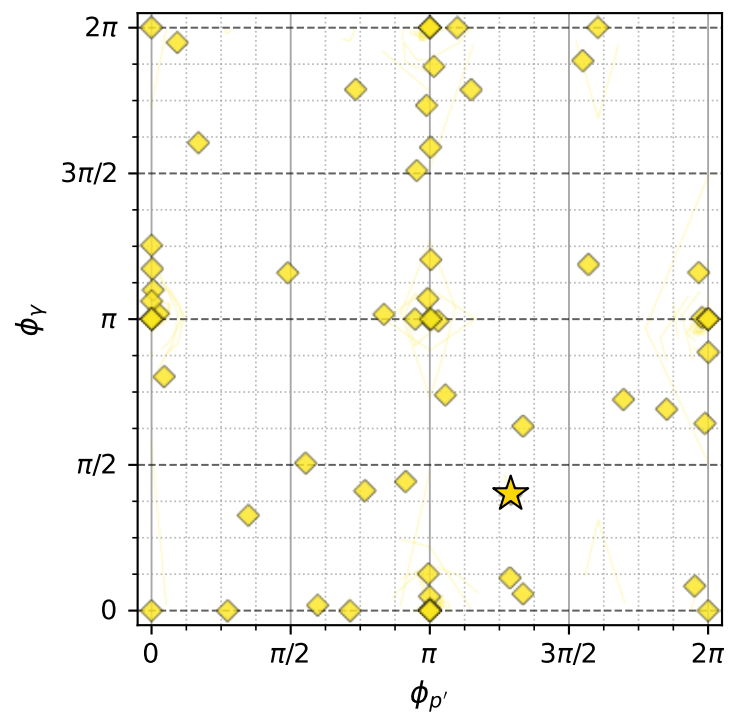
electron: polarization cluster P4 with projected 8D contours
