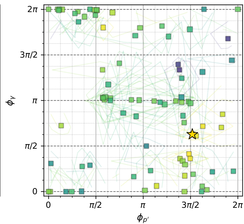
electron: polarization cluster P2 with projected 8D contours
