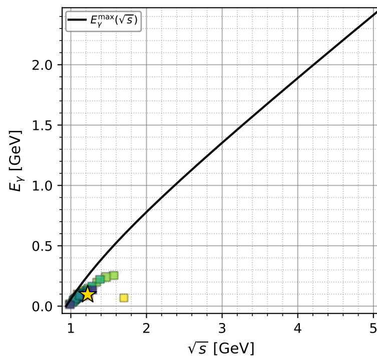
electron: polarization cluster P2 with projected 8D contours
