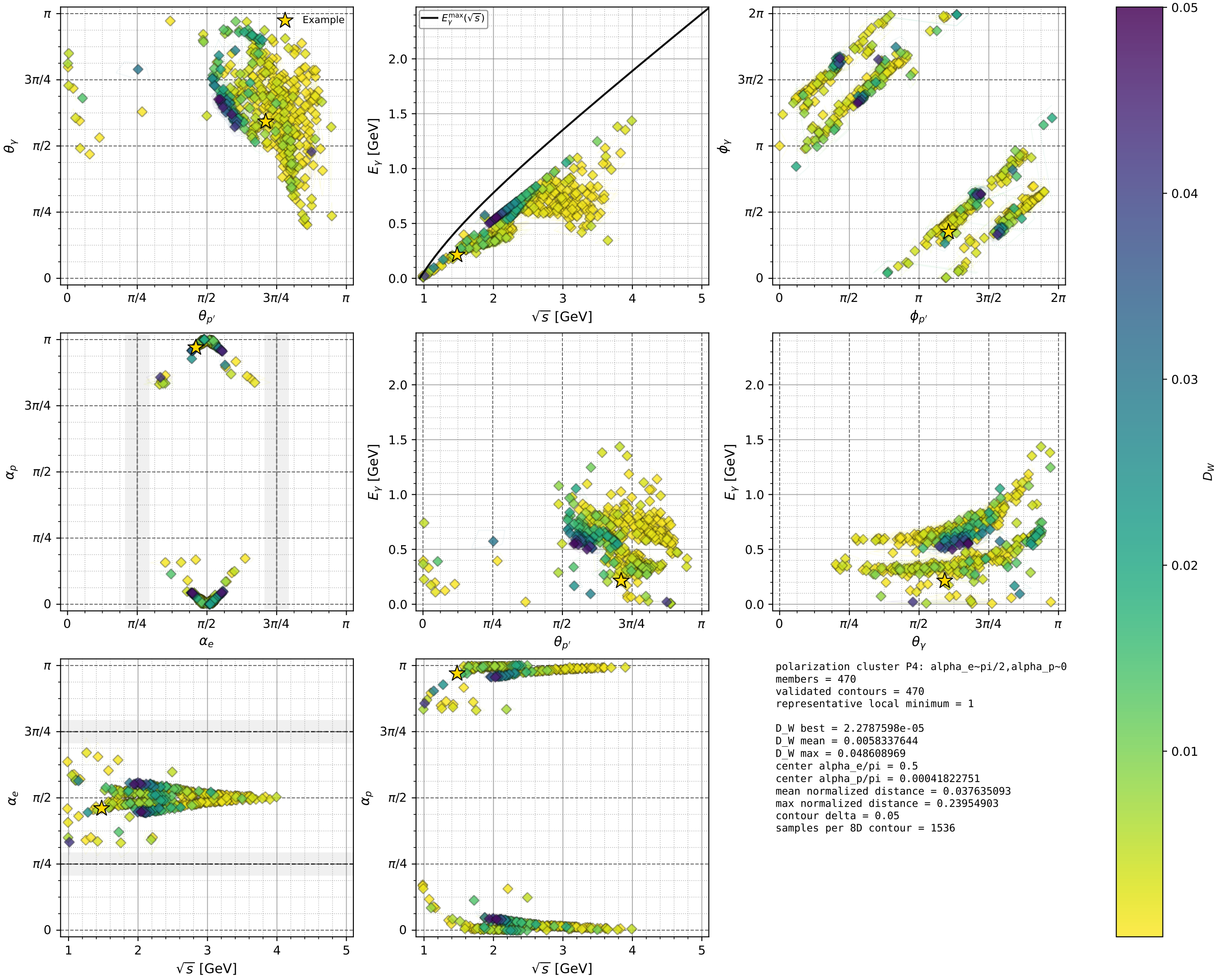
electron: polarization cluster P4 with projected 8D contours
