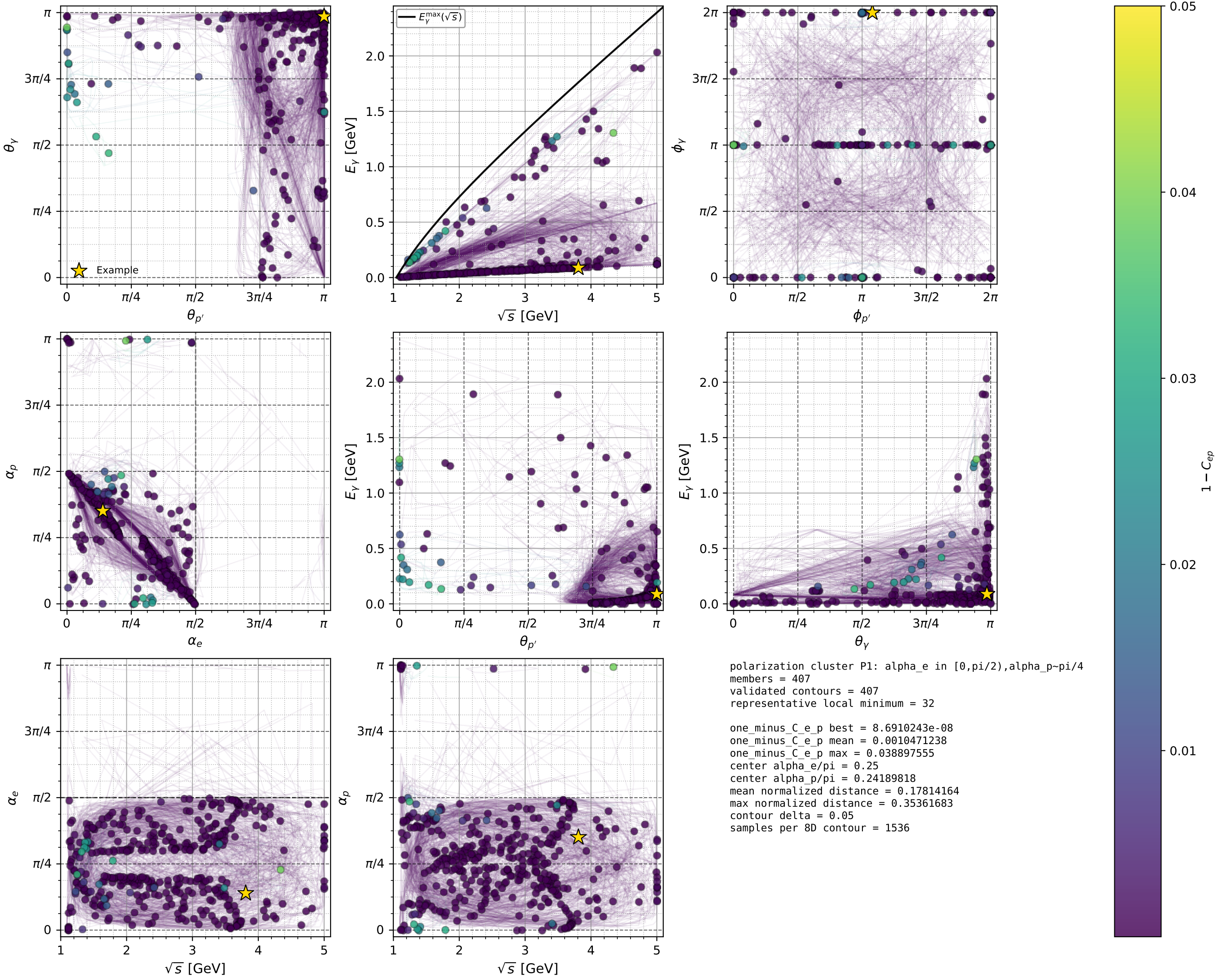
muon: polarization cluster P1 with projected 8D contours
