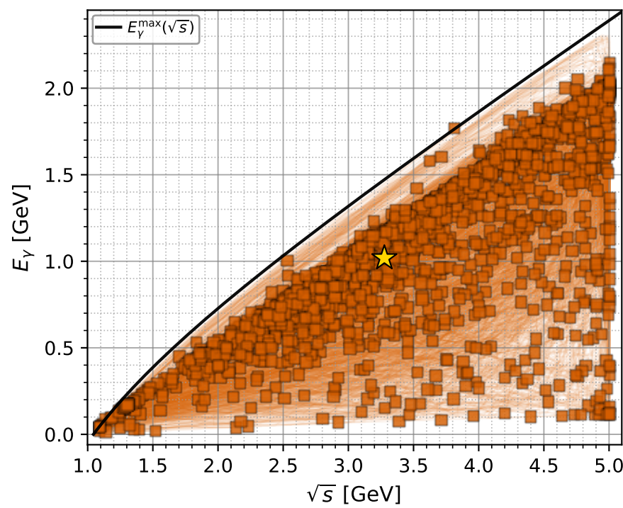
muon: full low-1 – C_{p\gamma} phase space with projected 8D contours
