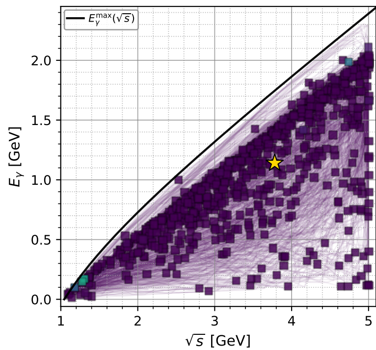
muon: polarization cluster P2 with projected 8D contours
