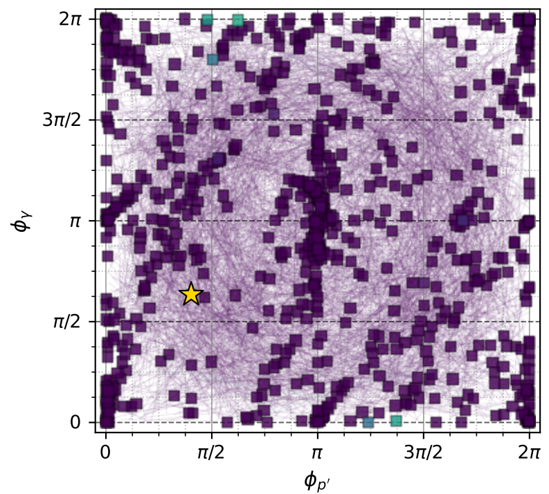
muon: polarization cluster P2 with projected 8D contours
