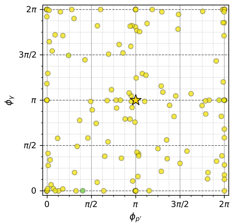
muon: polarization cluster P1 (contours omitted)
