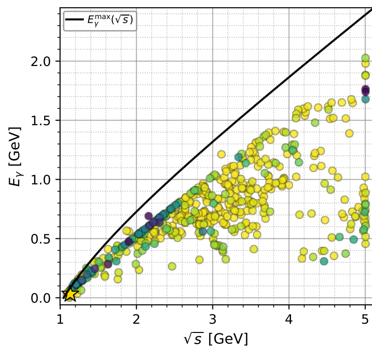
muon: polarization cluster P1 (contours omitted)
