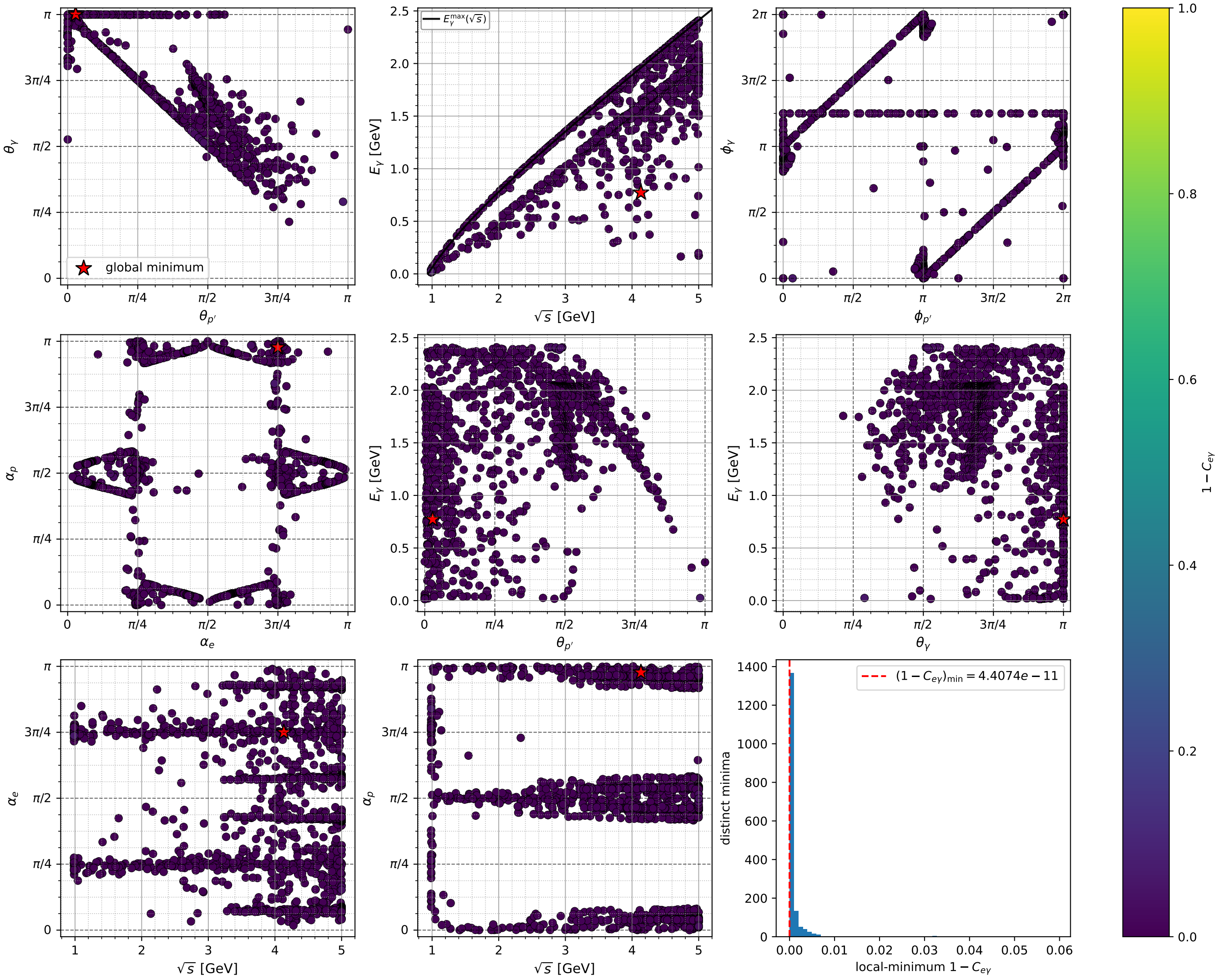
electron: all 1653 distinct gradient-search local minima of 1 - C_{e\gamma}
