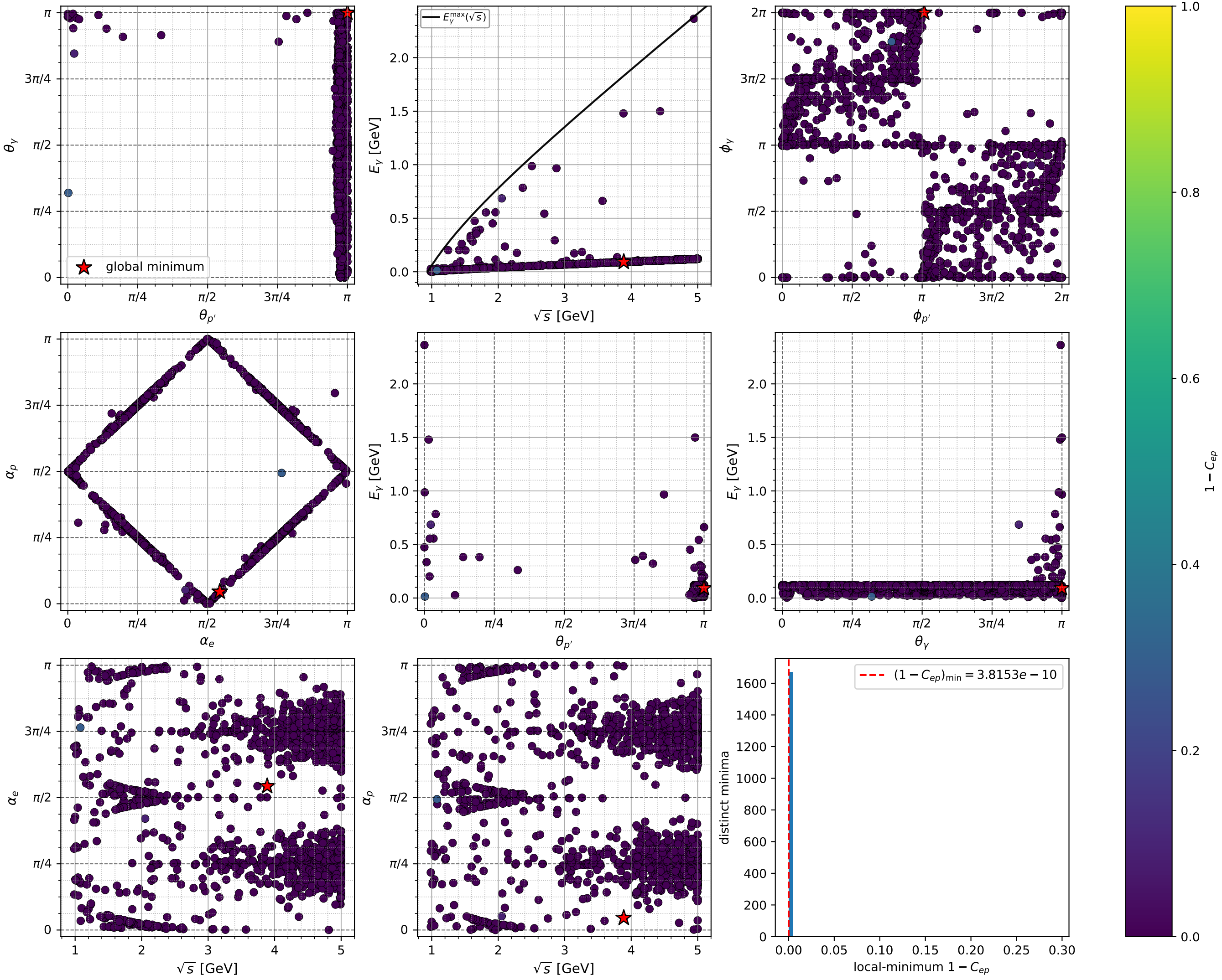
electron: all 1677 distinct gradient-search local minima of 1 - C_{ep}
