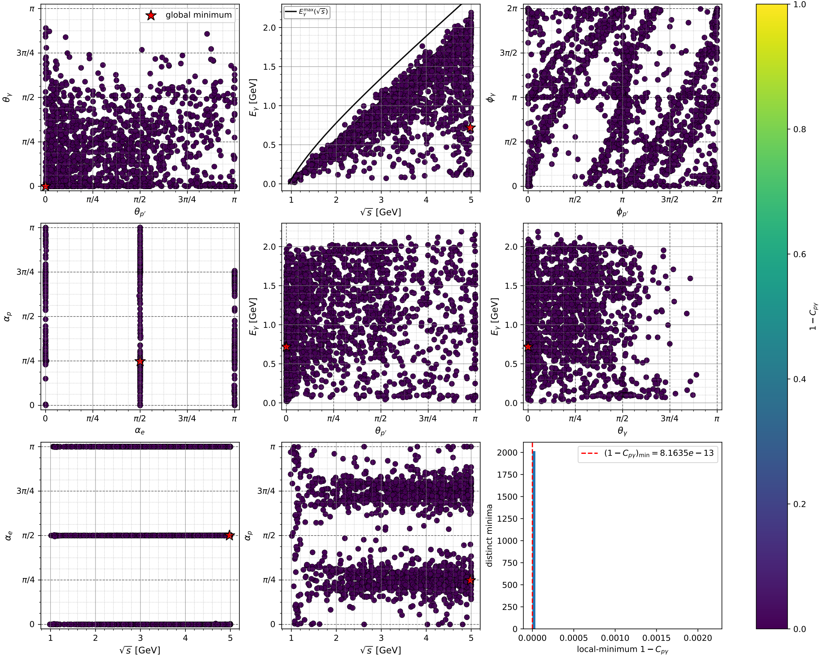
electron: all 2019 distinct gradient-search local minima of 1 - C_{p\gamma}
