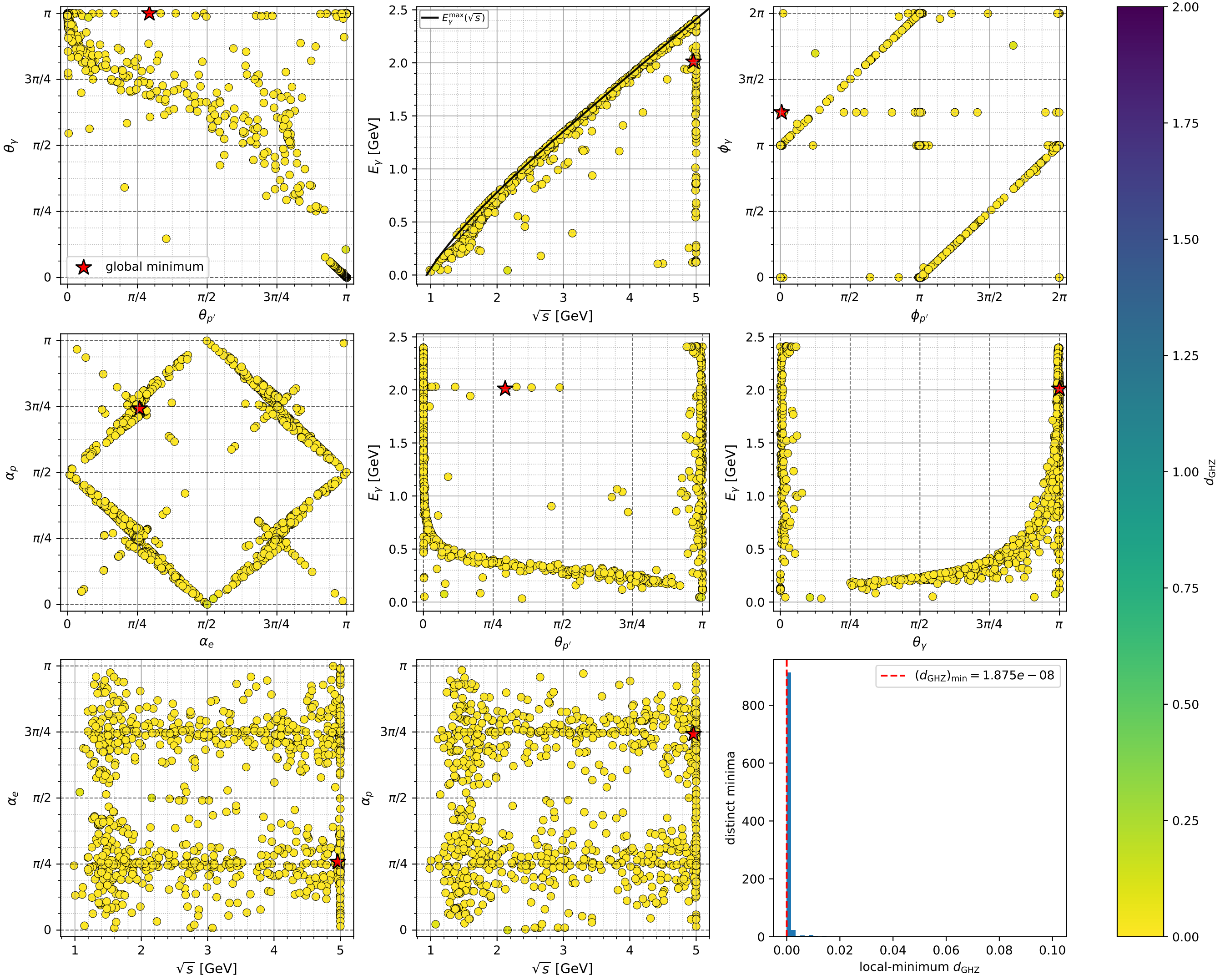
electron: all 960 distinct gradient-search local minima of d_{\text{GHZ}}
